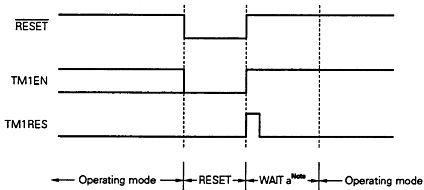
Fig. 19-2 Resetting
