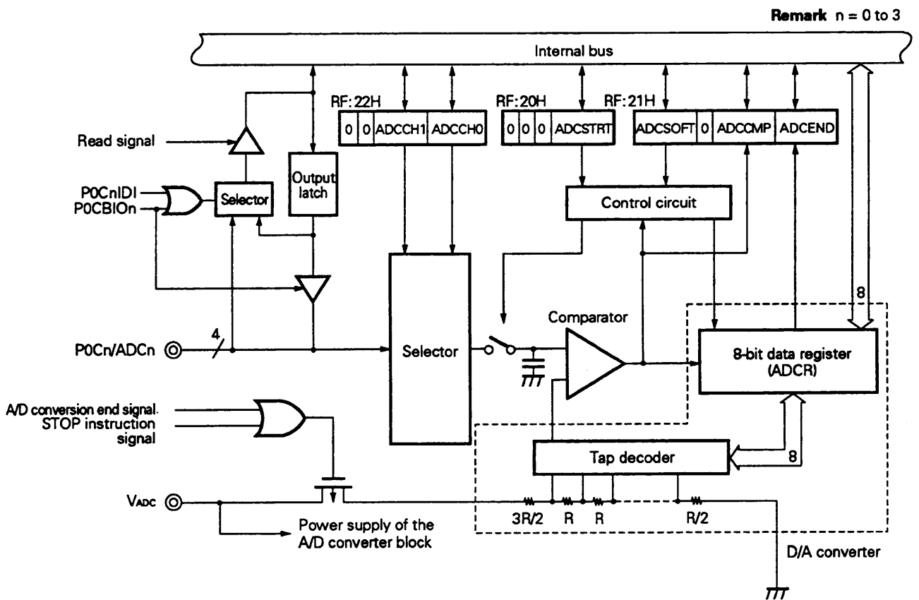
Fig. 14-1 Block Diagram for the A/D Converter
