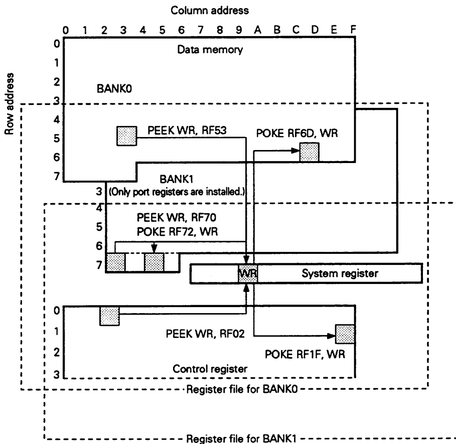
Fig. 8-1 Register File Configuration and Accessing the Register File Using the PEEK and POKE Instructions
