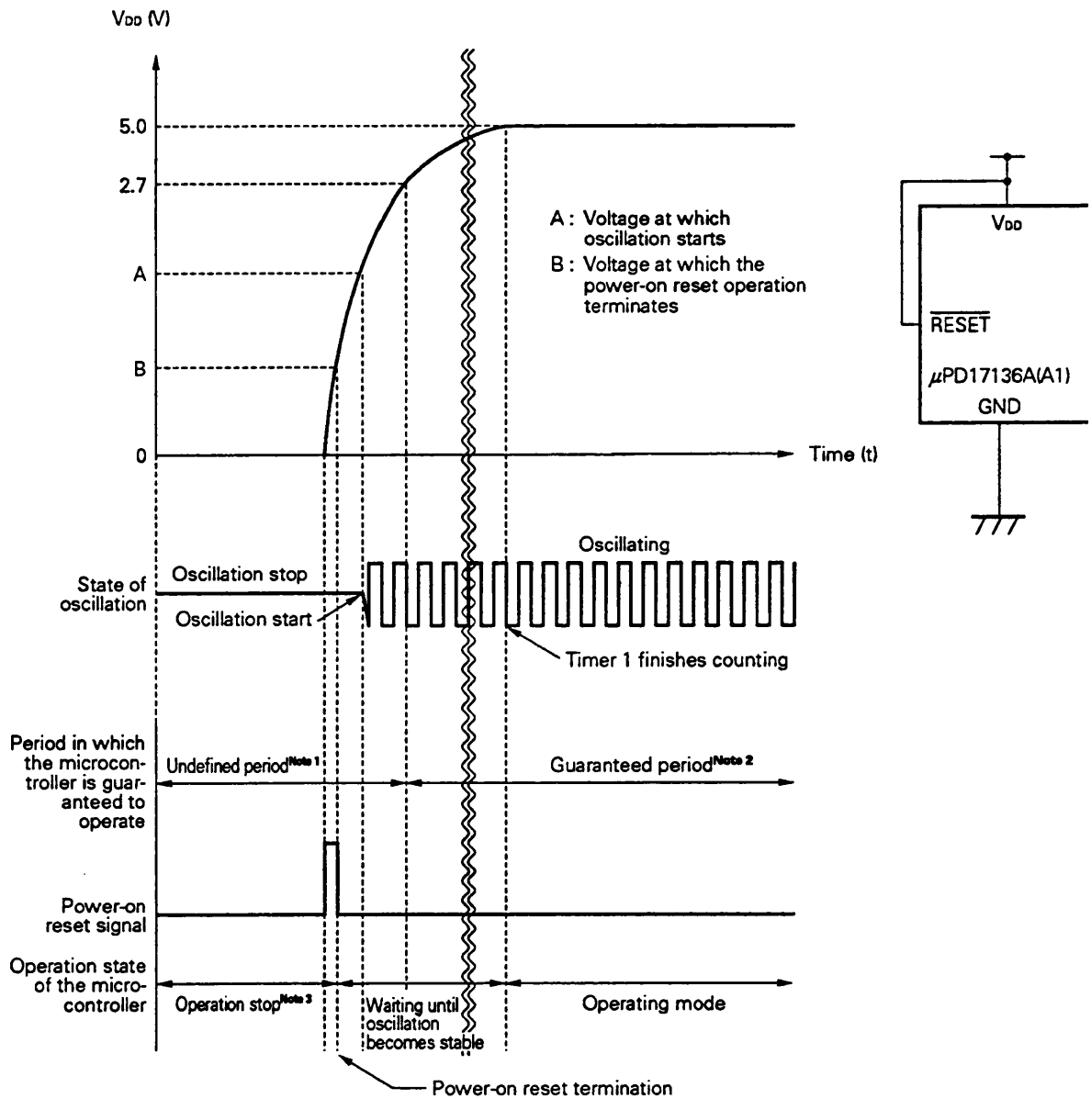
Fig. 19-3 Example of the Power-On Reset Operation
