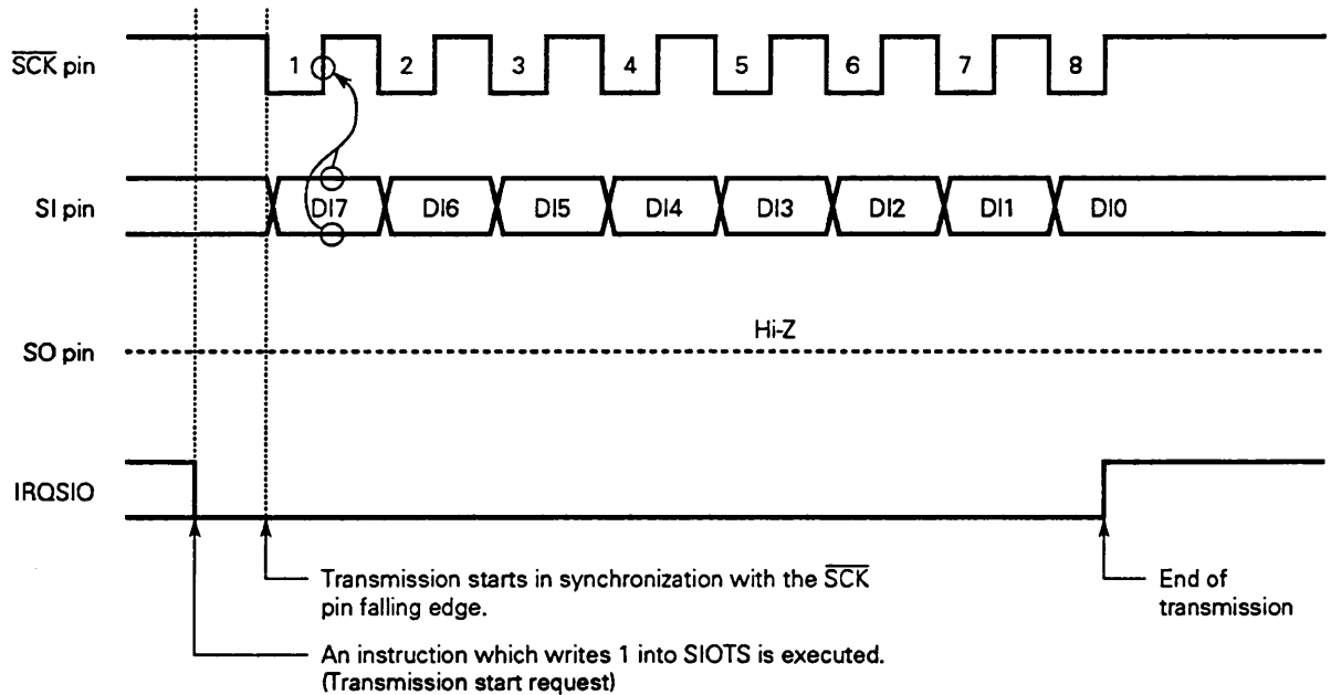
Fig. 15-3 Timing of 8-Bit Reception Mode
