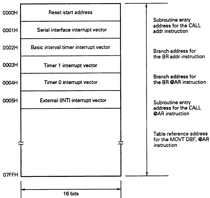
Fig. 2-1 Program Memory Map
