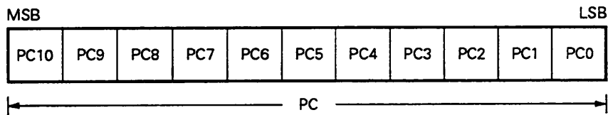
Fig. 3-1 Program Counter
