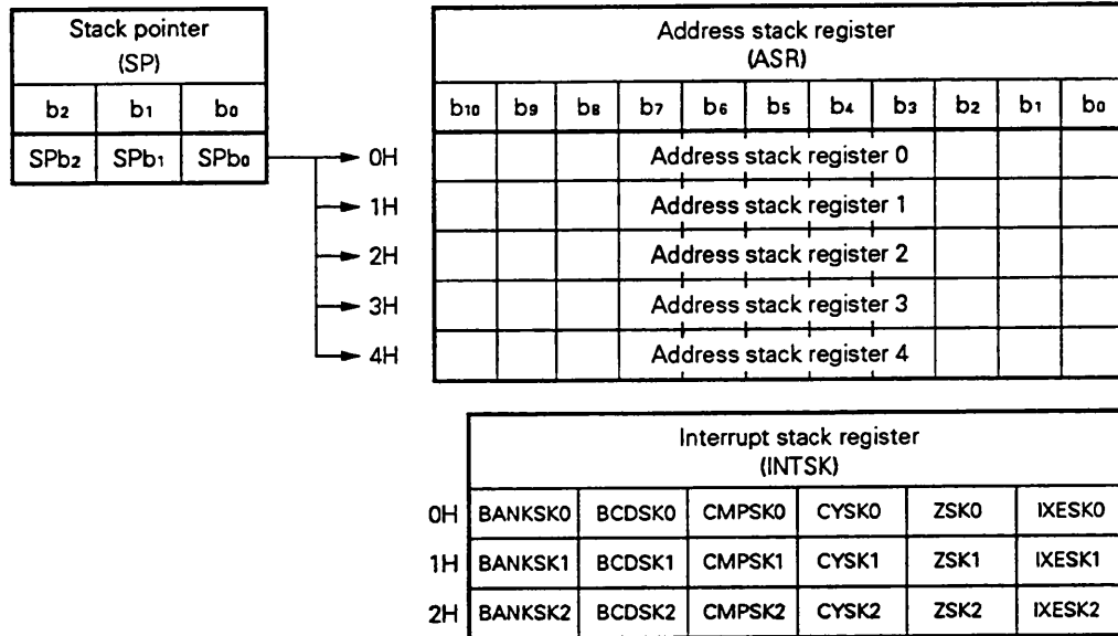
Fig. 4-1 Stack Configuration
