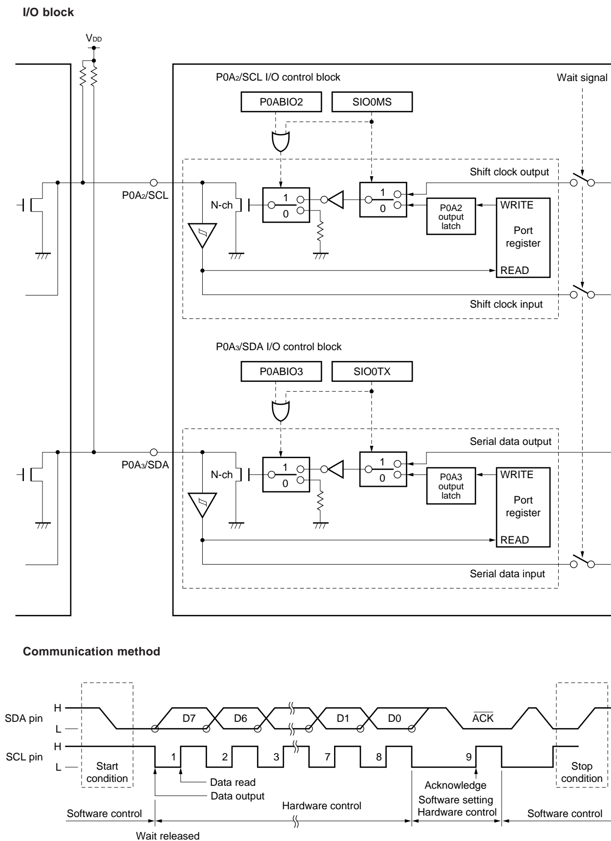
Figure 19-14. I/O Block and Communication Method in I 2 C Bus Mode
