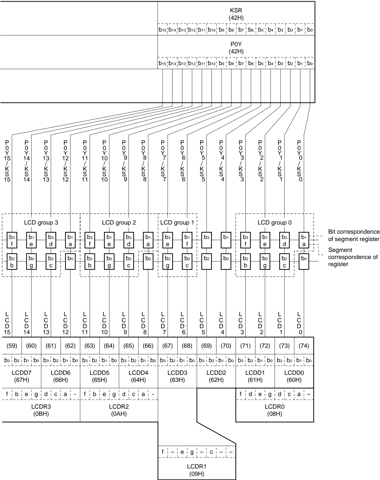
Figure 21-7. Relation among LCD Display Dot, Ports 0E Through 0Y, Key Source Output, and Data Setting Registers (2/2)
