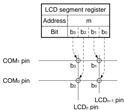
Figure 21-5. Relation between 1 Nibble of LCD Segment Register and LCD Display Dot
