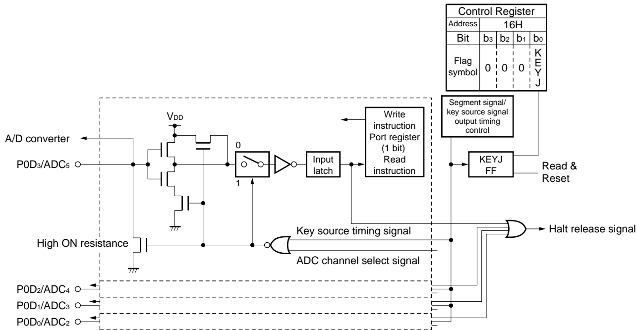
Figure 22-6. Configuration of Key Input Control Block
