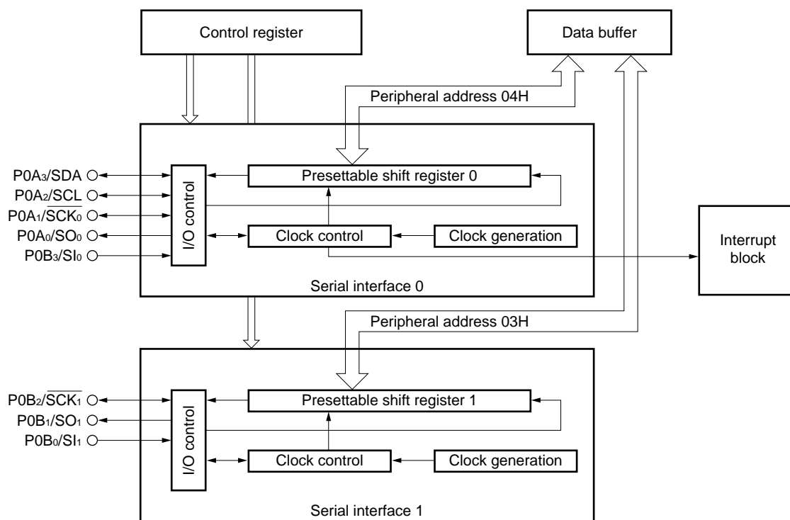
Figure 19-1. Block Diagram of Serial Interface
