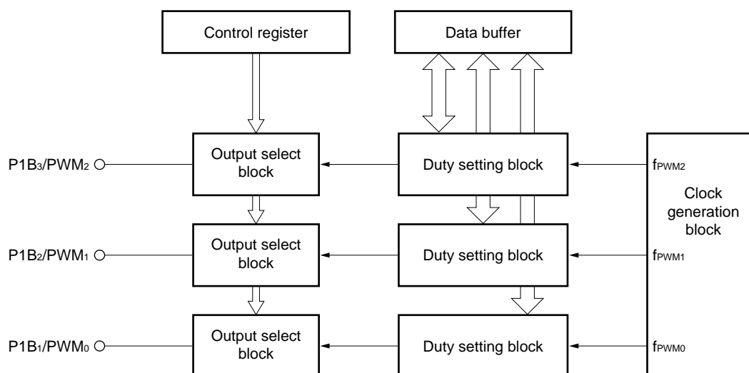
Figure 17-1. Block Diagram of D/A Converter
