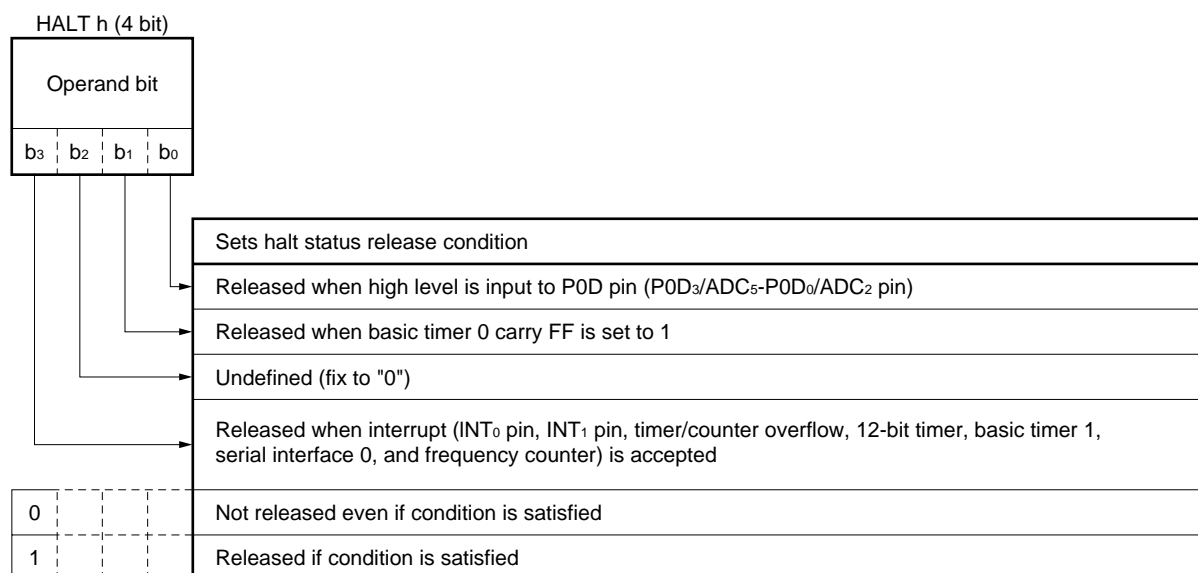
Figure 12-3. Halt Release Condition
