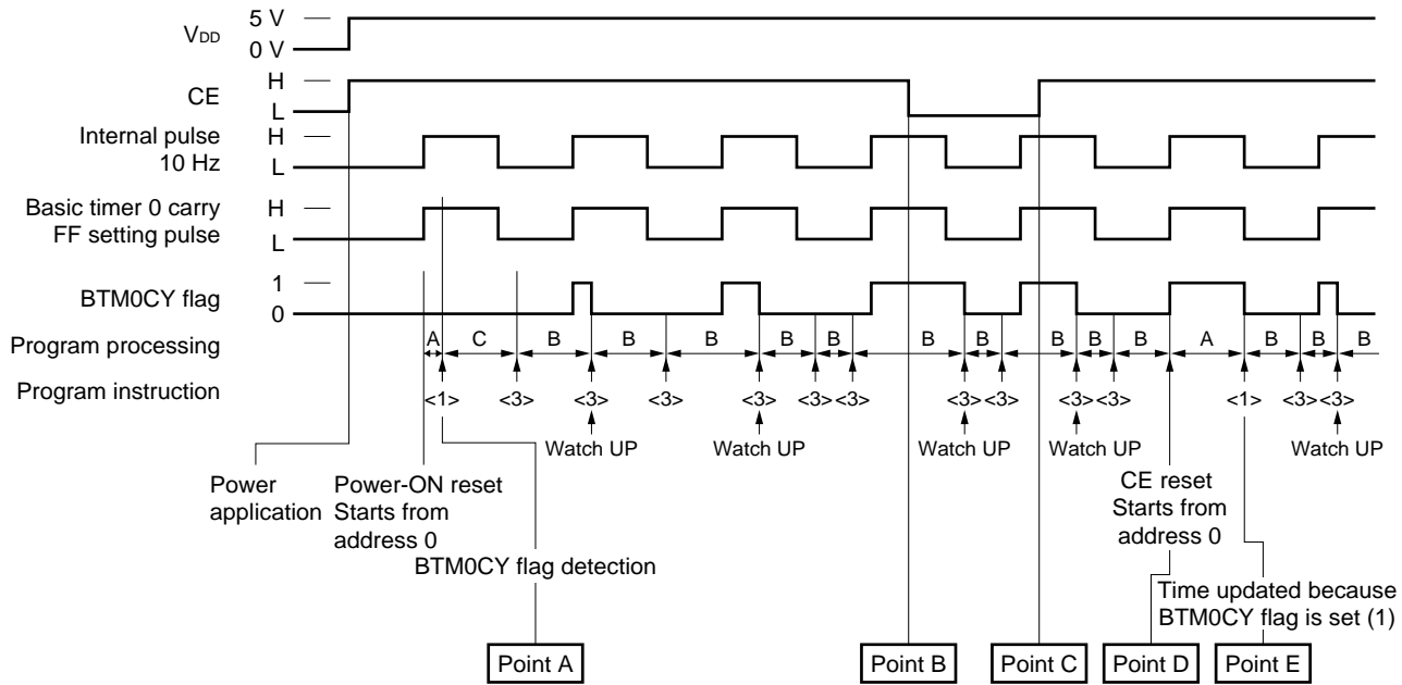
Figure 11-7. Timing Chart
