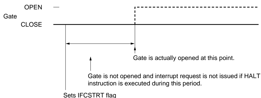
Figure 20-5. Gate Operation When “HALT” Instruction Is Used
