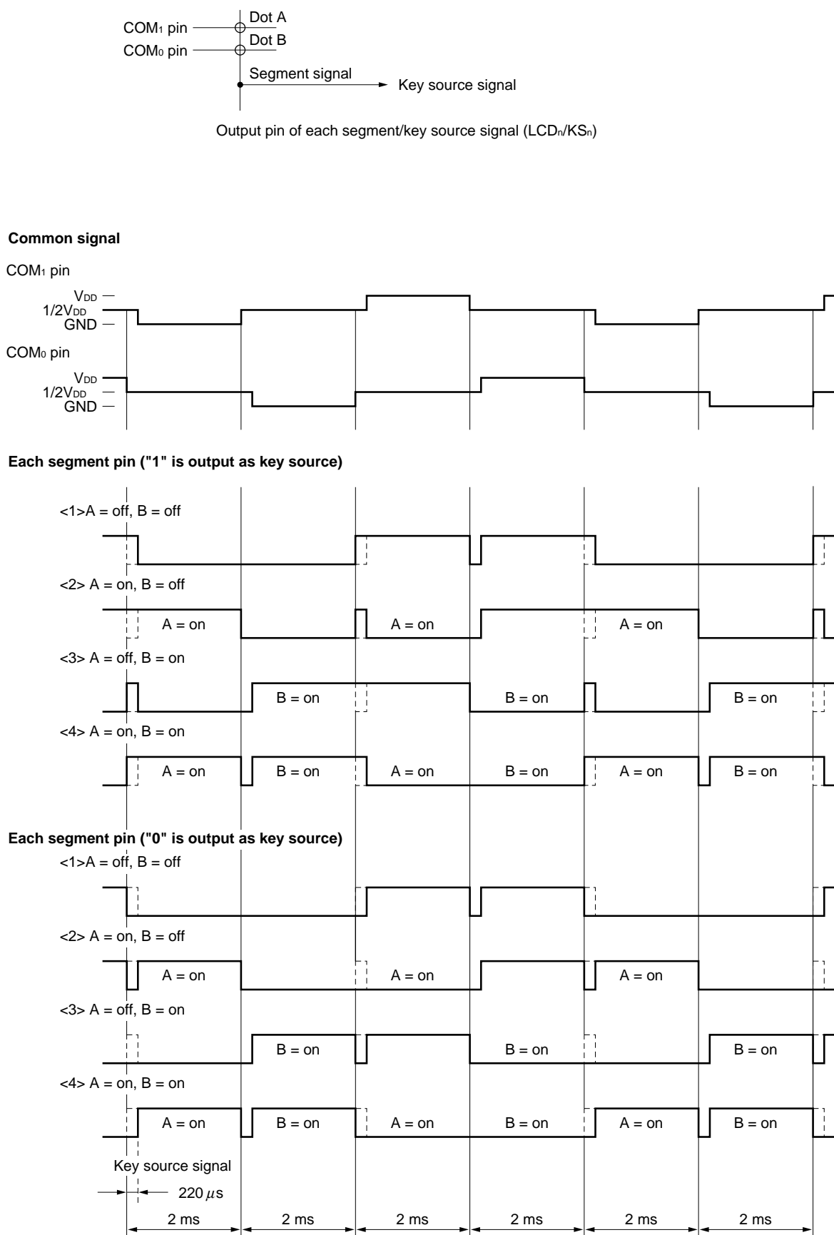
Figure 22-5. Output Waveforms of Key Source and Segment Signals
