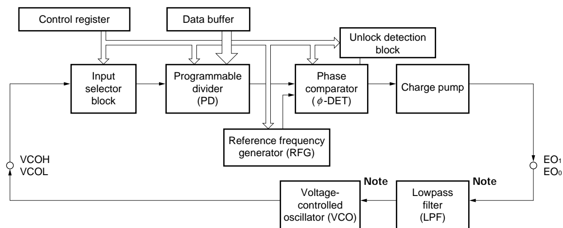
Figure 14-1. Block Diagram of PLL Frequency Synthesizer
