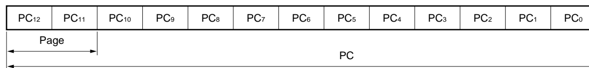
Figure 2-3. Program Counter Configuration
