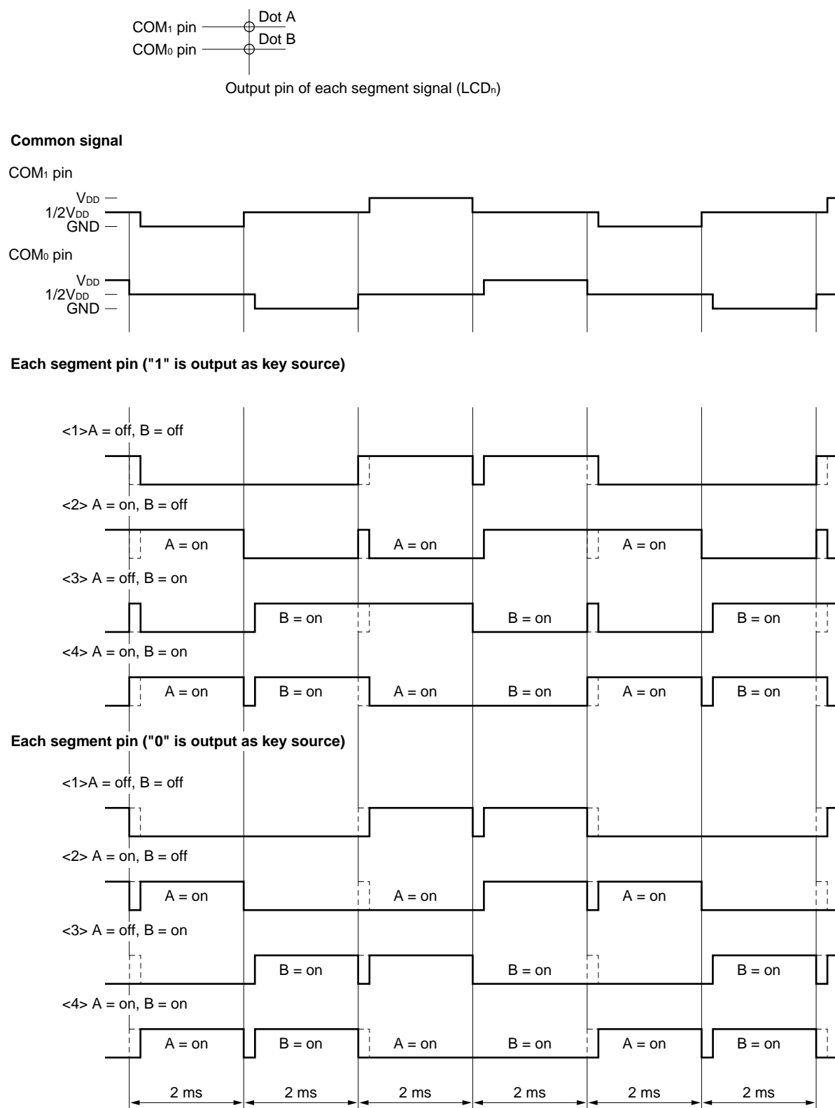
Figure 21-10. Output Waveforms of Common and Segment Signals (when key source signals are output)
