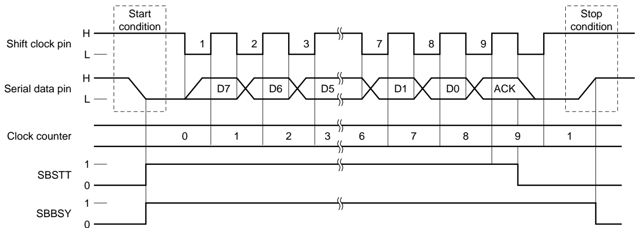
Figure 19-5. Operations of SBSTT and SBBSY Flags
