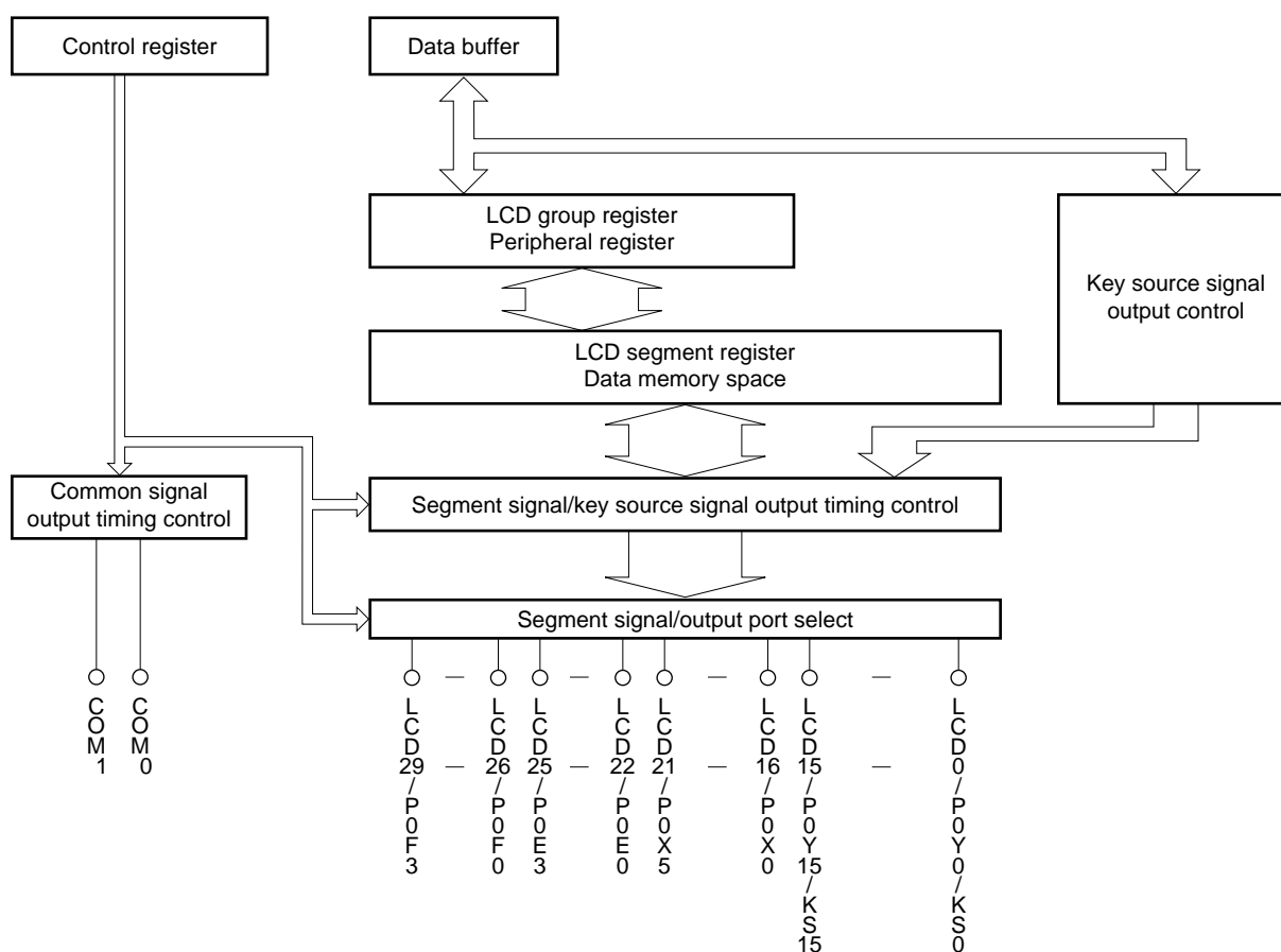
Figure 21-1. Block Diagram of LCD Controller/Driver
