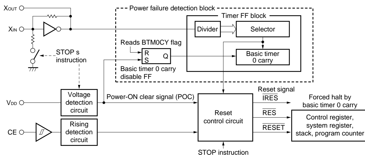
Figure 13-1. Configuration of Reset Block
