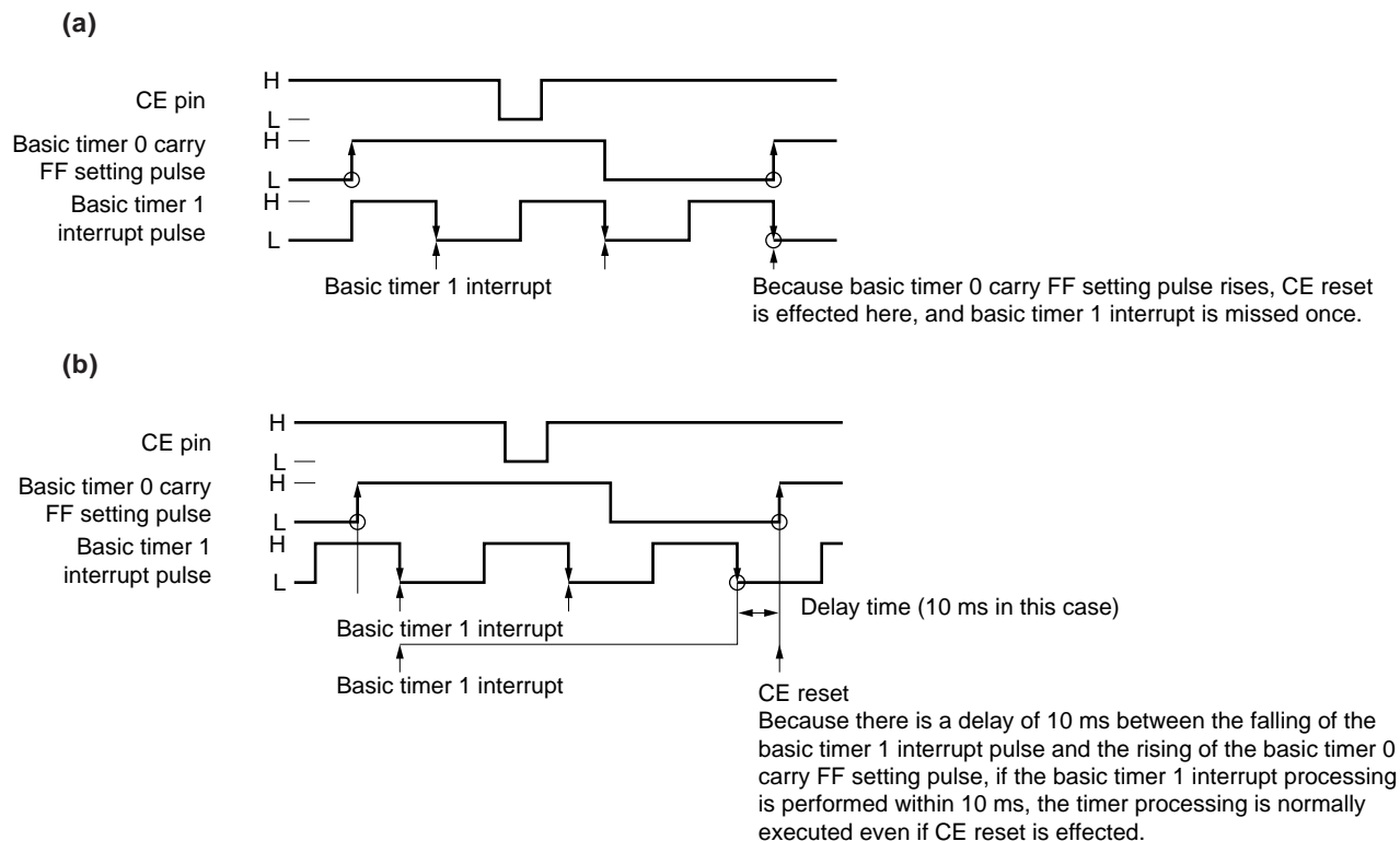
Figure 11-12. Timing Chart
