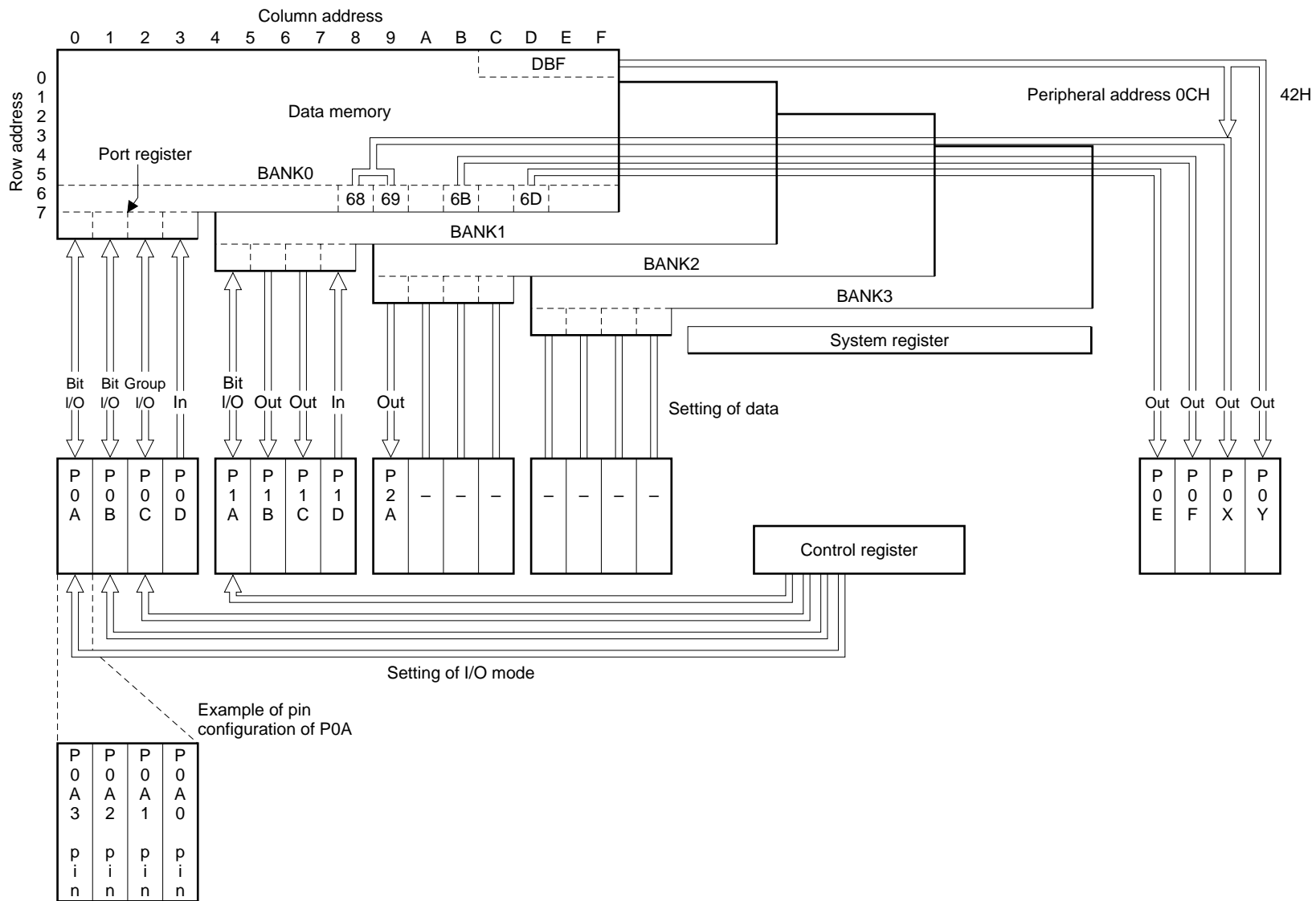
Figure 15-1. Block Diagram of General-Purpose Ports
