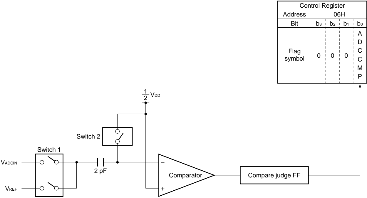
Figure 16-4. Configuration of Compare Block
