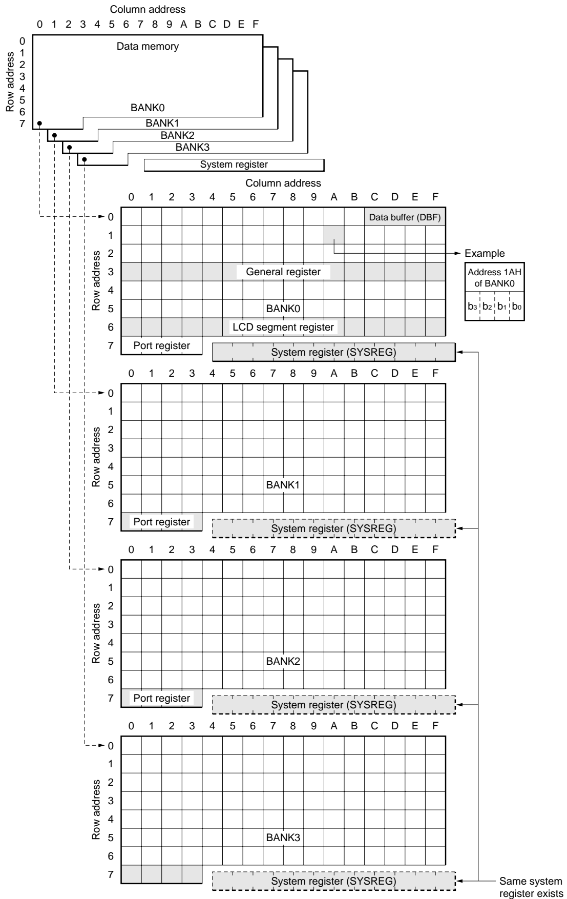
Figure 4-2. Data Memory Configuration
