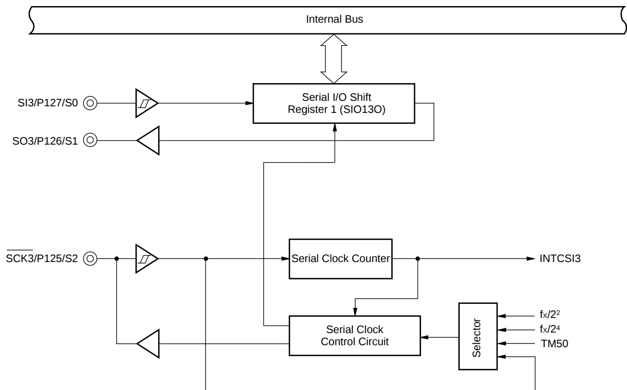
Figure 5-14: Serial Interface Channel 30 Block Diagram
