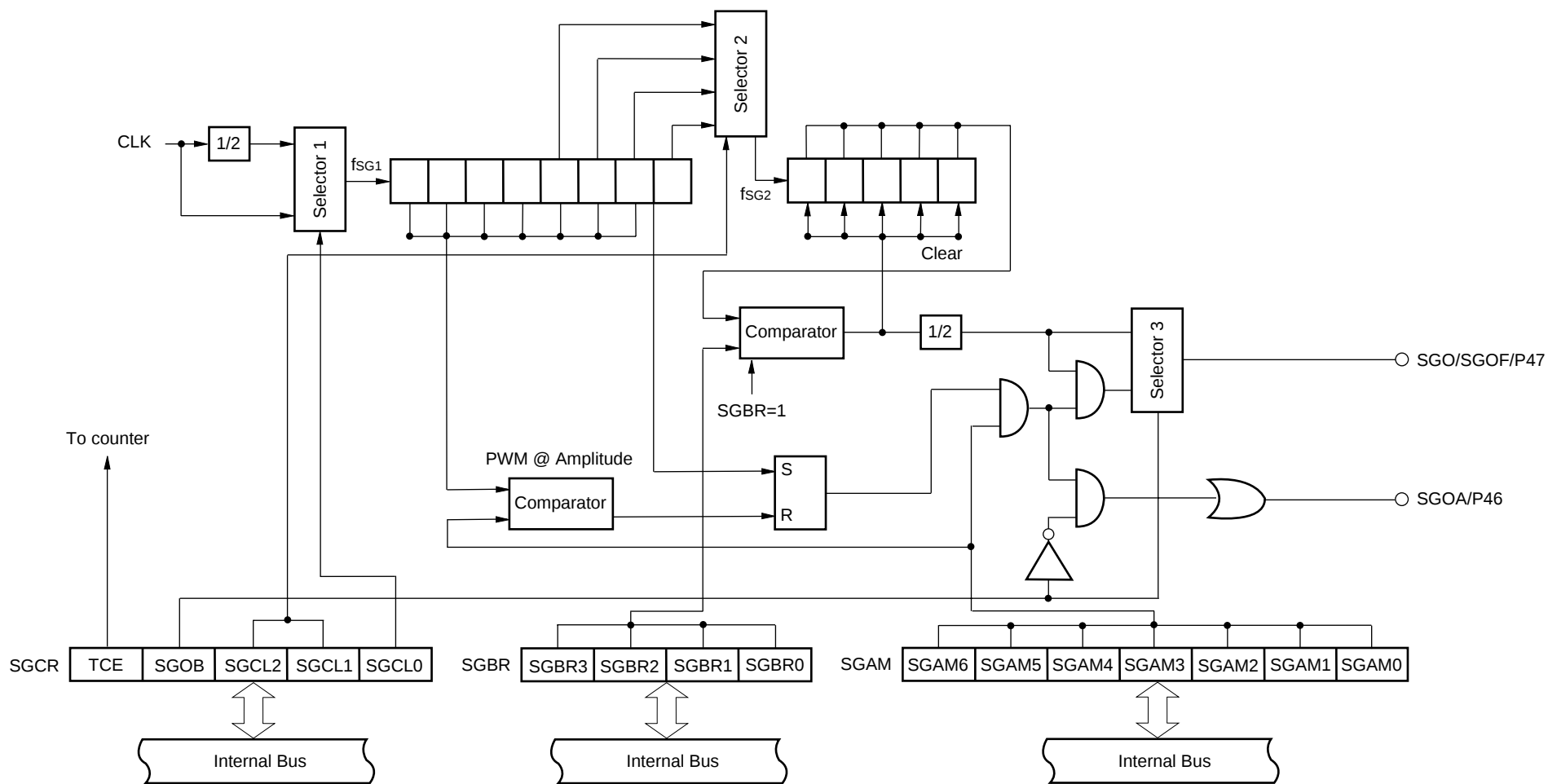
Figure 5-10: Block Diagram of the Sound Generator
