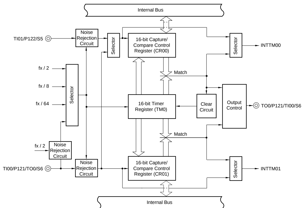
Figure 5-4: 16 bit Timer TM0
