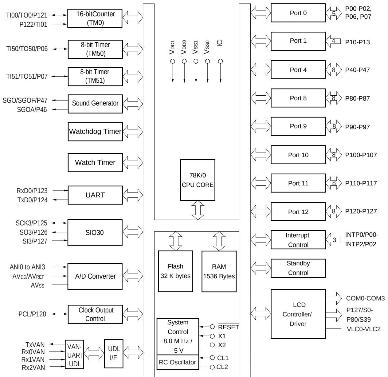
Figure 2-1: Block Diagram μPD1615
