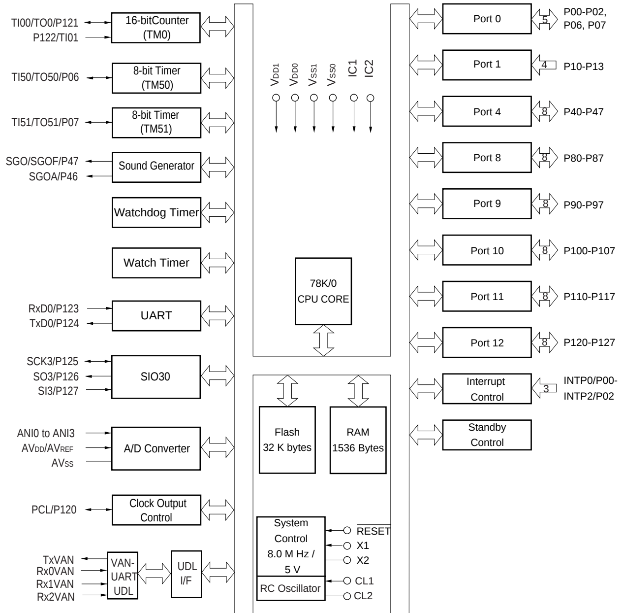
Figure 2-2: Block Diagram μPD1616
