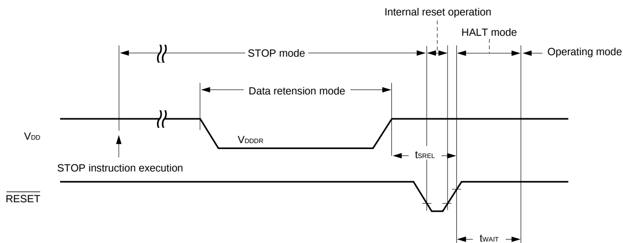
Figure 10-6: Data Retention Timing (STOP mode release by RESET)
