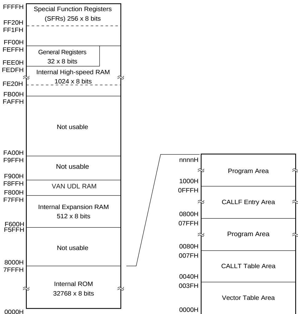
Figure 4-2: Memory Map (μPD1616)
