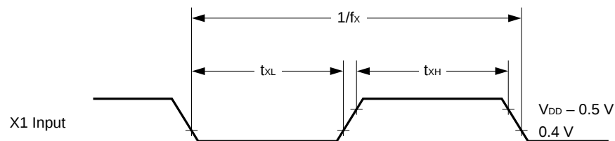
Figure 10-3: Clock Timing
