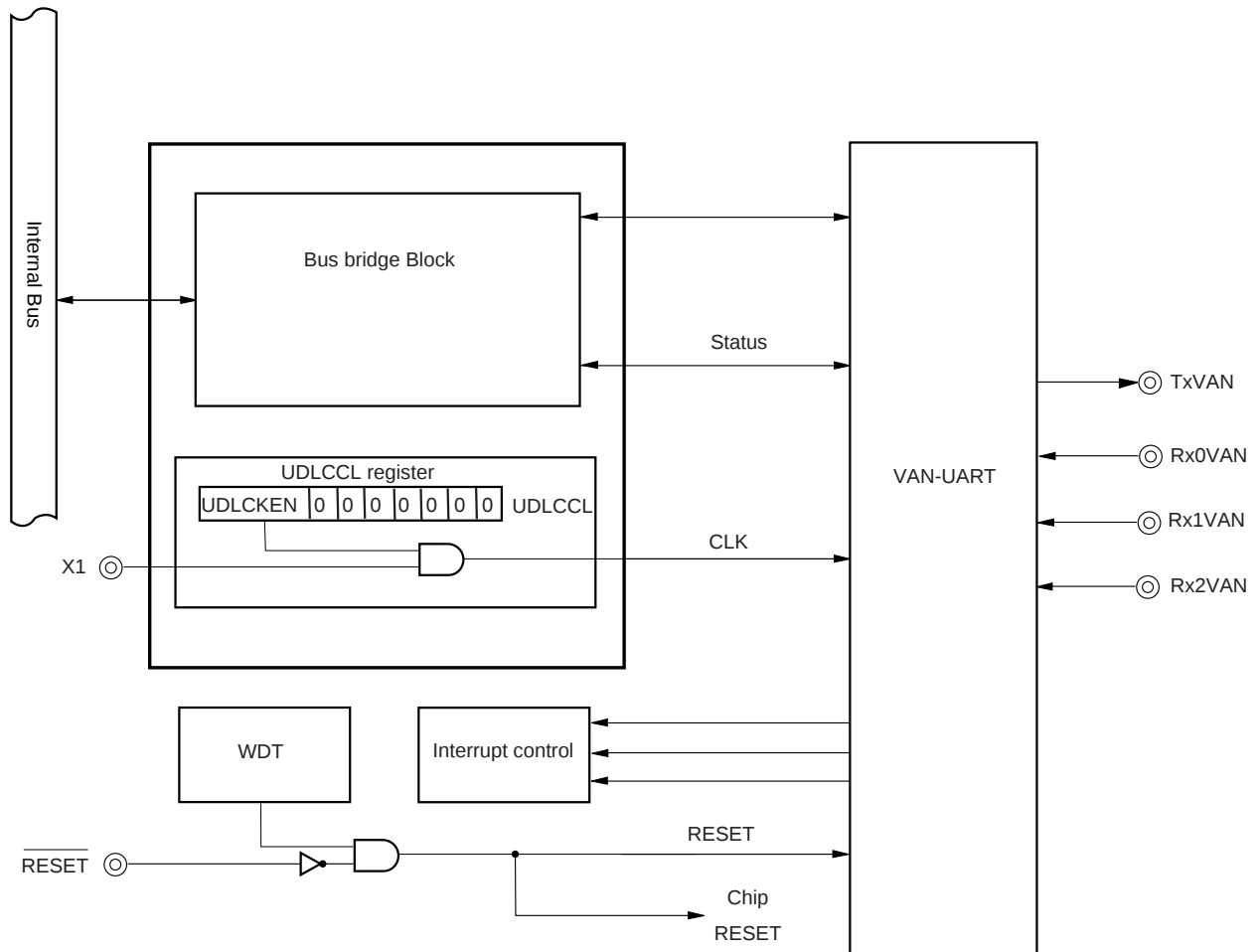
Figure 5-16: VAN-Bus Interface
