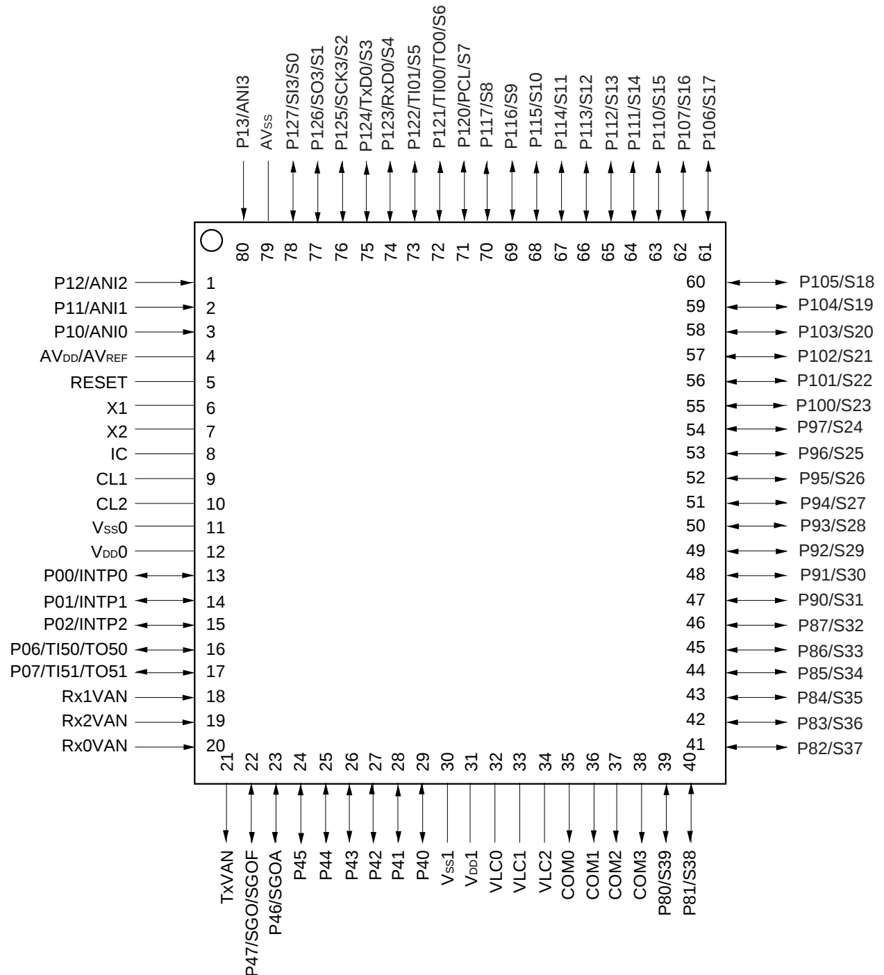
Figure 1-1: Pin Configuration μPD1615
