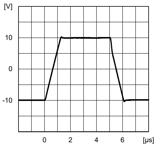
パルス応答特性 1 ( V^\pm = \pm 15\text{ V} , A_V = +1 ) (R_L = 2\text{ k}\Omega, C_L = 100\text{ pF})
