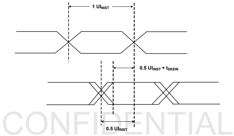
FIGURE 4. MIPI HIGH SPEED AC TIMING DIAGRAM
