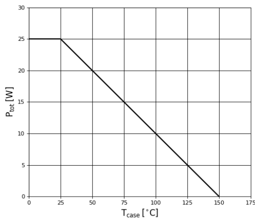
Figure 10. Power Dissipation
