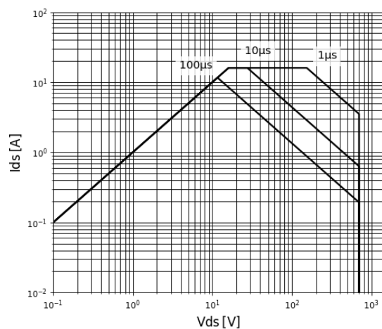
Figure 3. Safe Operating Area T_c = 25^\circ\text{C}
