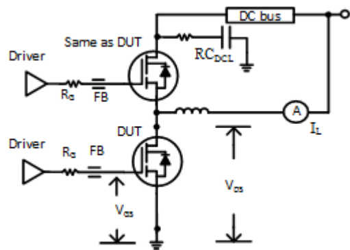
Figure 4. Switching Time Test Circuit
