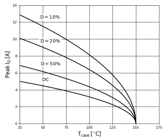
Figure 11. Current Derating
