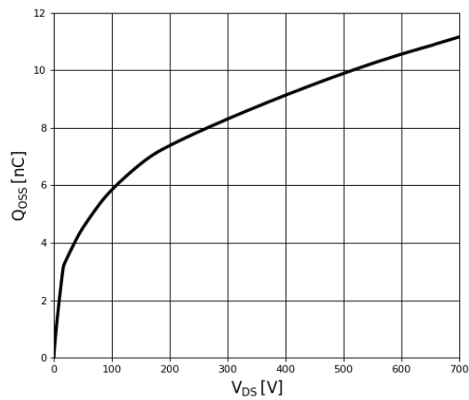
Figure 8. Typical QOSS
