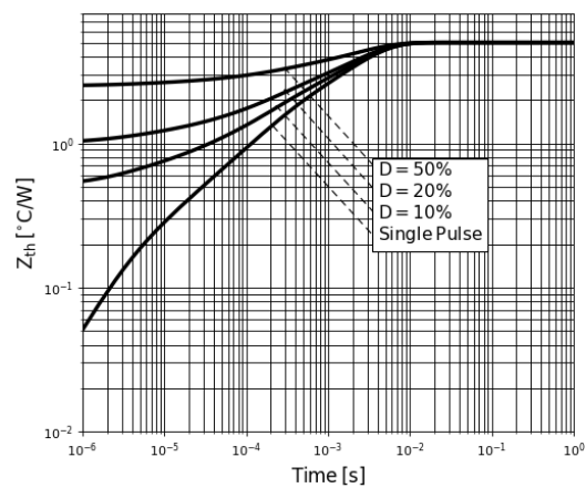
Figure 2. Transient Thermal Resistance
