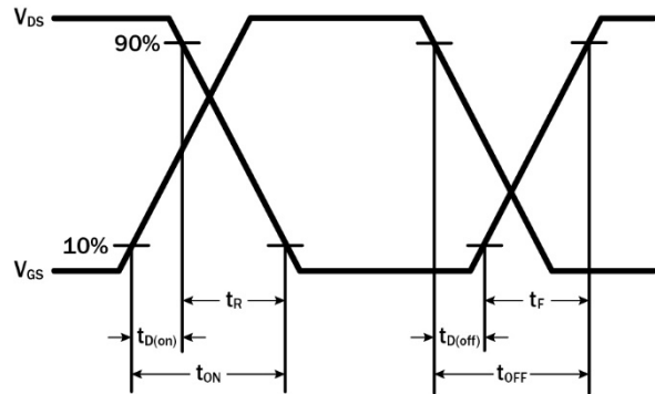
Figure 5. Switching Time Waveform
