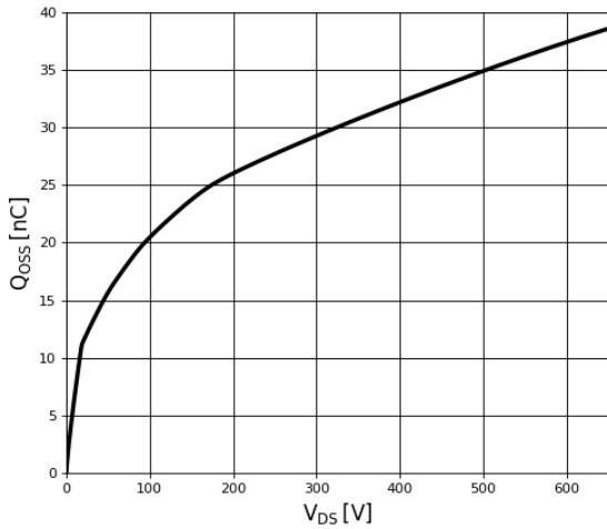
Figure 10. Typical Qoss
