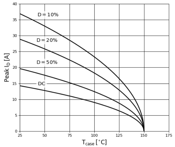
Figure 13. Current Derating Pulse width ≤ 10μs, V GS ≥ 6V
