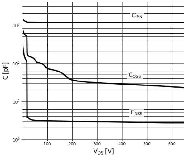
Figure 8. Typical Capacitance V_{GS} = 0V, f = 1MHz
