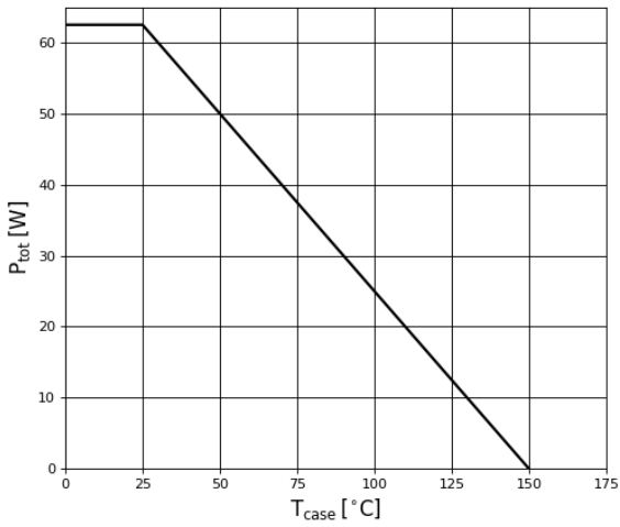
Figure 12. Power Dissipation
