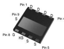
TP65H150G4LSGB PQFN (top view)
