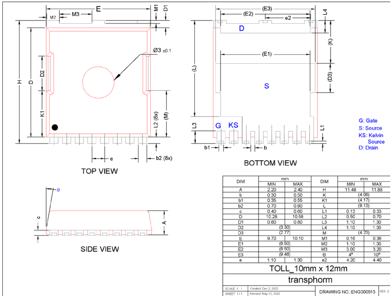
Figure 19. 10 x 12 mm TOLL Package Outline Drawing
