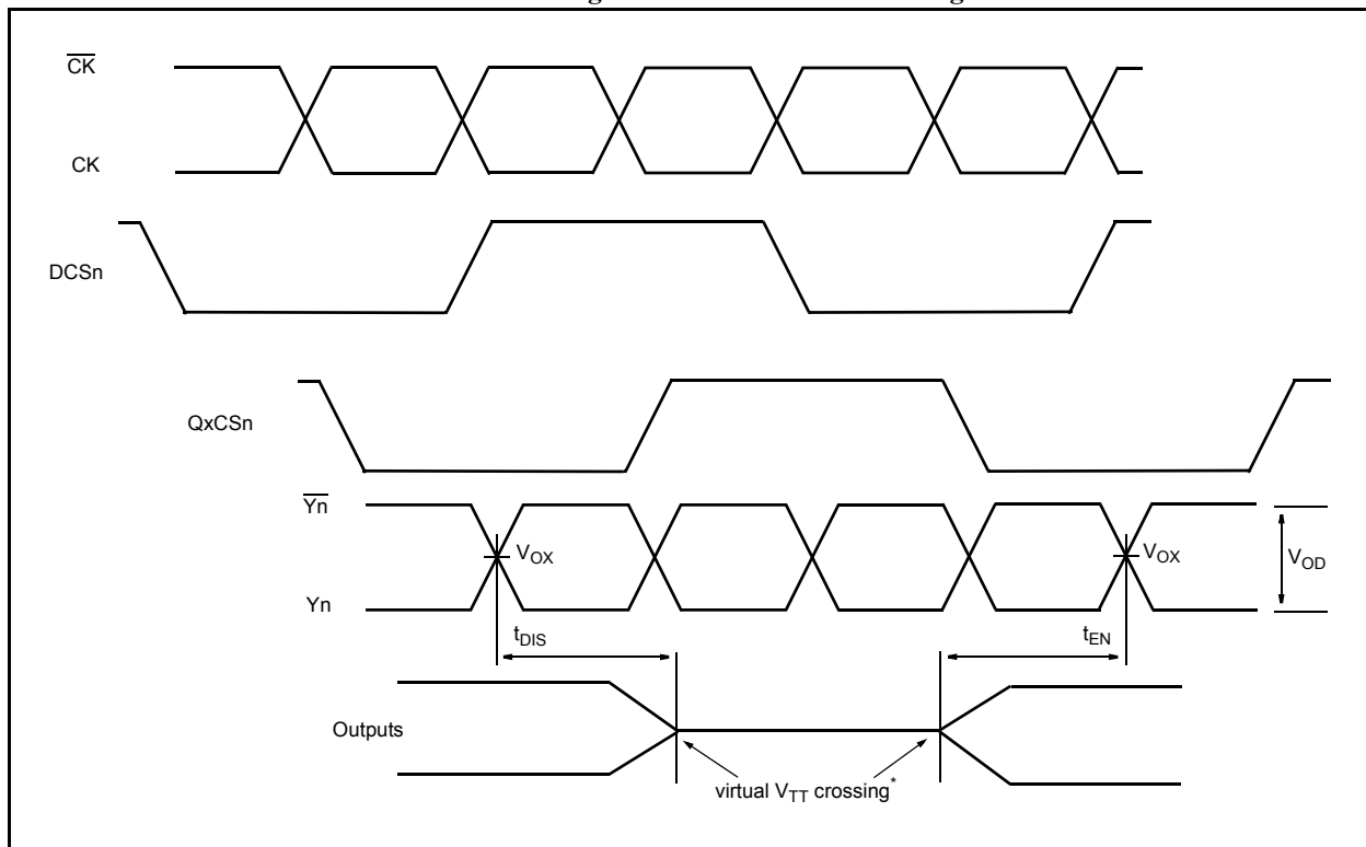
Voltage waveforms address floating
