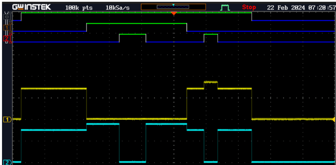
Figure 5. Chip Functionality
