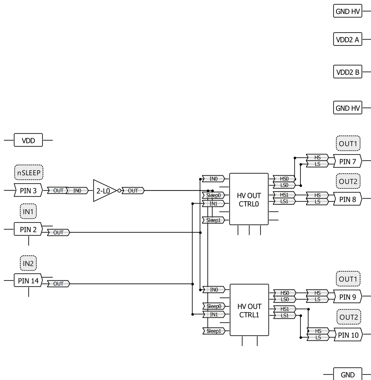
Figure 2. Block Diagram
