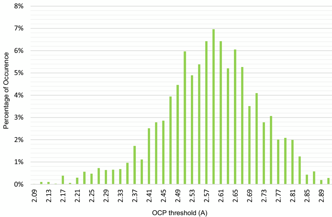
Figure 25. Full Bridge Low-side OCP Threshold Distribution at V_{DD}=2.3V to 5.5V , V_{DD2}=3V to 26.4V , T_J=-40^{\circ}C to 105^{\circ}C
