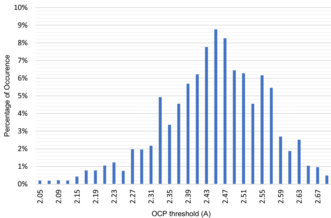
Figure 24. Full Bridge High-side OCP Threshold Distribution at V_{DD}=2.3\text{ V} to 5.5\text{ V} , V_{DD2}=3\text{ V} to 26.4\text{ V} , T_j=-40^\circ\text{C} to 105^\circ\text{C}
