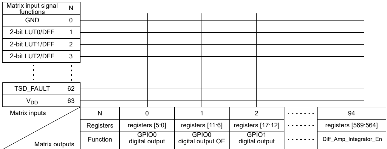
Figure 52. Connection Matrix
