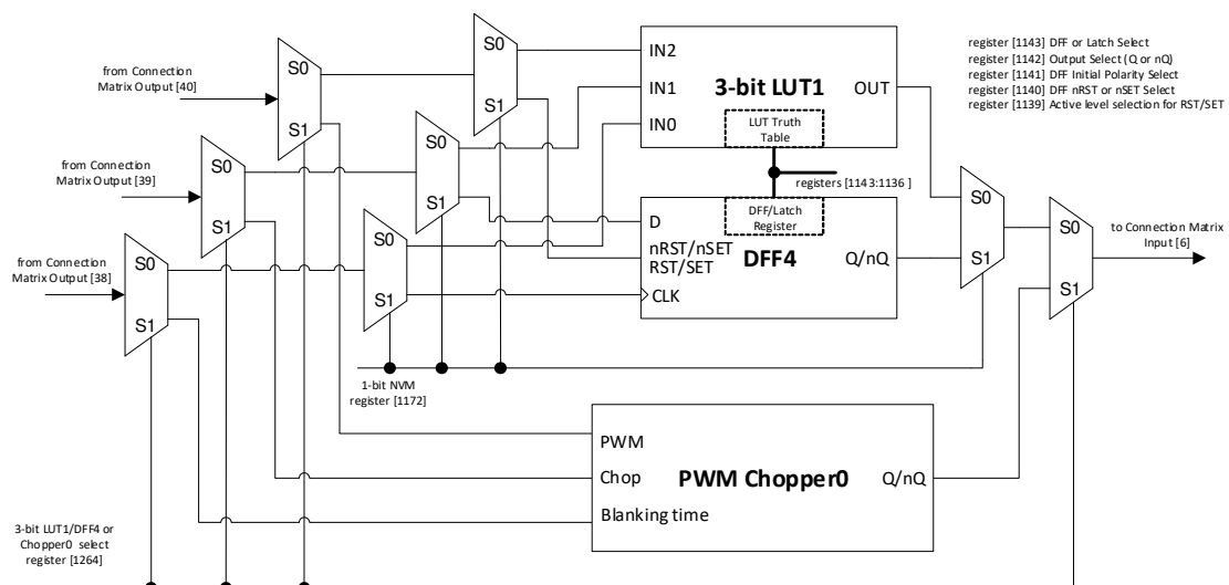
Figure 66. 3-bit LUT1 or DFF4
