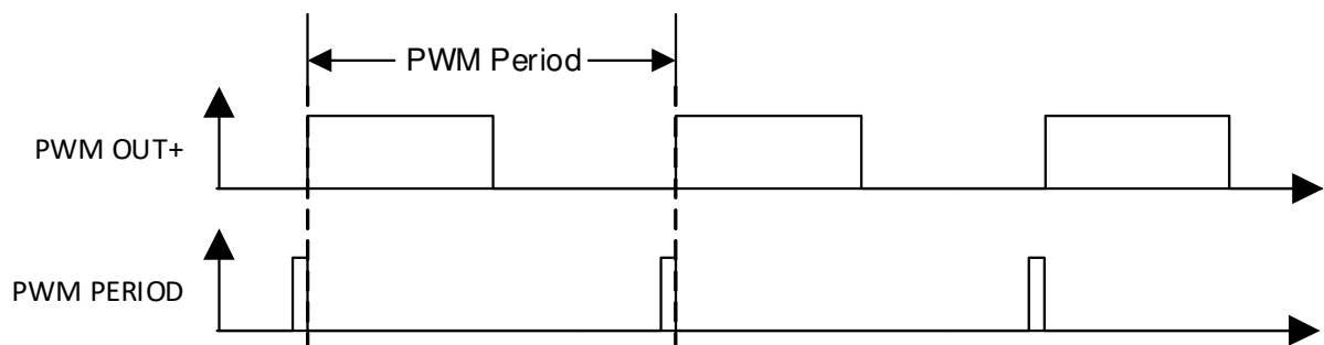
Figure 113. PWM Period Waveform
