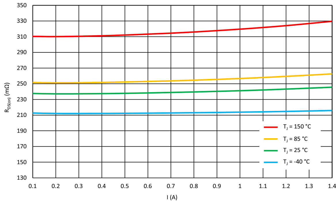
Figure 19. Full Bridge High-Side Typical Drain-Source On-Resistance vs. Load Current at V DD = 5.5 V, V DD2 = 5 V
