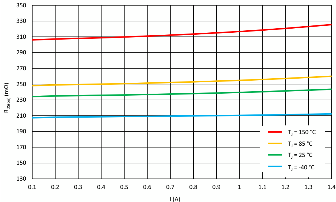
Figure 20. Full Bridge Low-Side Typical Drain-Source On-Resistance vs. Load Current at V DD = 5.5 V, V DD2 = 5 V
