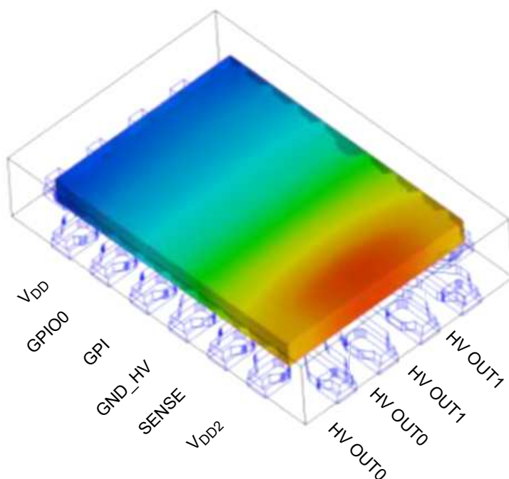
Figure 166. Die Temperature when HV OUTs are Active
