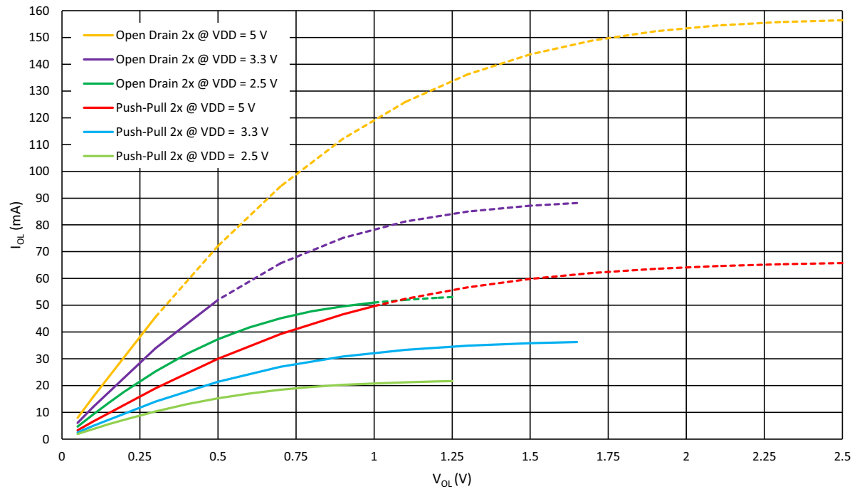
Figure 11. Typical Low Level Output Current vs. Low Level Output Voltage, 2x Drive at T_A = 25^\circ\text{C} , Full Range
