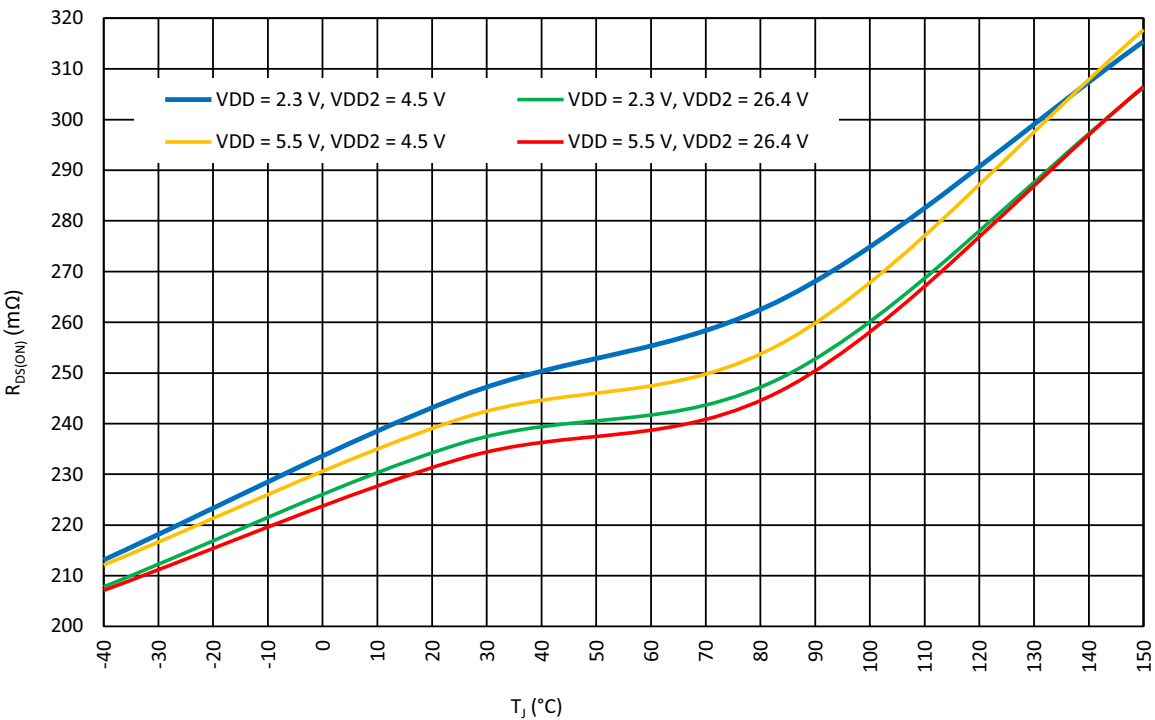
Figure 22. Full Bridge Low-Side Typical Drain-Source On-Resistance vs. Temperature at I LOAD = 0.5 A
