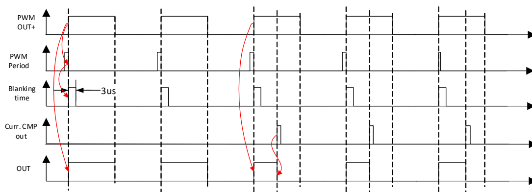
Figure 70. PWM Chopper. Overcurrent Timing Diagram
