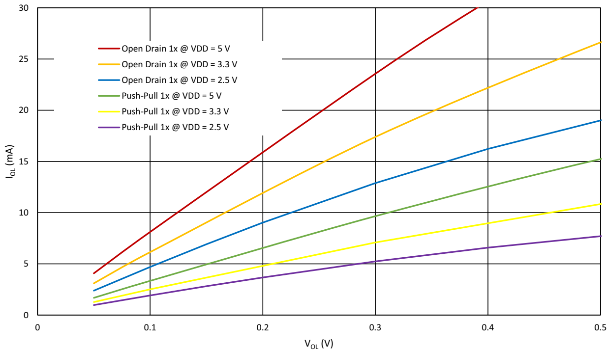
Figure 10. Typical Low Level Output Current vs. Low Level Output Voltage, 1x Drive at T_A = 25^\circ\text{C}
