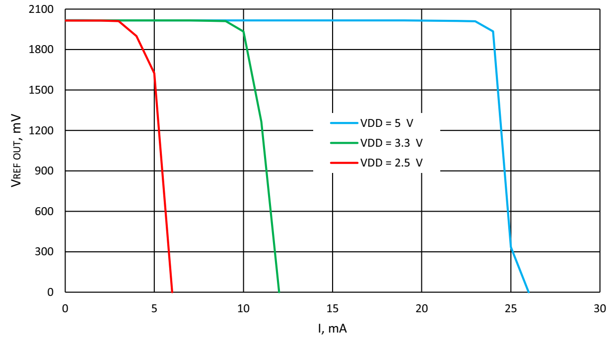
Figure 131. Typical Load Regulation, V_{ref} = 2016 \text{ mV} , T_A = -40^\circ\text{C} to +85^\circ\text{C} , Buffer - Enabled
