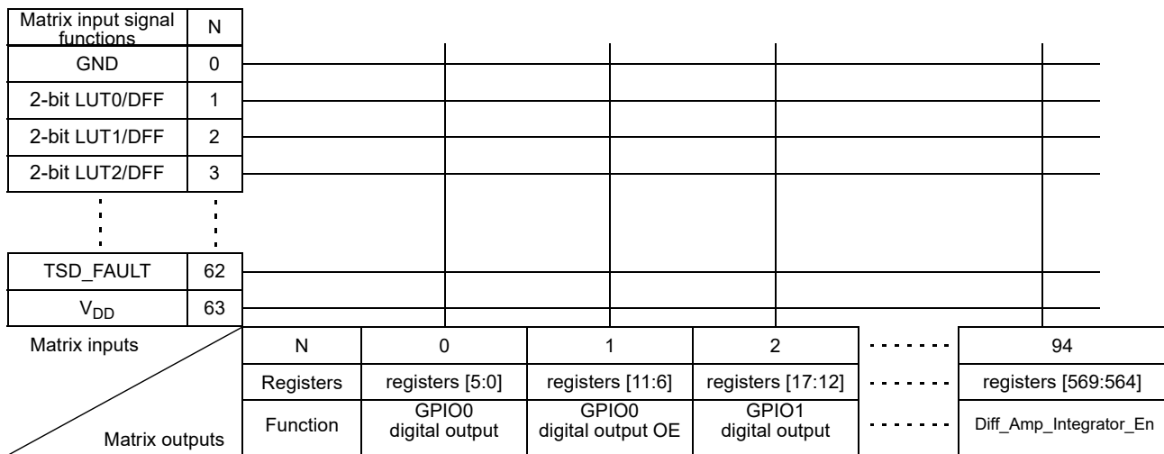
Figure 52. Connection Matrix
