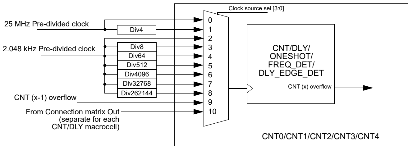
Figure 134. Clock Scheme
