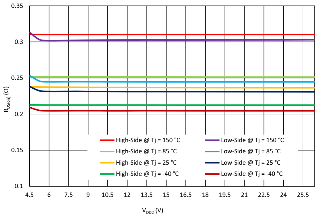
Figure 23. Full Bridge Typical Drain-Source On-Resistance vs. V_{DD2} at V_{DD} = 5.5\text{ V} , I_{LOAD} = 0.1\text{ A}
