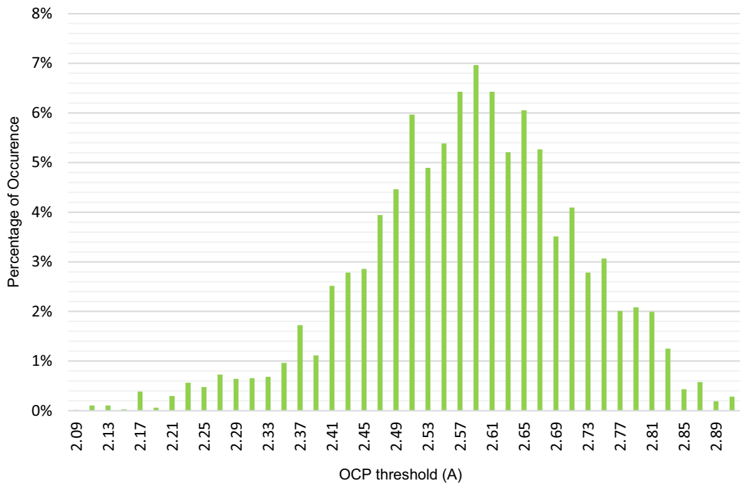
Figure 25. Full Bridge Low-side OCP Threshold Distribution at V_{DD}=2.3V to 5.5V , V_{DD2}=3V to 26.4V , T_J=-40^{\circ}C to 150^{\circ}C
