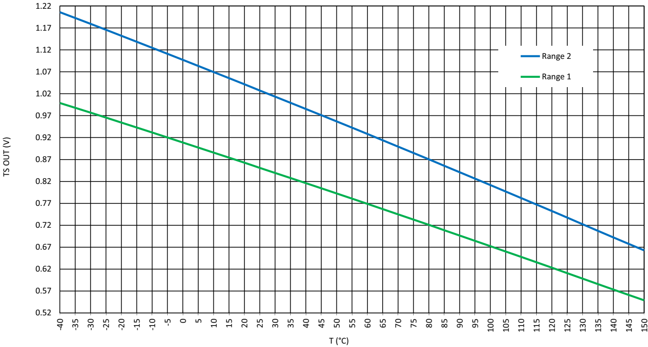
Figure 159. TS Output vs. Temperature, V DD = 2.3 V to 5.5 V
