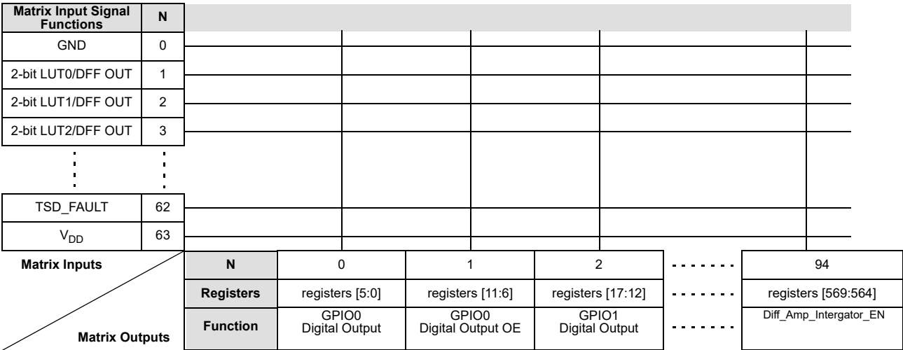
Figure 47. Connection Matrix
