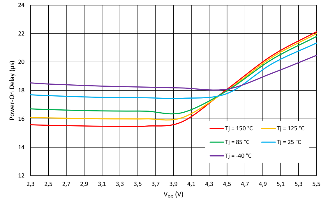
Figure 115. ACMPxH Power-On Delay vs. V DD
