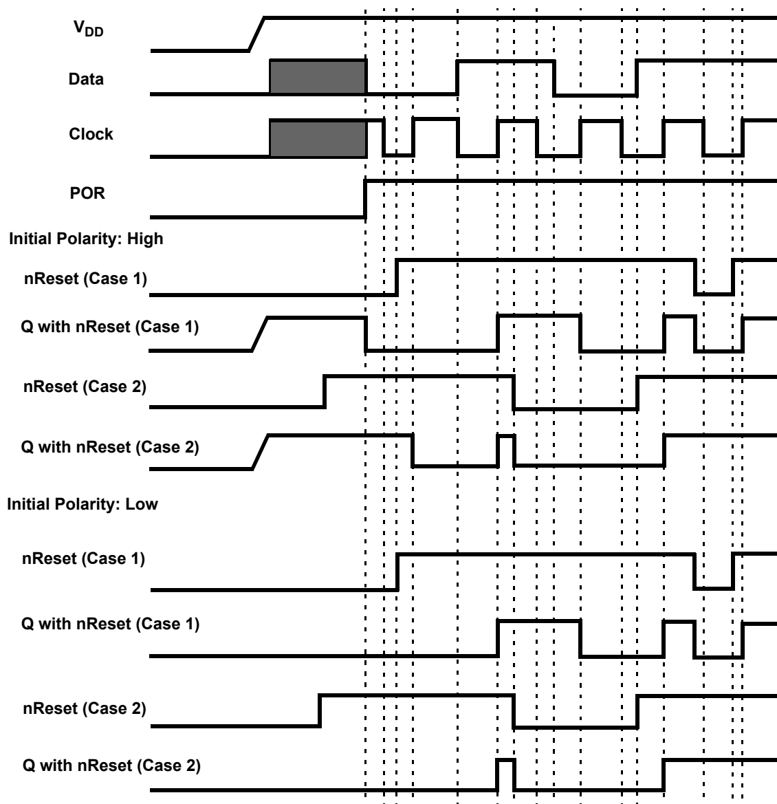
Figure 59. DFF Polarity Operations with n\text{Reset}
