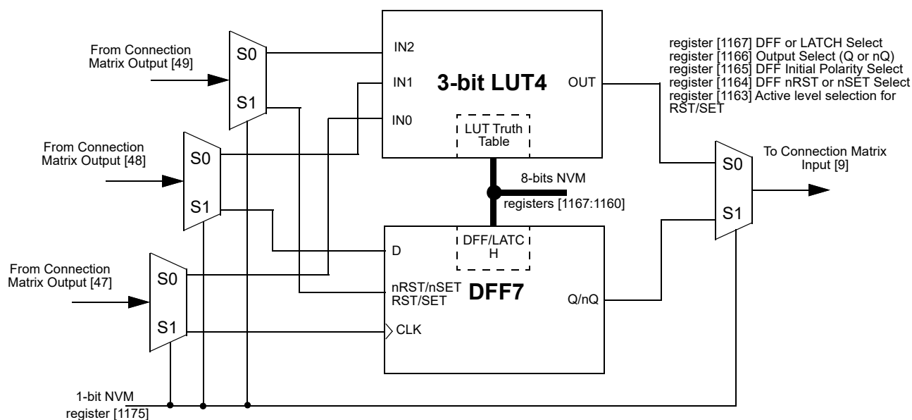
Figure 57. 3-bit LUT4 or DFF7
