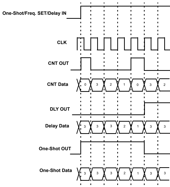
Figure 93. Counter Value, Counter Data = 3
