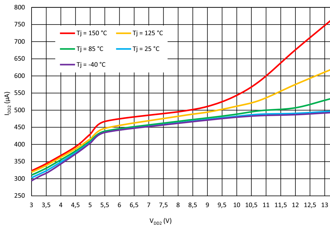
Figure 38. One Full Bridge + Integrator + PWM + OSC1 + One CCMP I_{DD2} vs. V_{DD2} at V_{DD} = 5.5 V
