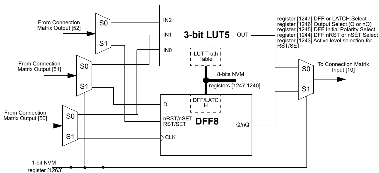
Figure 58. 3-bit LUT5 or DFF8
