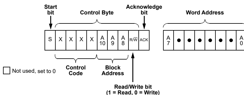
Figure 116. Basic Command Structure
