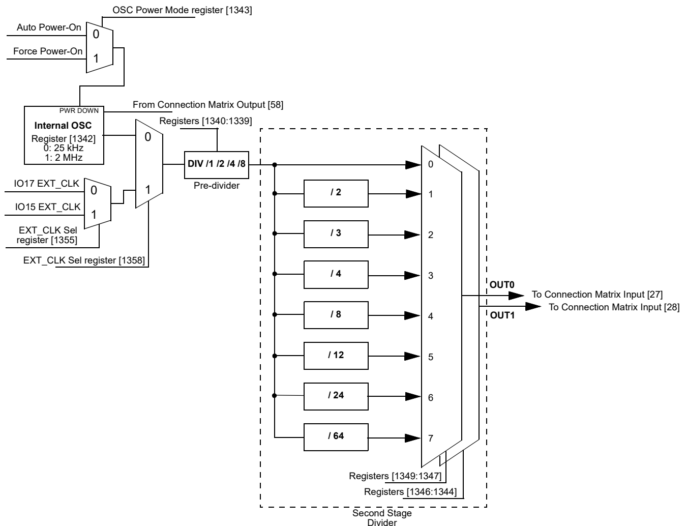
Figure 72. 25 kHz/2 MHz OSC0 Block Diagram
