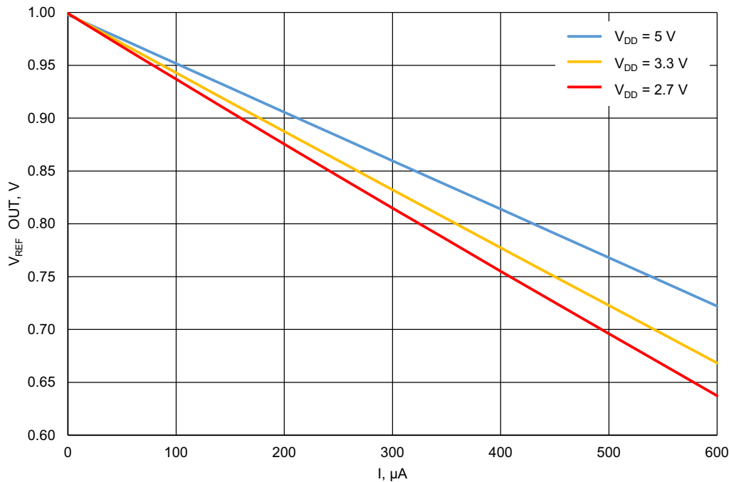
Figure 70. Typical Load Regulation, V REF = 1000 mV, T A = -40 °C to 125 °C, Buffer - Enable
