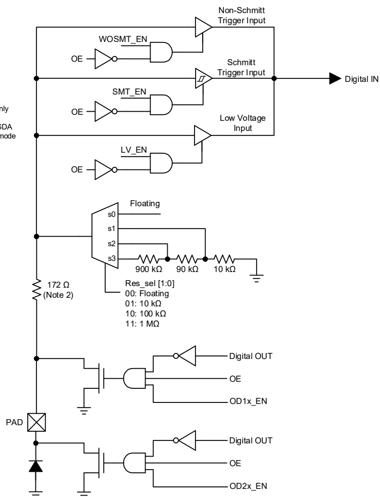
Figure 9. IO Structure Diagram
