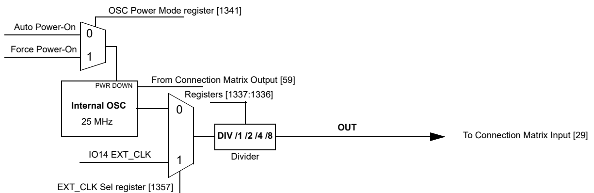
Figure 73. 25 MHz OSC1 Block Diagram
