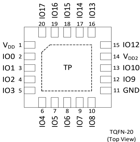
Figure 2. Pin Assignments - TQFN-20 (Top View)
