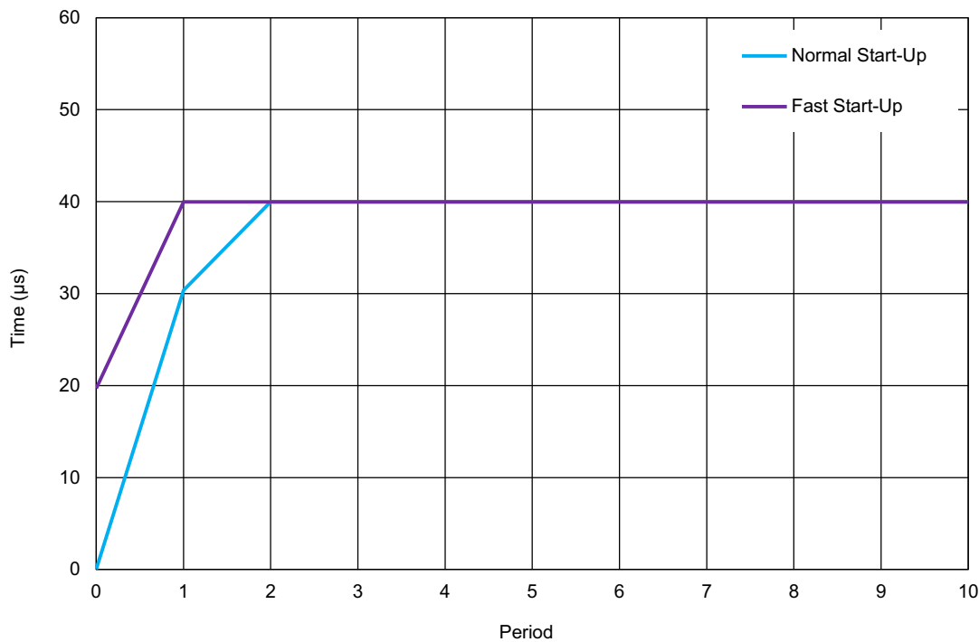
Figure 82. Oscillator0 Settling Time, V_{DD} = 3.3\text{ V} , T_A = 25\text{ °C} , OSC0 = 25 kHz
