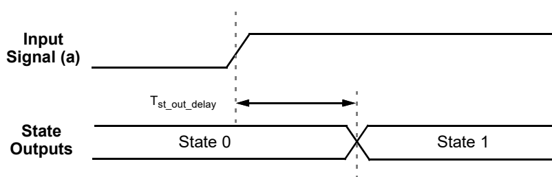
Figure 104. State Transition Timing
