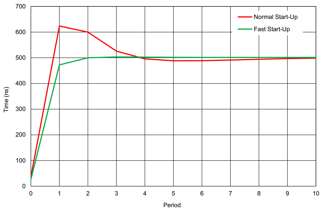
Figure 83. Oscillator0 Settling Time, V_{DD} = 3.3\text{ V} , T_A = 25\text{ }^{\circ}\text{C} , OSC0 = 2\text{ MHz}
