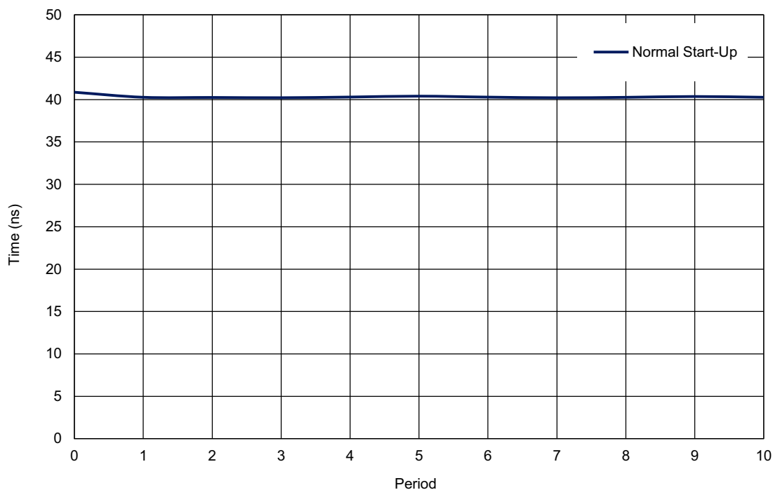
Figure 84. Oscillator1 Settling Time, V_{DD} = 3.3\text{ V} , T_A = 25\text{ }^{\circ}\text{C} , OSC2 = 25\text{ MHz}
