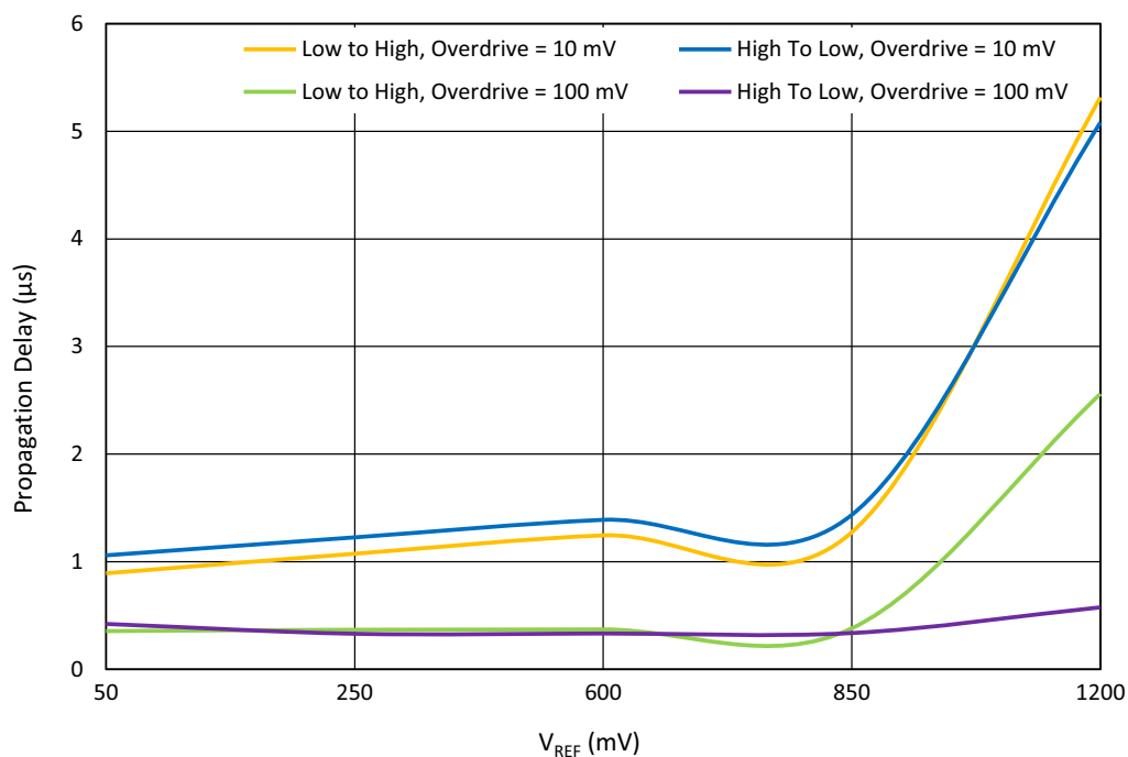
Figure 61. ACMPx Propagation Delay at T_A = 25\text{ }^{\circ}\text{C} , Gain = 1, Hysteresis = 0, V_{DD} = 1.71\text{ V} to 5.5 V, LPF – Disable
