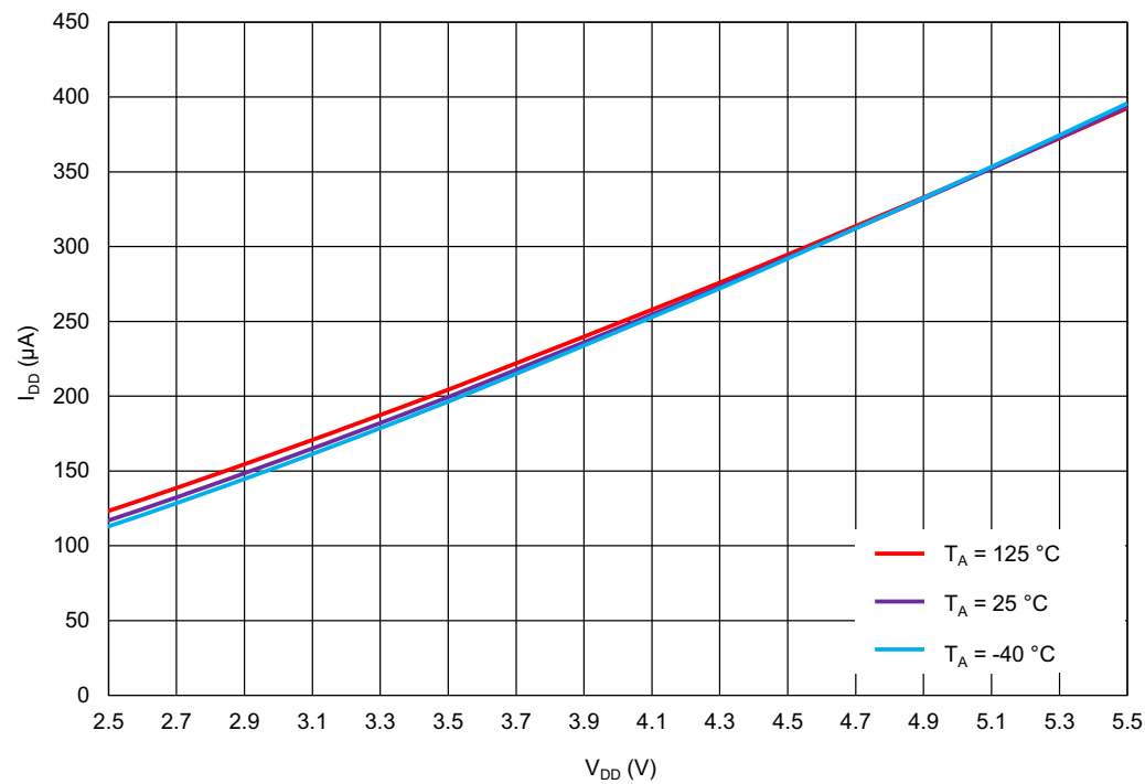
Figure 93. OSC1 (25 MHz) Current Consumption vs. V_{DD} , Pre-Divider = 8
