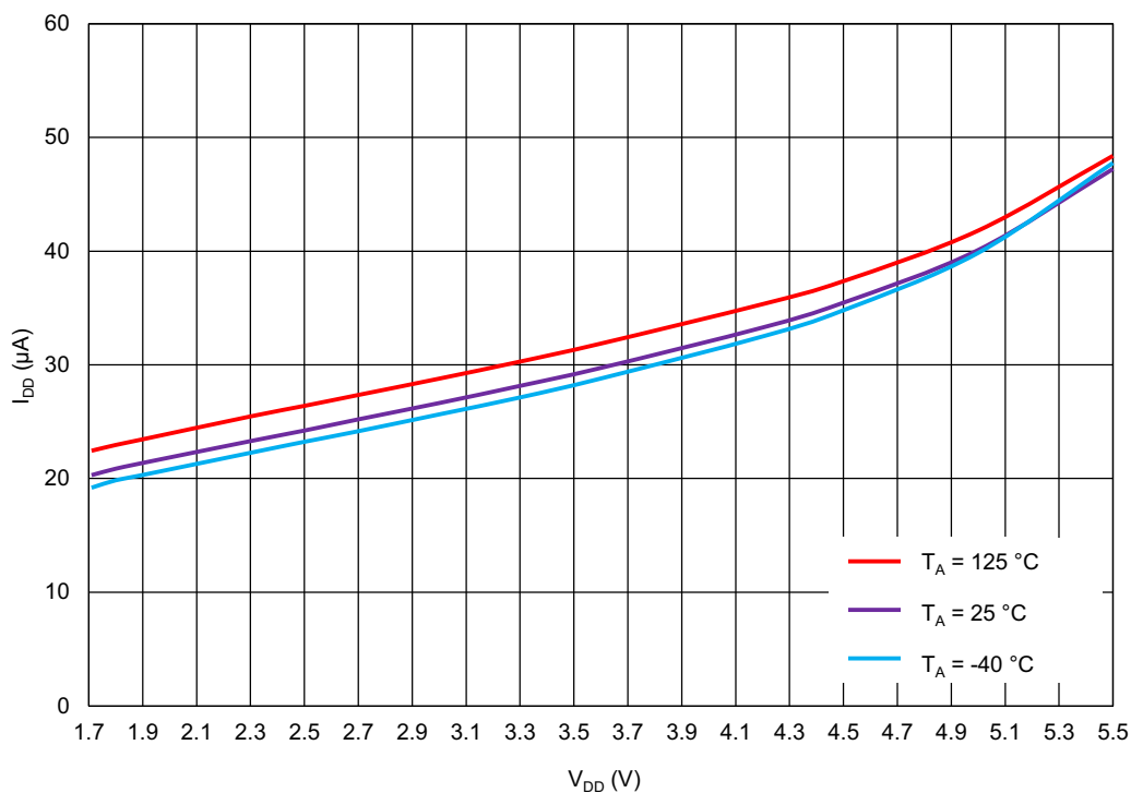
Figure 88. OSC0 (2 MHz) Current Consumption vs. V DD , Pre-Divider = 4
