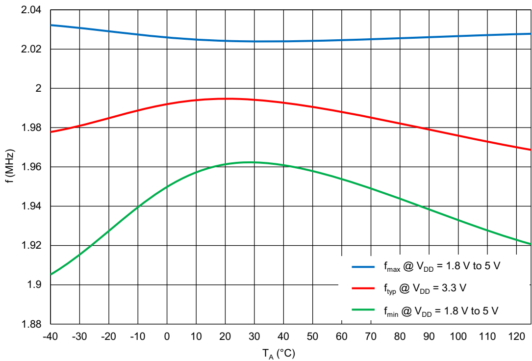
Figure 79. Oscillator Frequency vs. Ambient Temperature, OSC0 = 2 MHz
