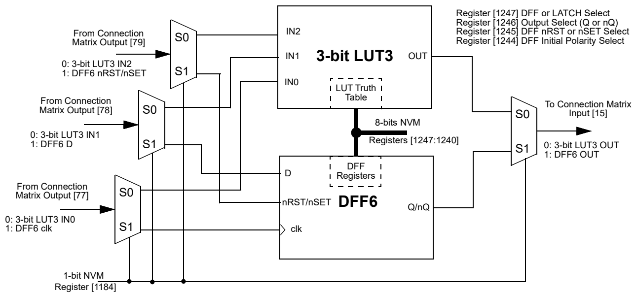
Figure 21. 3-bit LUT3 or DFF6 with RST/SET
