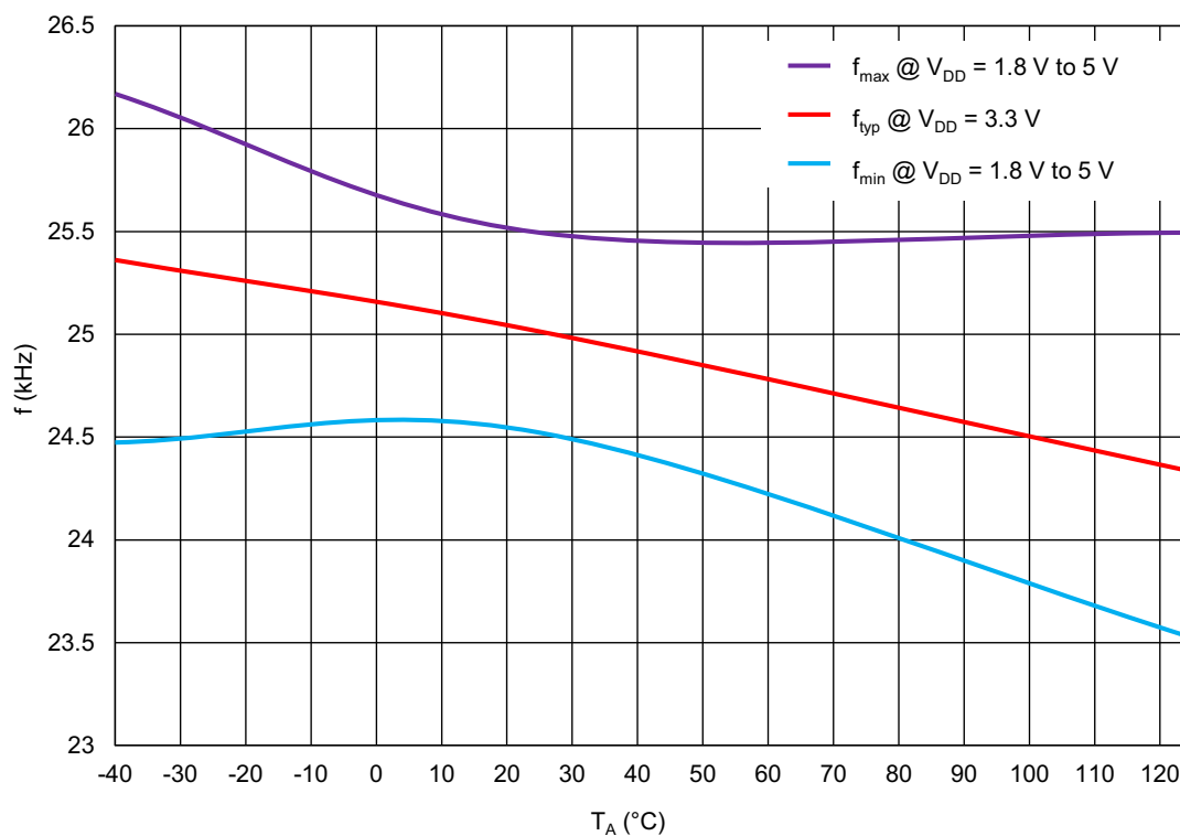
Figure 78. Oscillator Frequency vs. Ambient Temperature, OSC0 = 25 kHz
