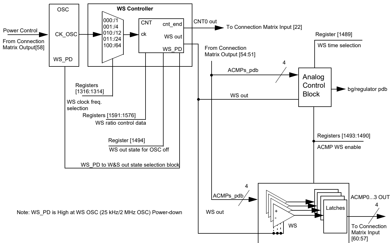
Figure 52. Wake/Sleep Controller
