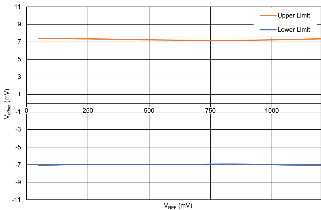
Figure 58. ACMPx Input Offset Voltage vs. V REF at V DD = 1.71 V to 5.5 V, T A = -40 °C to 125 °C
