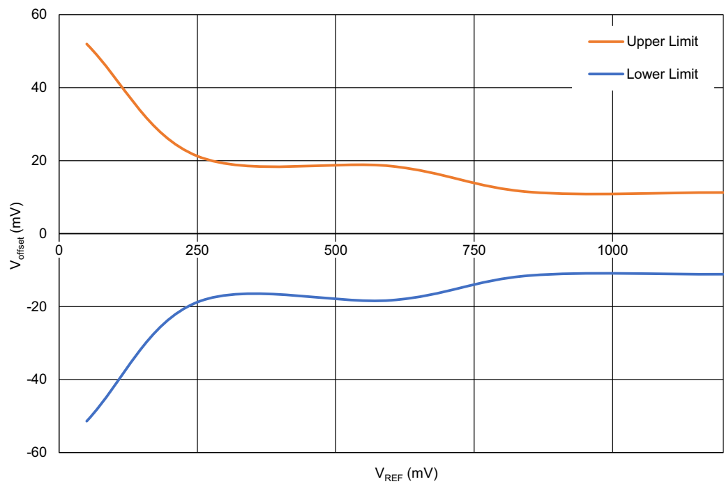
Figure 59. ACMPx Buffer Input Offset Voltage vs. V REF at V DD = 1.71 V to 5.5 V, T A = -40 °C to 125 °C
