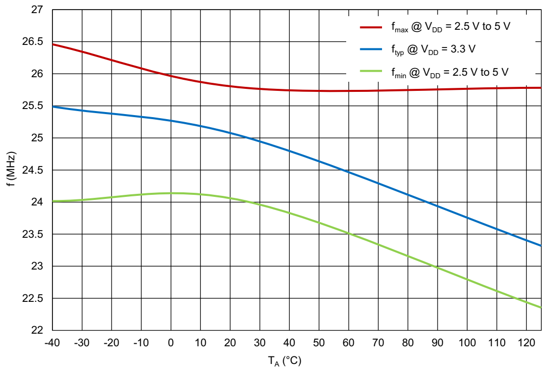
Figure 80. Oscillator Frequency vs. Ambient Temperature, OSC1 = 25 MHz
