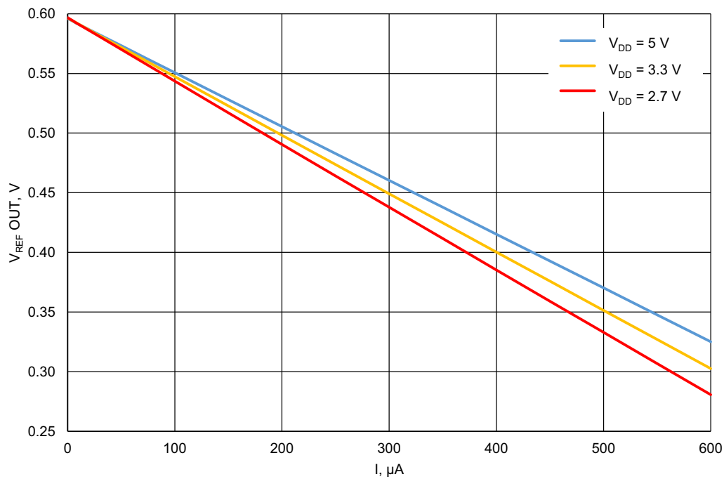
Figure 69. Typical Load Regulation, V REF = 600 mV, T A = -40 °C to 125 °C, Buffer - Enable
