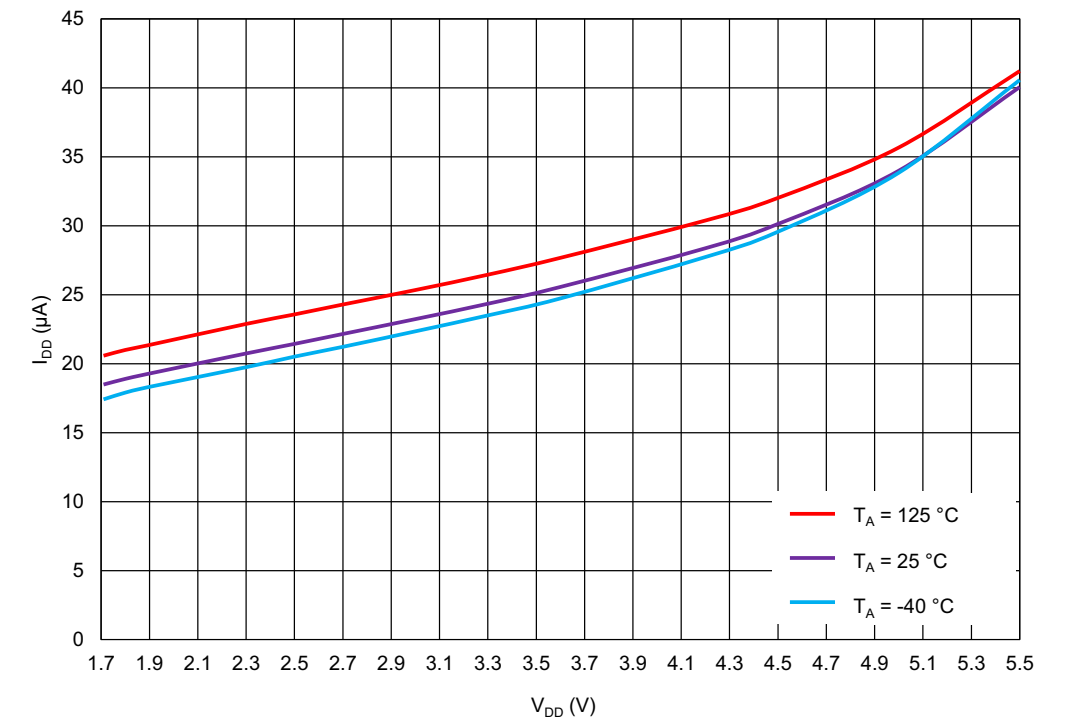
Figure 89. OSC0 (2 MHz) Current Consumption vs. V DD , Pre-Divider = 8
