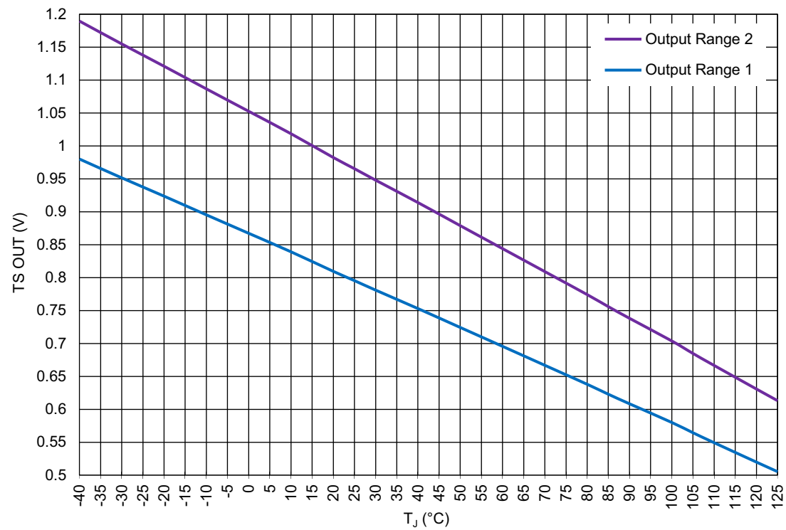
Figure 126. TS Output vs. Temperature, V DD = 1.71 V to 5.5 V
