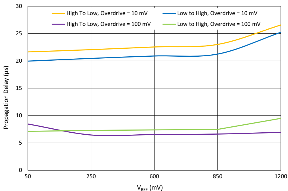
Figure 60. ACMPx Propagation Delay at T_A = 25\text{ }^{\circ}\text{C} , Gain = 1, Hysteresis = 0, V_{DD} = 1.71\text{ V} to 5.5 V, LPF – Enable
