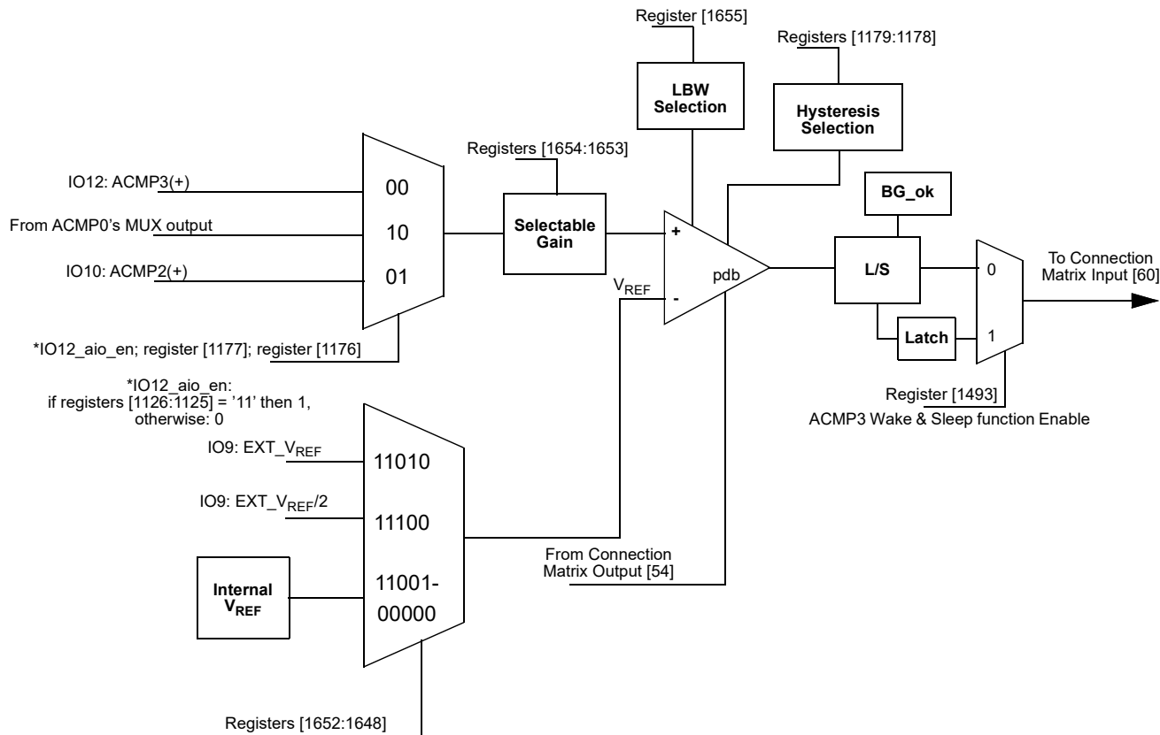
Figure 56. ACMP3 Block Diagram
