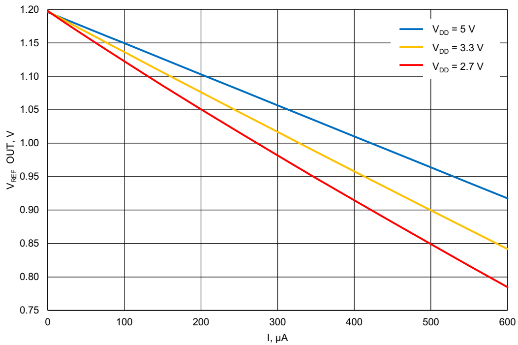
Figure 71. Typical Load Regulation, V_{REF} = 1200\text{ mV} , T_A = -40\text{ }^{\circ}\text{C} to 125\text{ }^{\circ}\text{C} , Buffer - Enable
