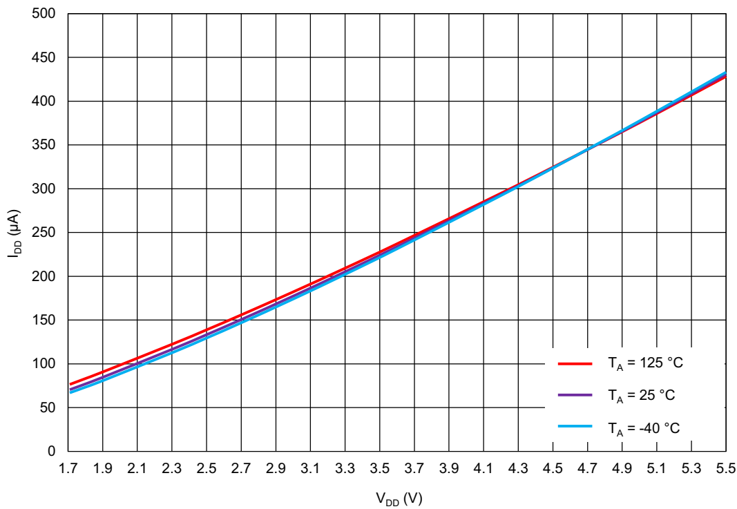
Figure 90. OSC1 (25 MHz) Current Consumption vs. V DD , Pre-Divider = 1
