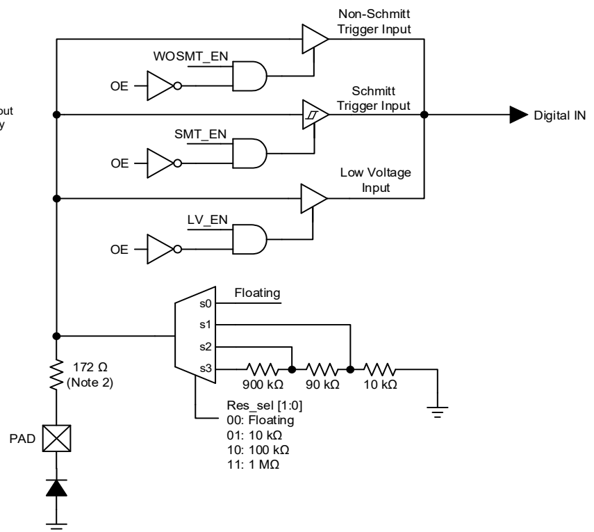
Figure 4. IO0 GPI Structure Diagram
