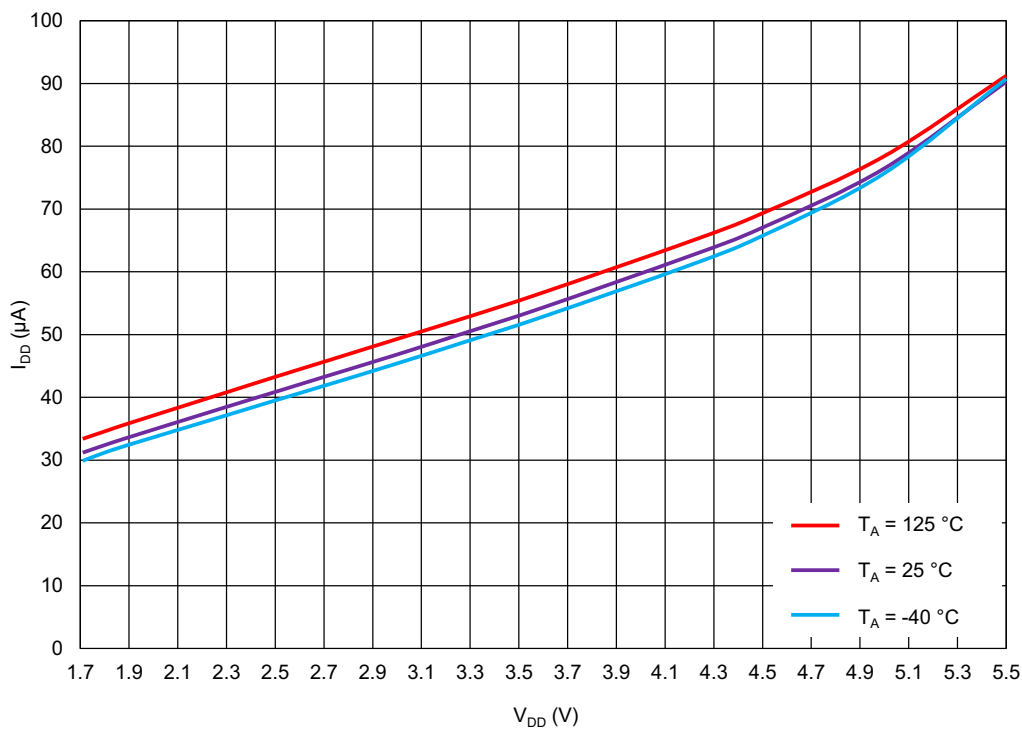
Figure 86. OSC0 (2 MHz) Current Consumption vs. V_{DD} , Pre-Divider = 1
