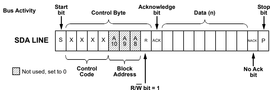
Figure 117. Current Address Read Command, \overline{R/W} = 1
