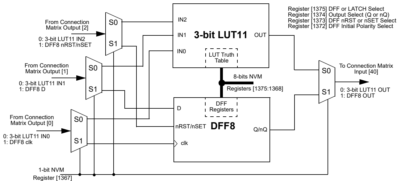
Figure 21. 3-bit LUT11 or DFF8 with RST/SET
