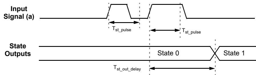
Figure 106. State Transition Pulse Input Timing
