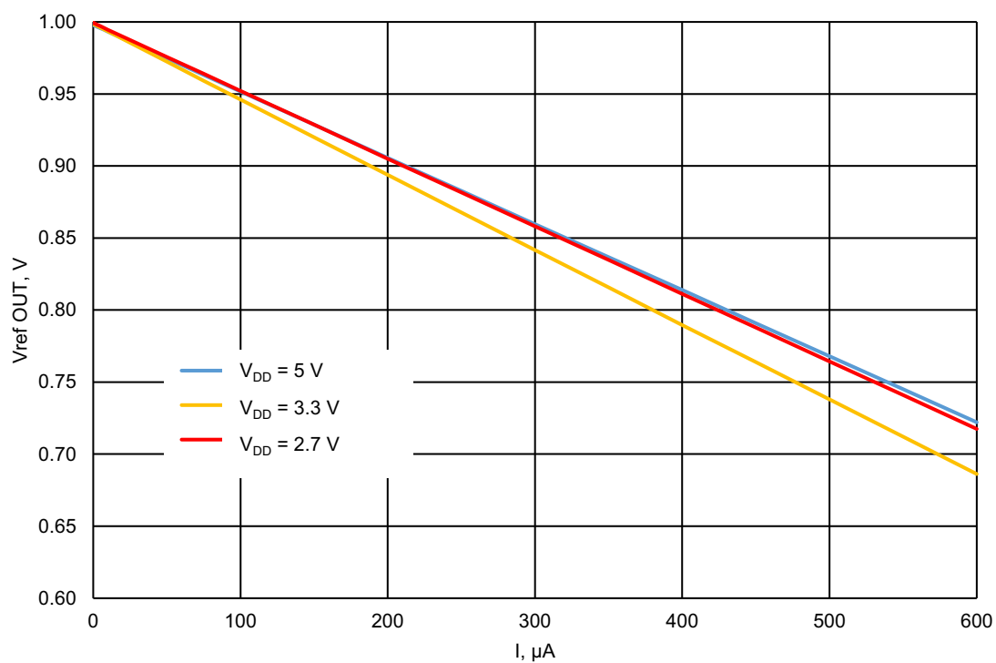
Figure 69. Typical Load Regulation, V_{REF} = 1200\text{ mV} , T_A = -40\text{ }^{\circ}\text{C} to +105\text{ }^{\circ}\text{C} , Buffer - Enable
