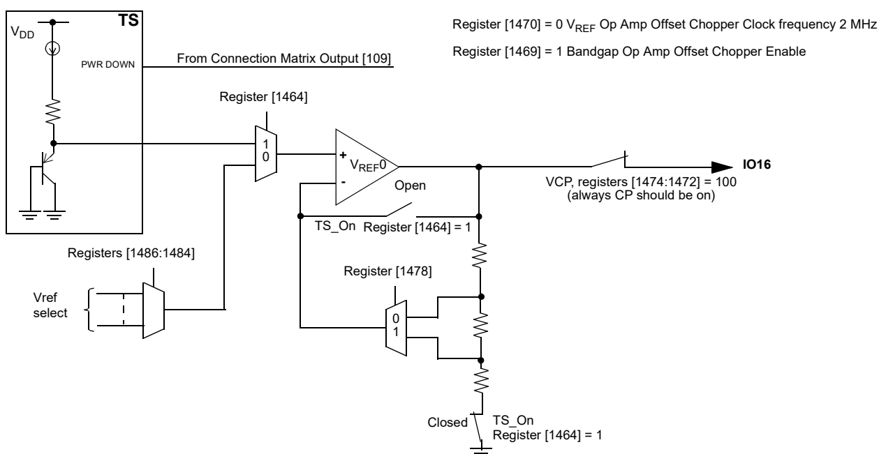
Figure 122. Analog Temperature Sensor Structure Diagram
