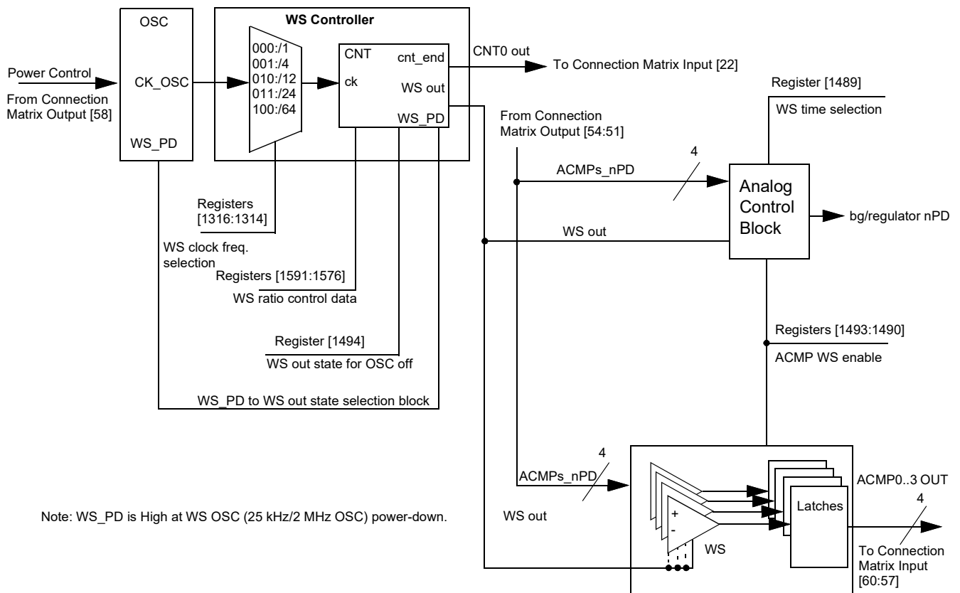
Figure 51. Wake/Sleep Controller
