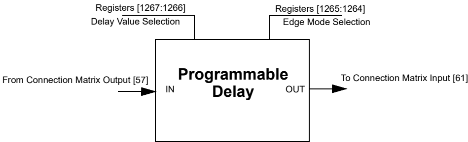
Figure 63. Programmable Delay
