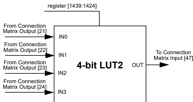
Figure 52. 4-bit LUT2
