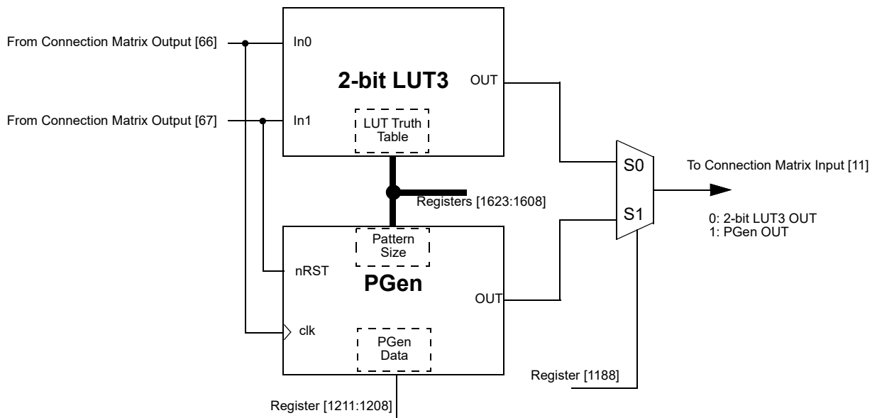
Figure 49. 2-bit LUT3 or PGen
