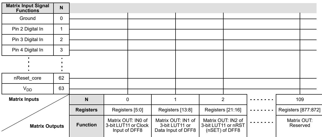
Figure 10. Connection Matrix
