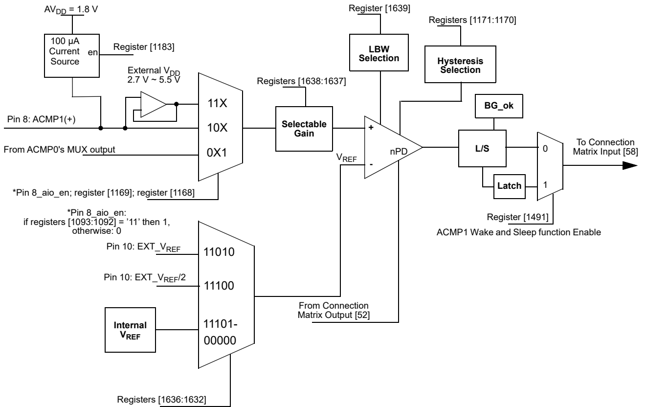
Figure 54. ACMP1 Block Diagram
