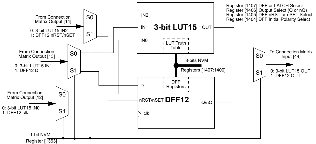
Figure 25. 3-bit LUT15 or DFF12 with RST/SET
