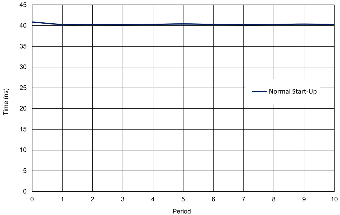
Figure 75. Oscillator Maximum Power-On Delay vs. V_{DD} at T_A = +25\text{ }^\circ\text{C} , OSC1 = 25 MHz
