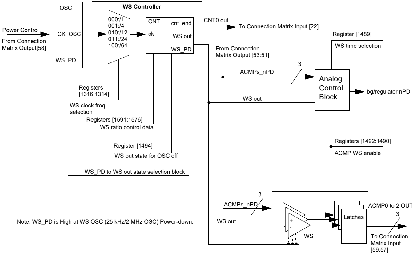
Figure 51. Wake/Sleep Controller
