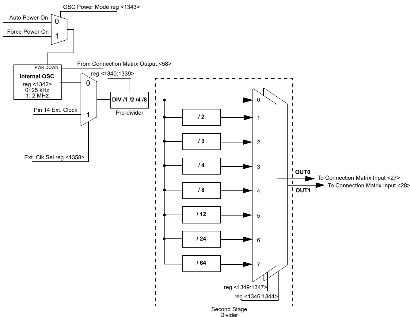
Figure 70. 25 kHz/2 MHz OSC0 Block Diagram
