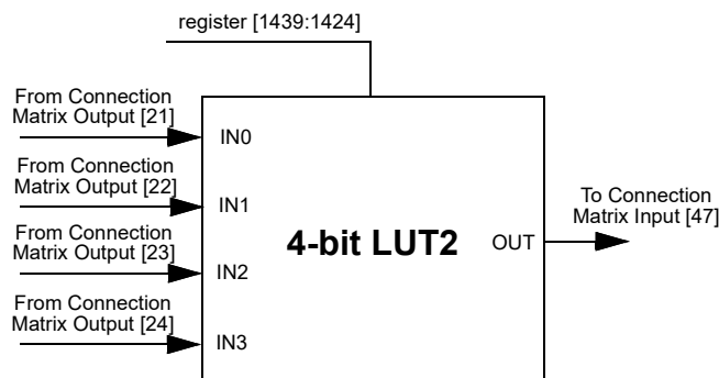
Figure 52. 4-bit LUT2
