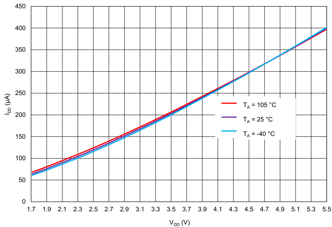
Figure 82. OSC1 (25 MHz) Current Consumption vs. V_{DD} , Pre-Divider = 4
