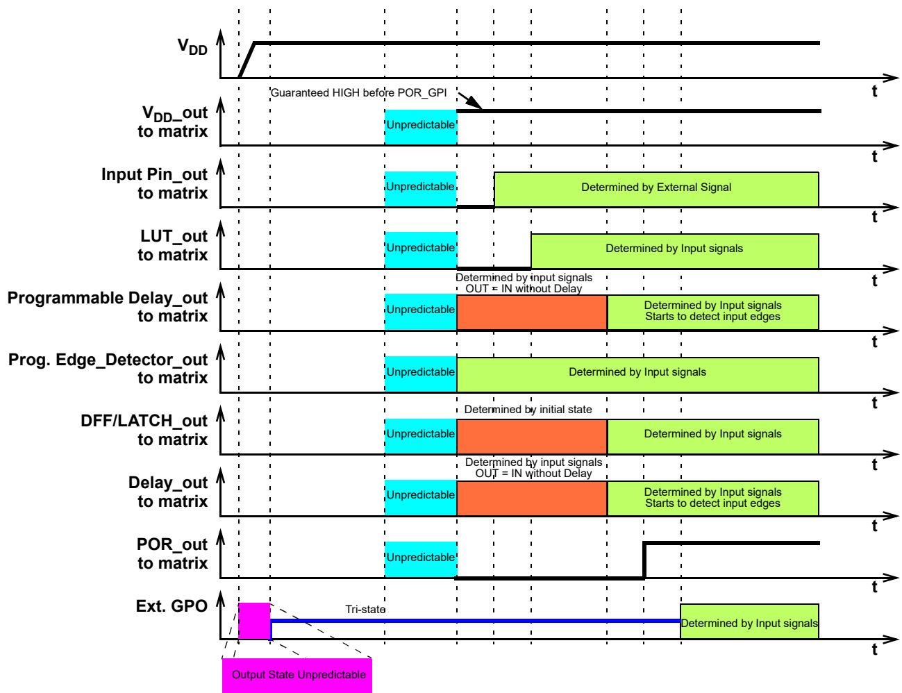
Figure 85. Internal Macrocell States during POR Sequence
