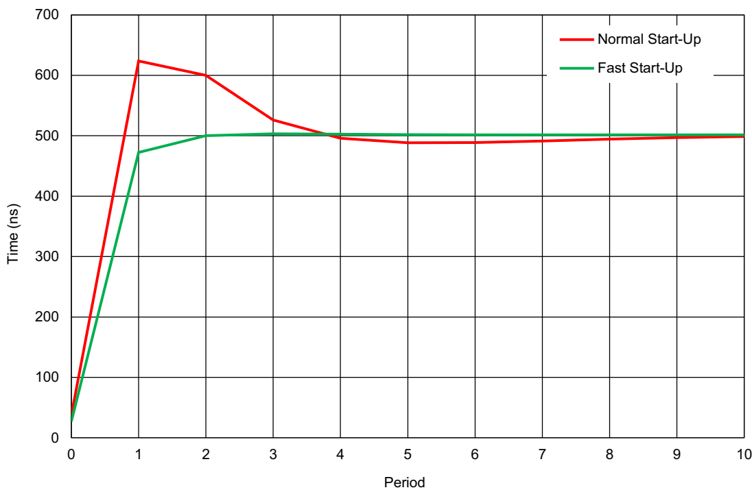
Figure 73. Oscillator0 Settling Time, V_{DD} = 3.3\text{ V} , T_A = +25\text{ }^{\circ}\text{C} , \text{OSC0} = 2\text{ MHz}
