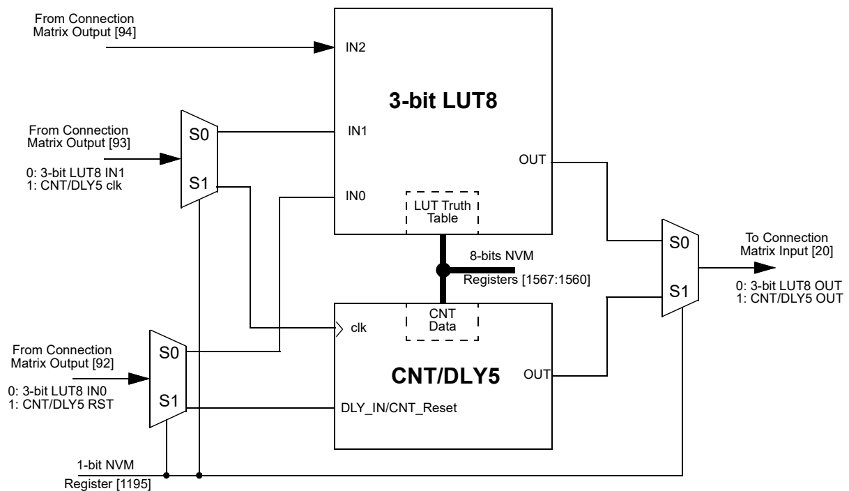
Figure 27. 3-bit LUT8 or CNT/DLY5
