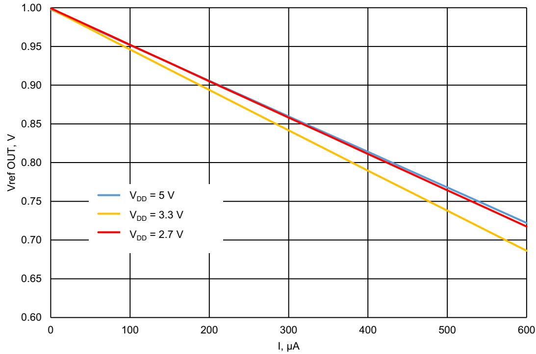
Figure 61. Typical Load Regulation, V REF = 1200 mV, T A = -40 °C to +105 °C, Buffer - Enable
