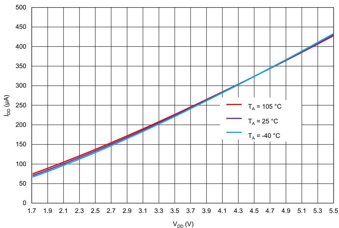
Figure 80. OSC1 (25 MHz) Current Consumption vs. V DD , Pre-Divider = 1
