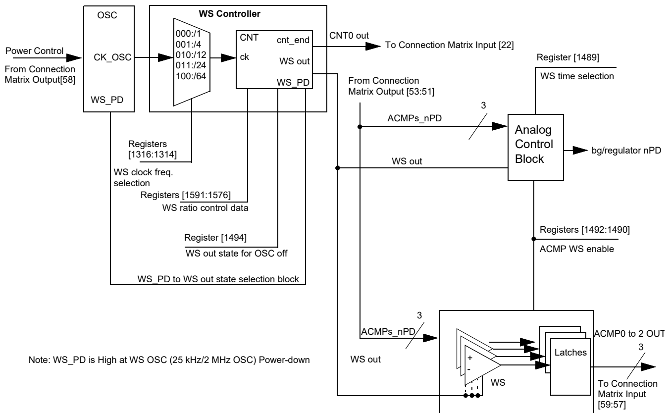
Figure 44. Wake/Sleep Controller
