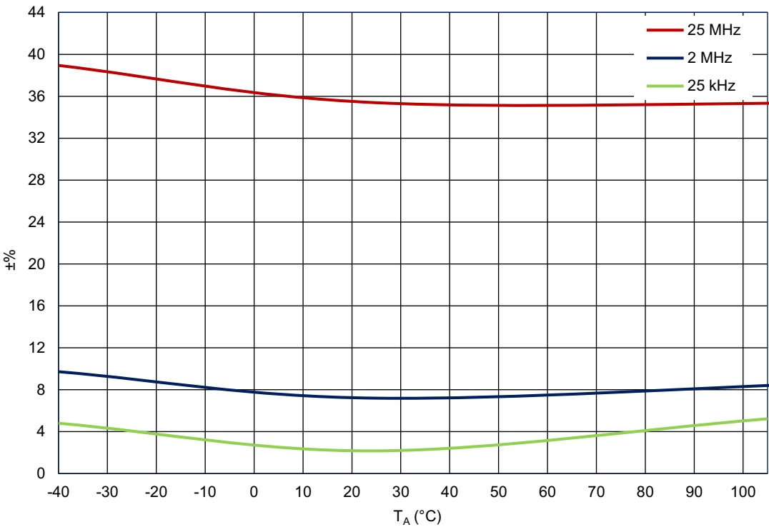
Figure 71. Oscillators Total Error vs. Ambient Temperature
