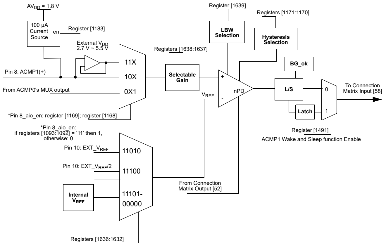
Figure 46. ACMP1 Block Diagram
