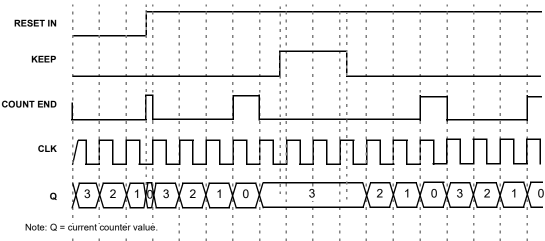
Figure 37. CNT/FSM Timing Diagram (Reset Rising Edge Mode, Oscillator is Forced On, UP = 0) for Counter Data = 3
