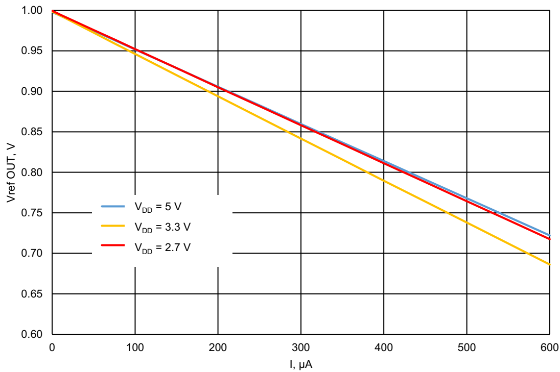
Figure 60. Typical Load Regulation, V REF = 1000 mV, T A = -40 °C to +105 °C, Buffer - Enable
