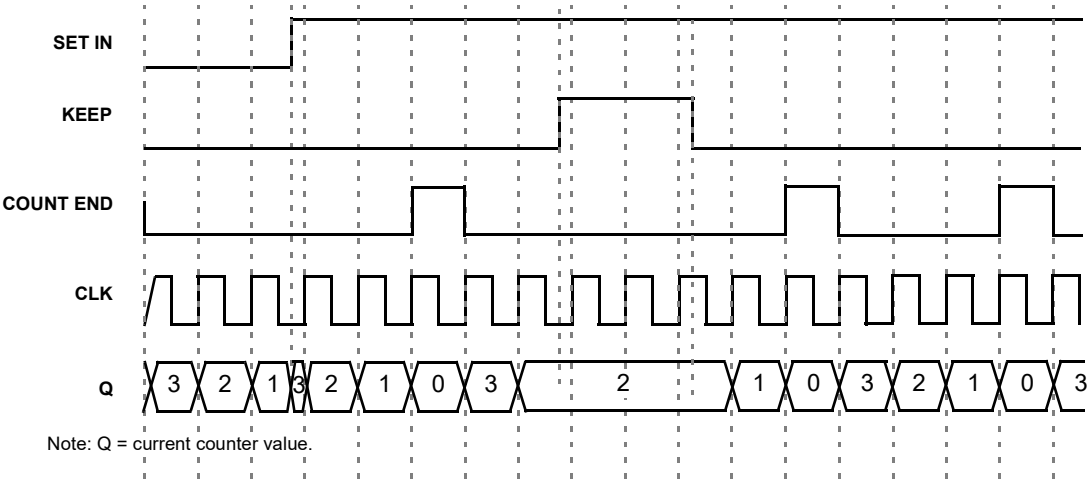
Figure 38. CNT/FSM Timing Diagram (Set Rising Edge Mode, Oscillator is Forced On, UP = 0) for Counter Data = 3
