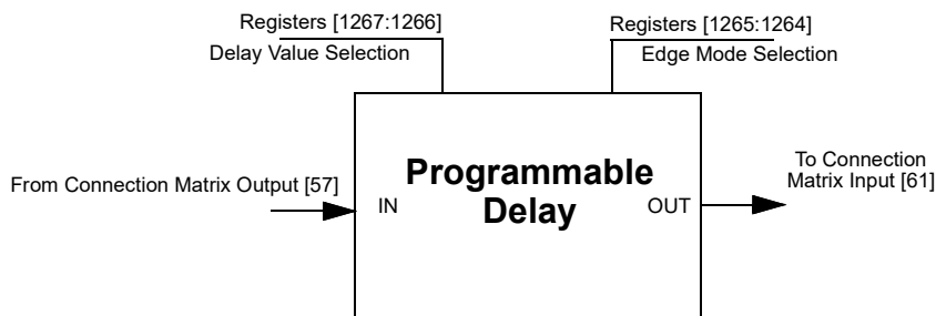
Figure 63. Programmable Delay
