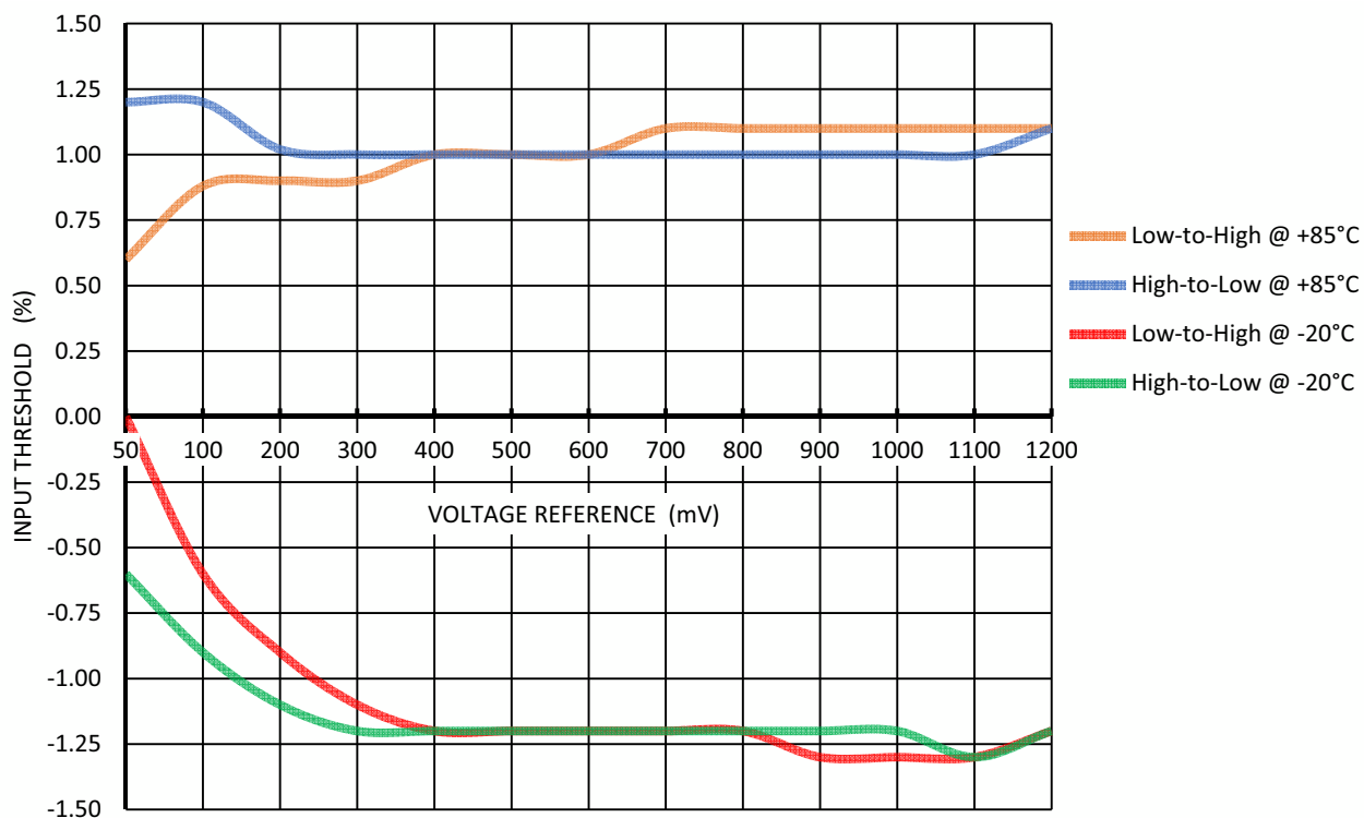
Figure 24. Input Threshold Ratio vs. Voltage Reference at V_{DD} = (1.71 - 5.5) \text{ V} , V_{hys} = 0 , Gain = 1
