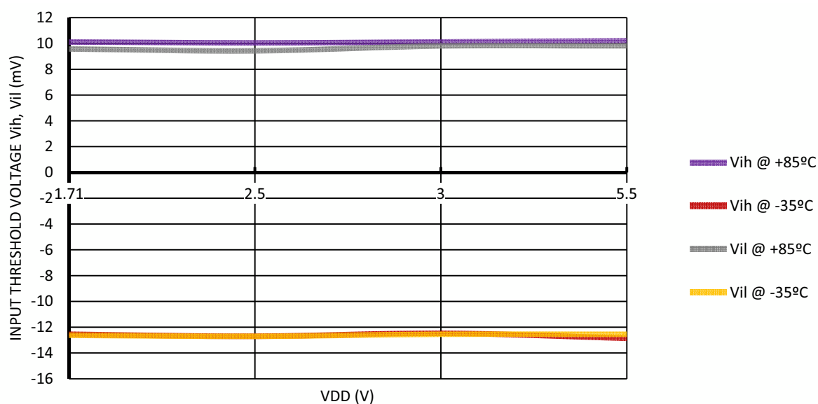
Figure 25. Input Threshold Voltage V_{ih} , V_{il} vs. V_{DD} at V_{ref} = 1000 \text{ mV} , Gain = 1
