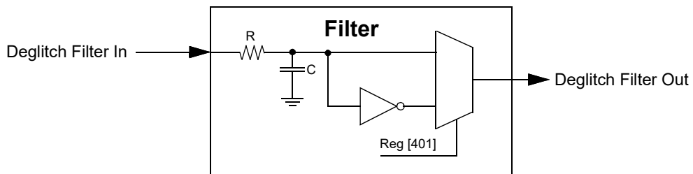
Figure 26. Deglitch Filter
