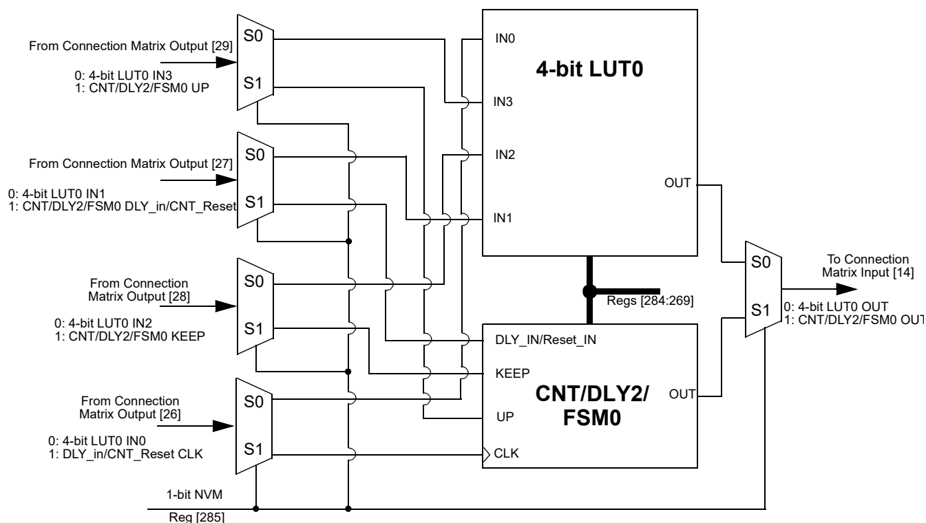
Figure 16. 4-bit LUT1 or CNT/DLY2/FSM0
