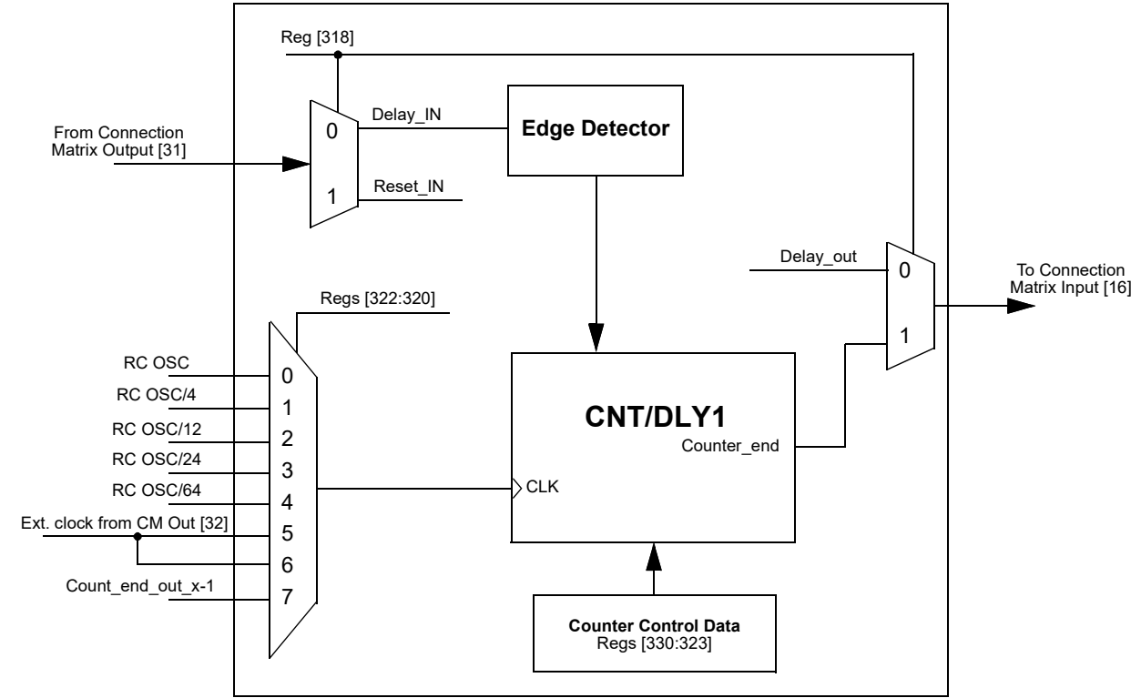
Figure 28. CNT/DLY1
