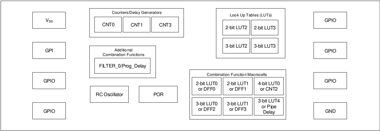
Figure 1. Block Diagram
