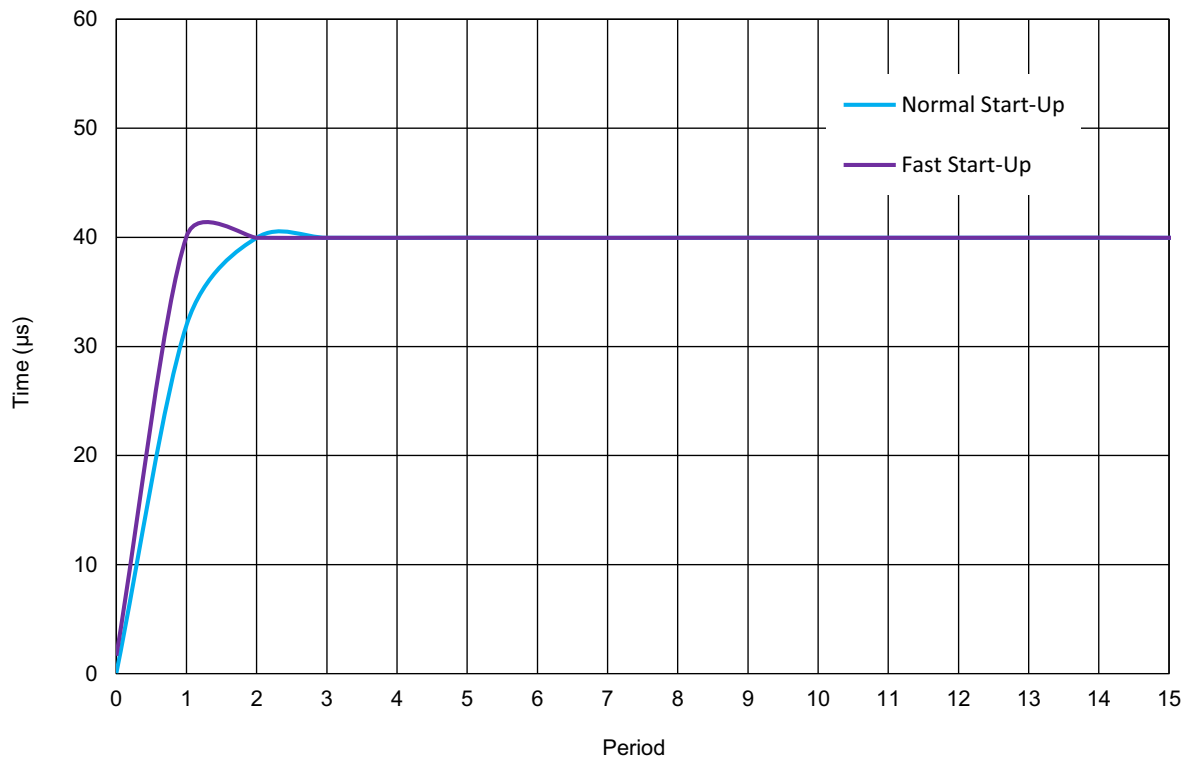
Figure 37. Oscillator Settling Time, V_{DD} = 3.3\text{ V} , T_A = 25\text{ }^{\circ}\text{C} , \text{OSC} = 25\text{ kHz}
