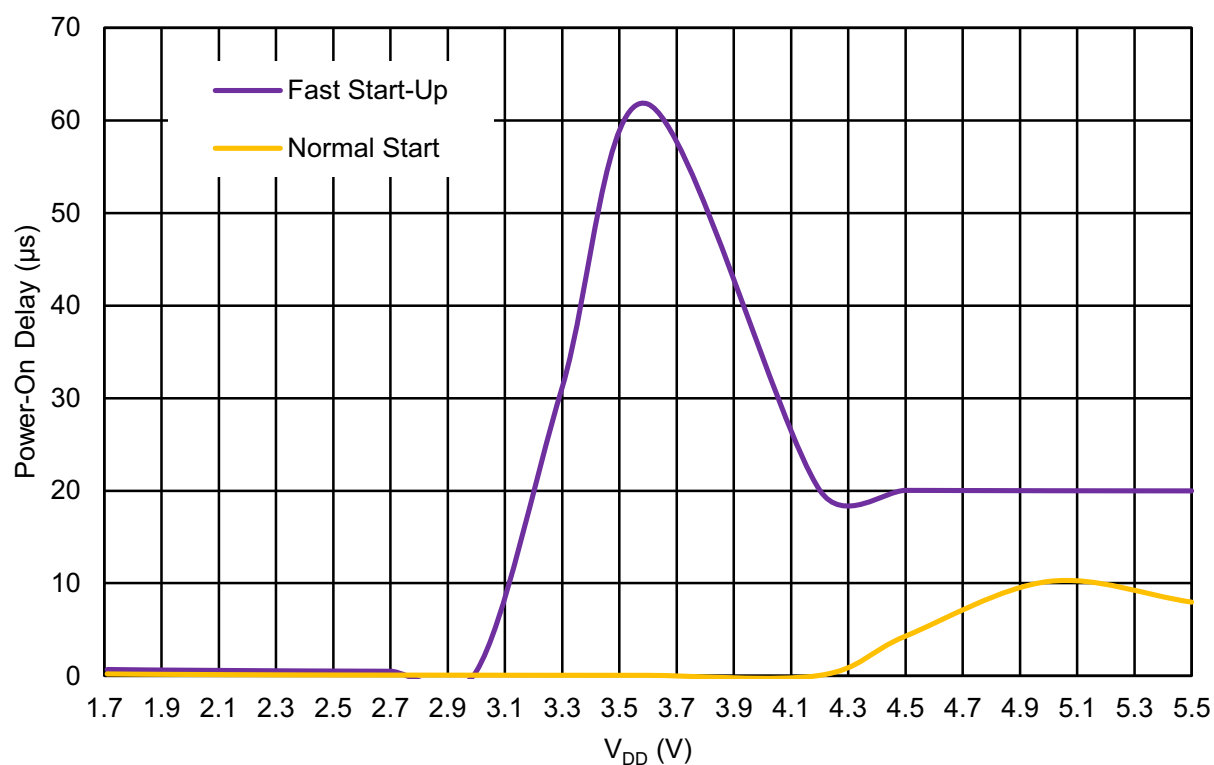
Figure 32. Oscillator Maximum Power-On Delay vs. V_{DD} at T_A = 25\text{ }^{\circ}\text{C} , OSC = 25 kHz
