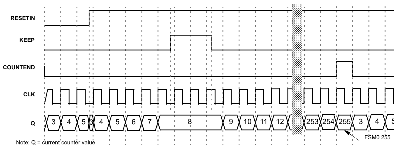
Figure 23. Timing (Set Rising Edge Mode, Oscillator is Forced On, Up = 1) for Count Data = 3
