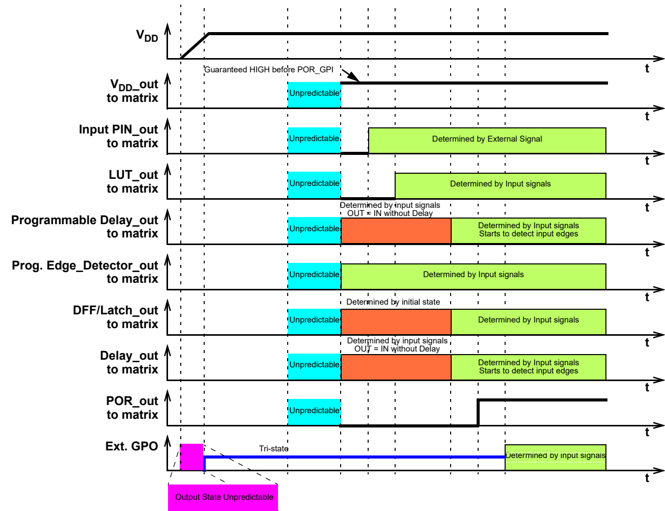
Figure 40. Internal Macrocell States during POR Sequence
