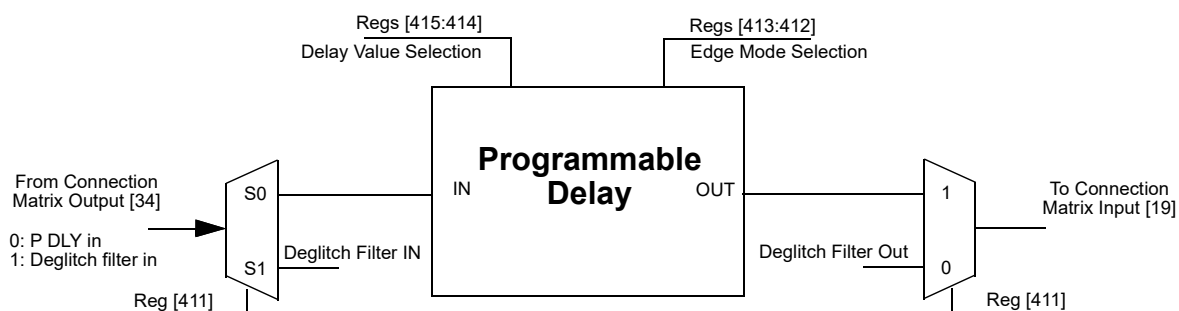
Figure 24. Programmable Delay
