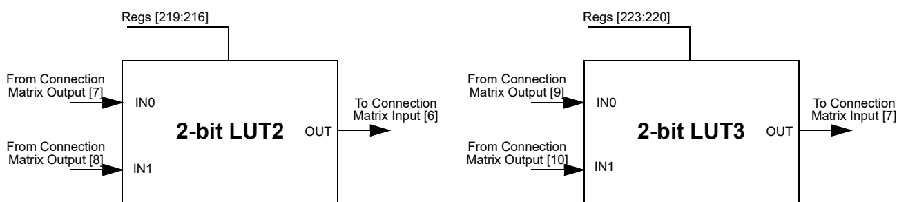
Figure 9. 2-bit LUTs
