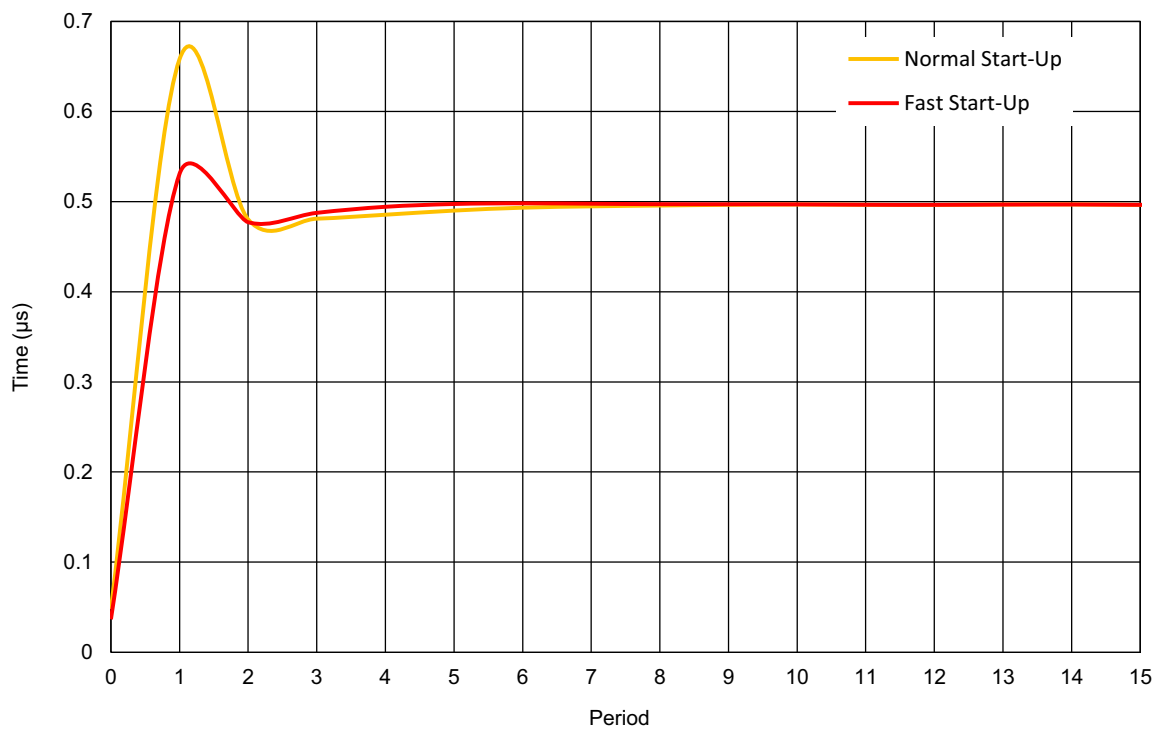
Figure 38. Oscillator Settling Time, V_{DD} = 3.3\text{ V} , T_A = 25\text{ }^{\circ}\text{C} , \text{OSC} = 2\text{ MHz}
