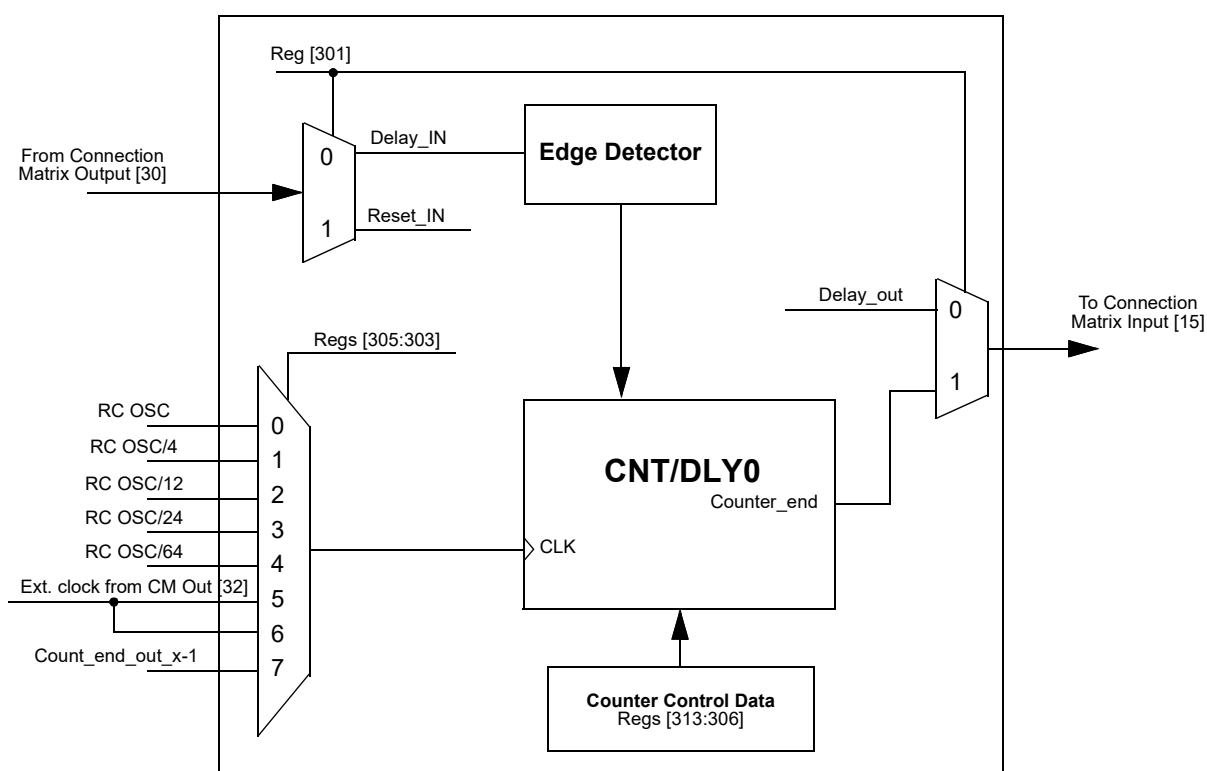
Figure 27. CNT/DLY0
