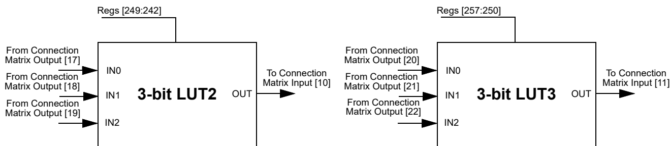
Figure 10. 3-bit LUTs
