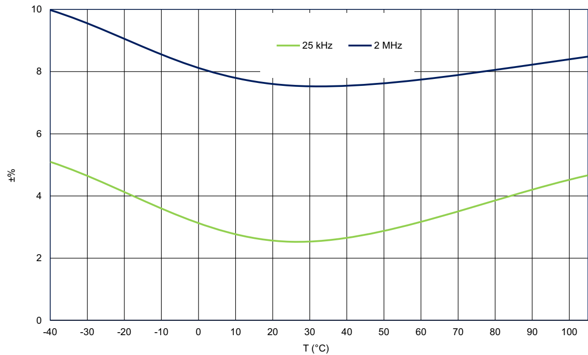
Figure 36. Oscillators Total Error vs. Temperature
