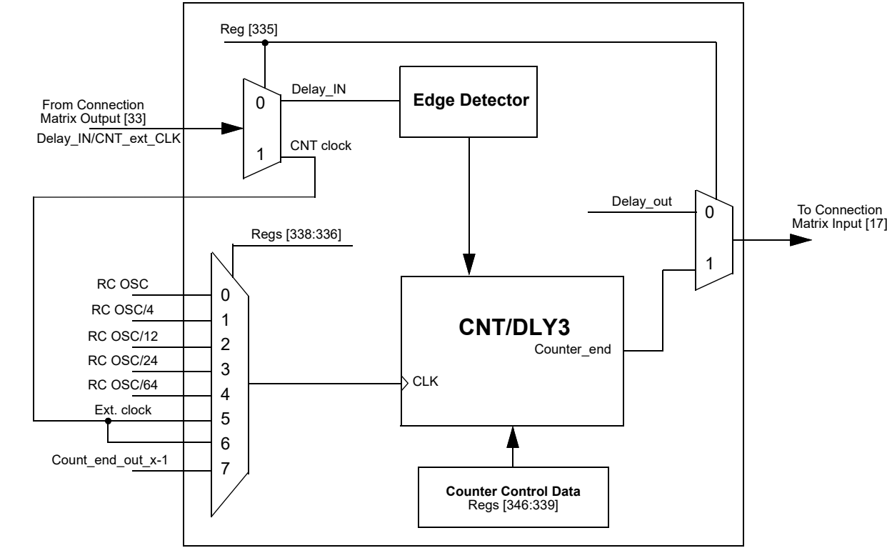
Figure 29. CNT/DLY3
