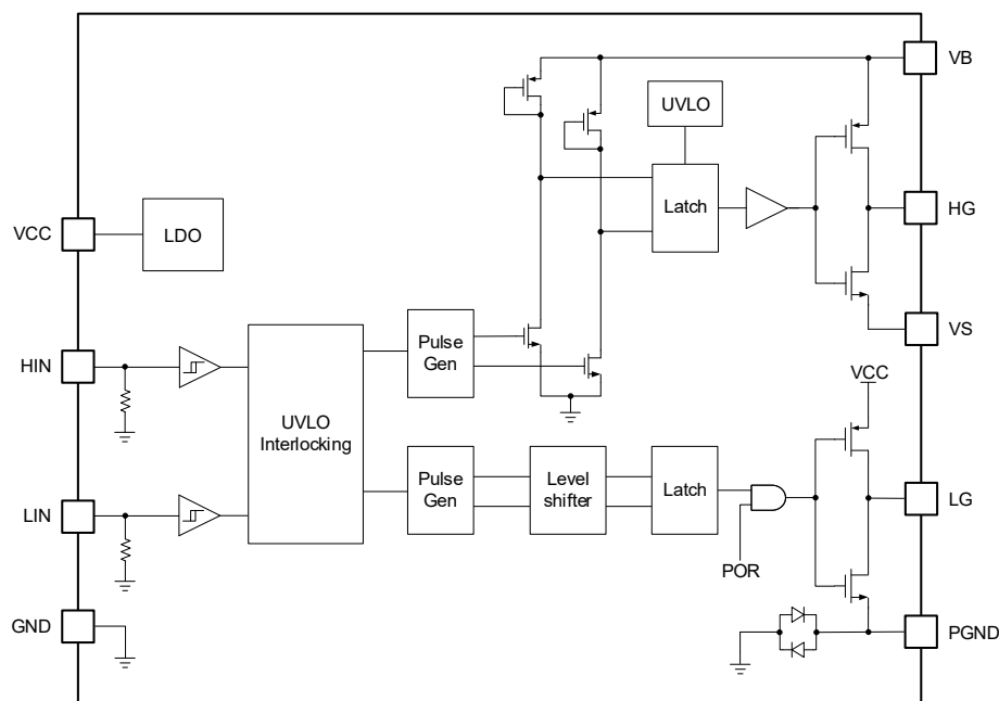
Figure 1. RRW40120 Block Diagram
