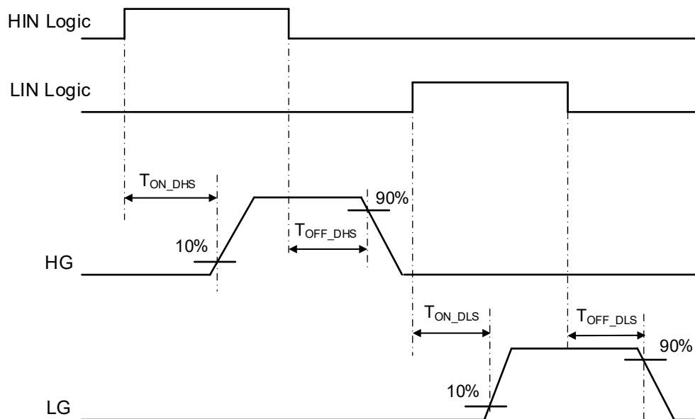
Figure 5. Input/Output Timing Relationships
