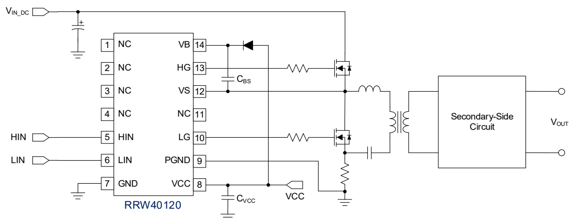
Figure 2. RRW40120 Typical Application Circuit
