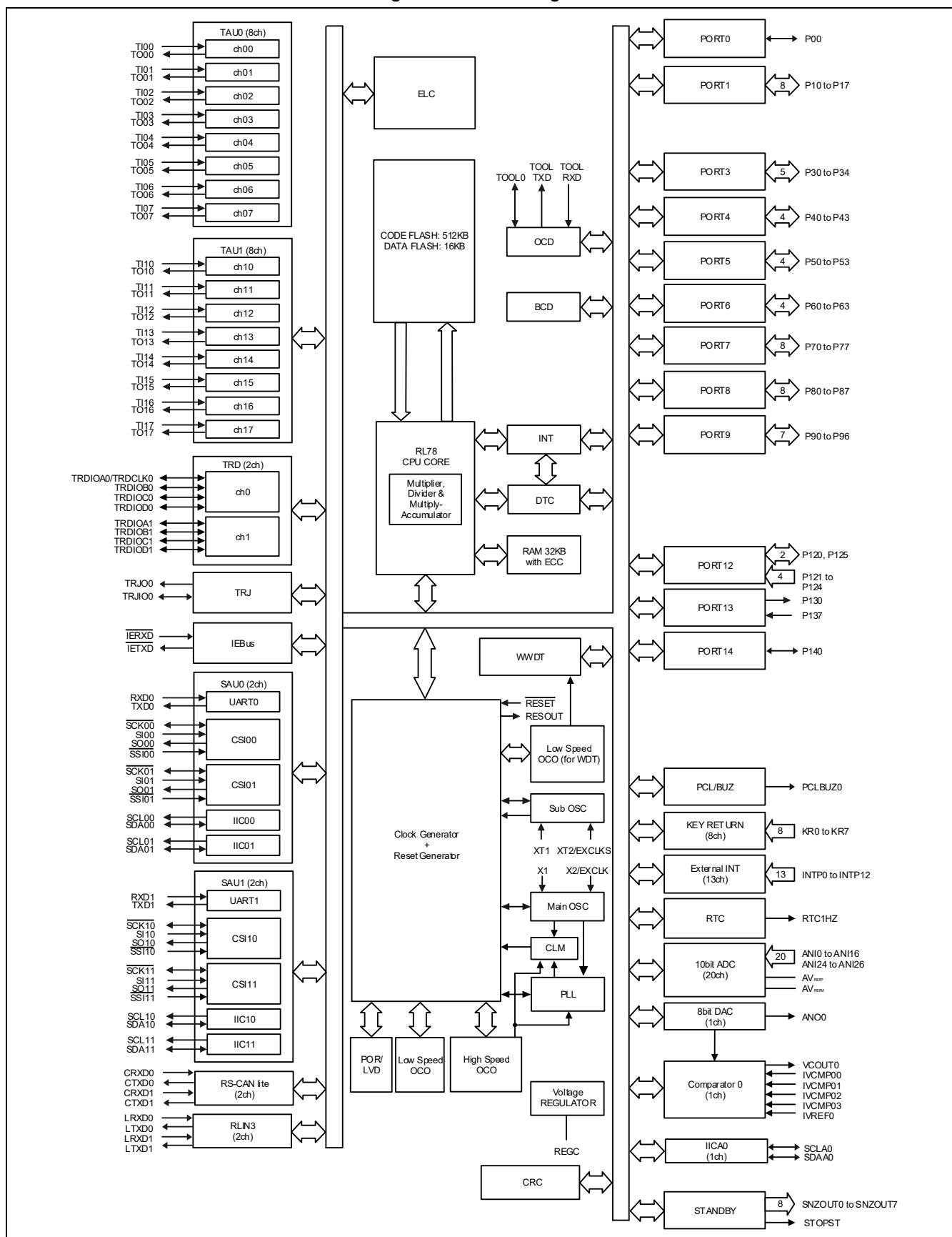
Figure 1-4. Block Diagram
