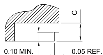
TERMINAL CROSS SECTION F-F'
