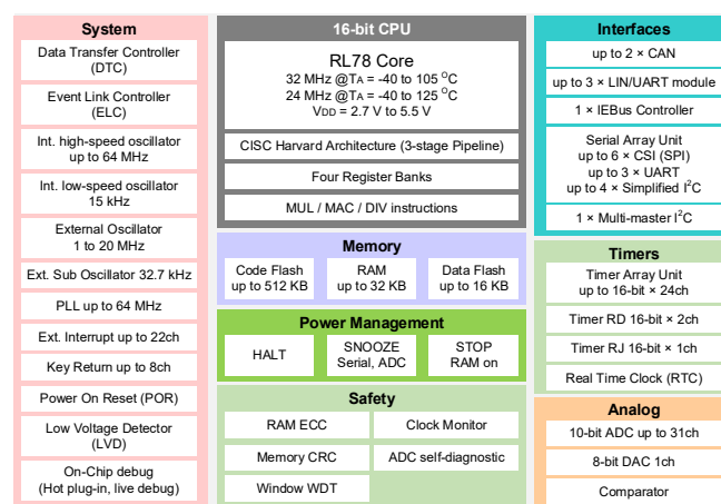
RL78/F15 Block Diagram (Outline)
