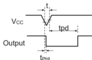
Time Chart at Momentary Voltage-Decrease
