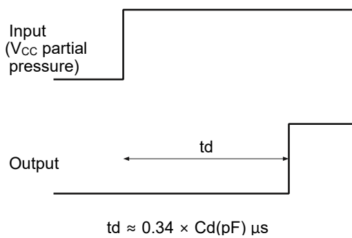
Operating Waveform
