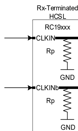
Figure 17. Receiver Termination
