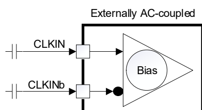
Figure 14. External AC-Coupling
