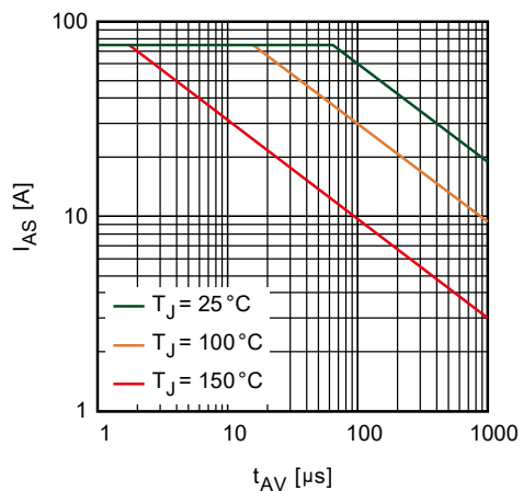
Figure 5. Avalanche Current Characteristics
