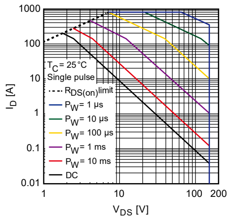
Figure 3. Forward Bias Safe Operating Area
