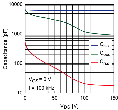
Figure 13. Capacitances vs. Drain to Source Voltage
