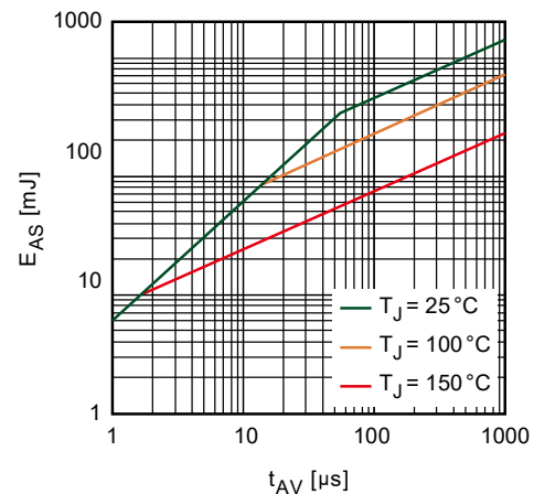
Figure 6. Avalanche Energy Characteristics
