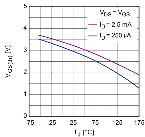
Figure 12. Gate to Source Threshold Voltage vs. Junction Temperature
