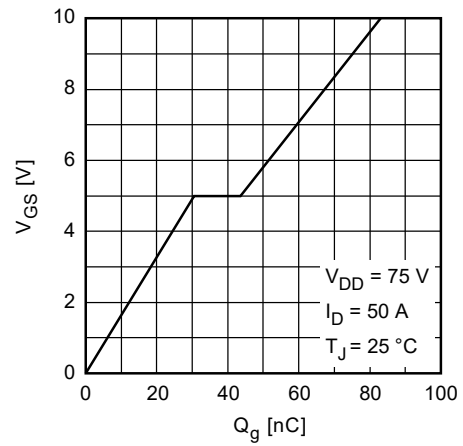
Figure 14. Dynamic Input/Output Characteristics
