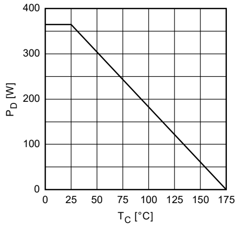
Figure 1. Power Dissipation vs. Case Temperature
