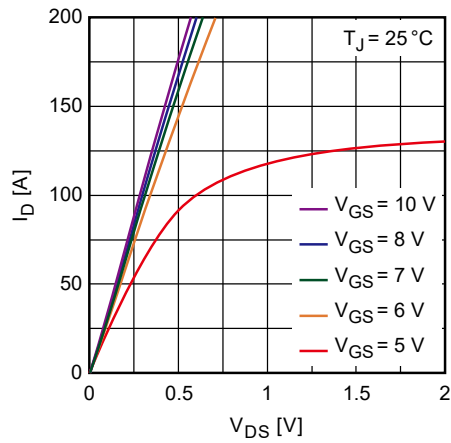
Figure 7. Typical Output Characteristics
