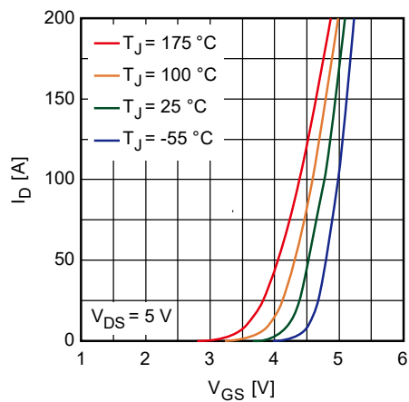
Figure 11. Typical Transfer Characteristics
