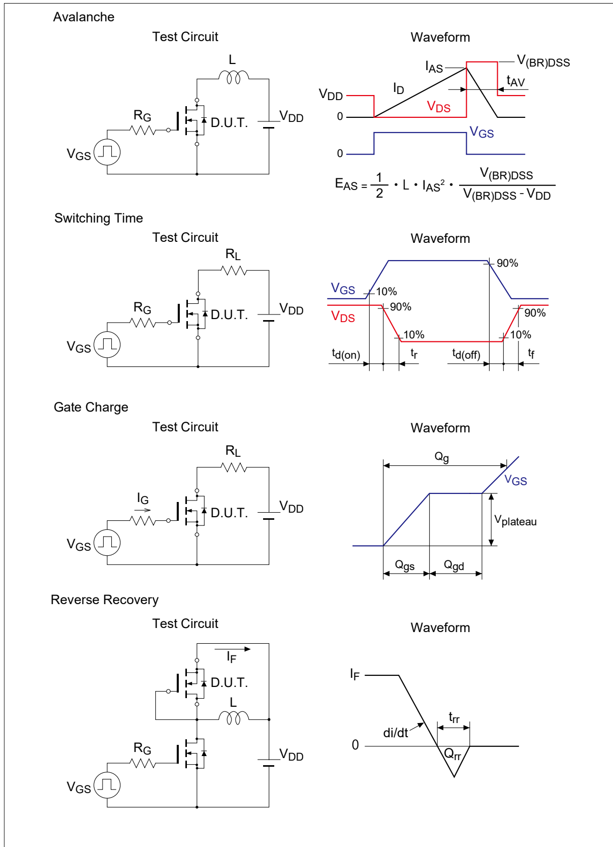
Figure 17. Test Circuits and waveforms
