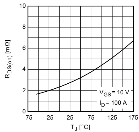
Figure 10. Drain to Source On-state Resistance vs. Junction Temperature
