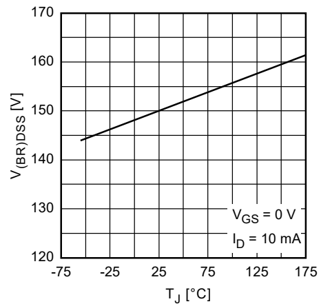
Figure 16. Drain to Source Breakdown Voltage vs. Junction Temperature
