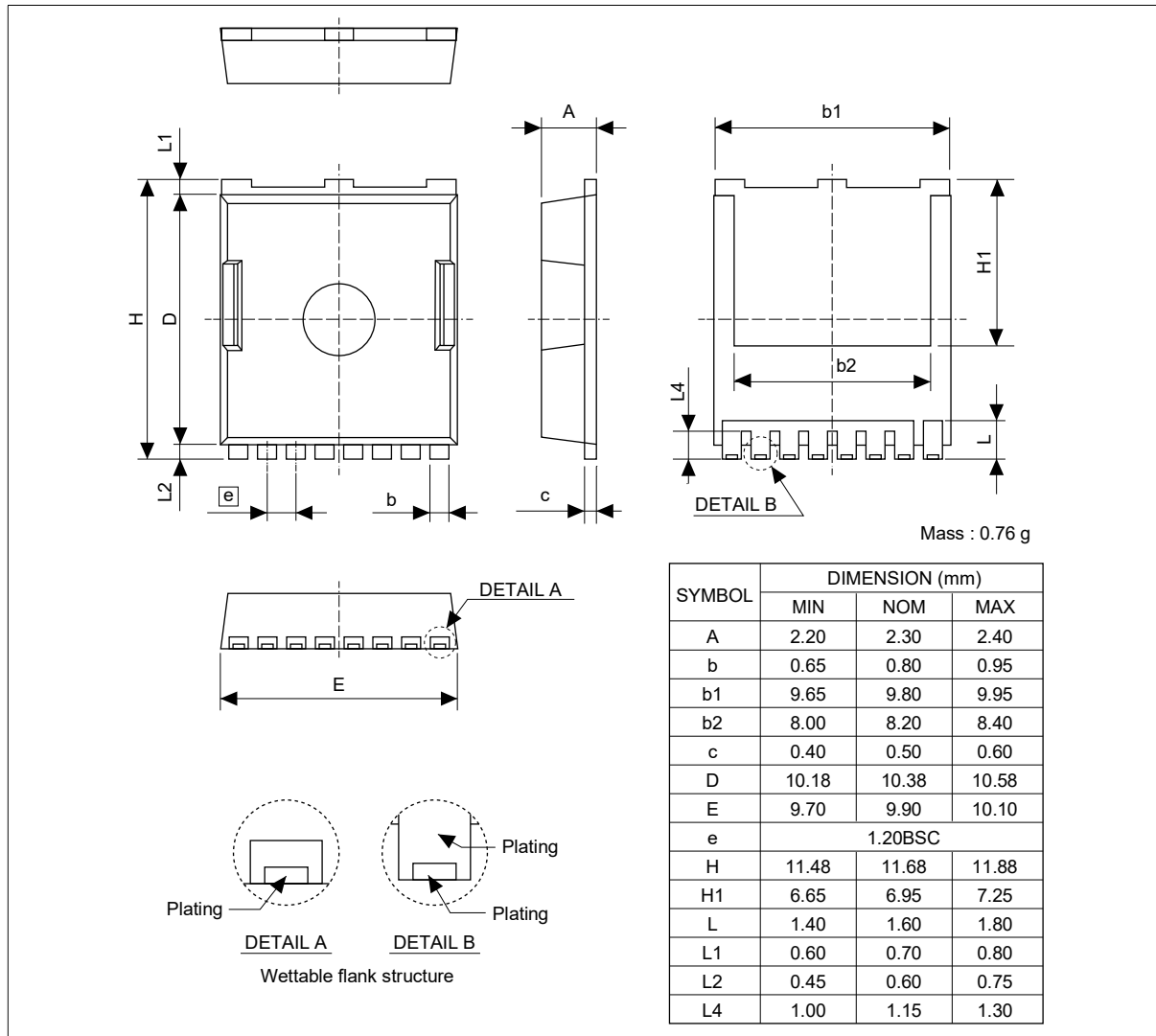
Figure 18. Package Outline – TOLL
