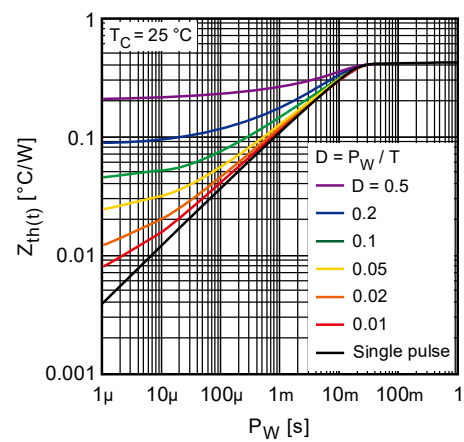
Figure 4. Transient Thermal Impedance vs. Pulse Width
