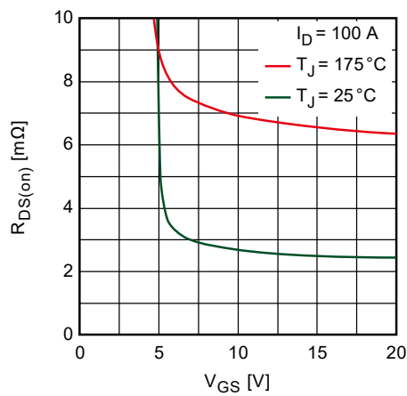
Figure 9. Drain to Source On-state Resistance vs. Gate to Source Voltage
