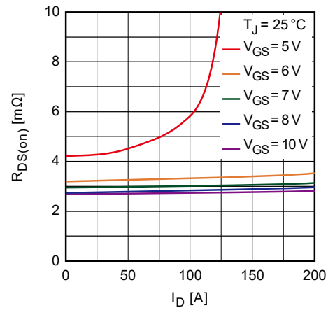
Figure 8. Drain to Source On-state Resistance vs. Drain Current
