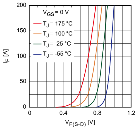
Figure 15. Source to Drain Diode Forward Voltage
