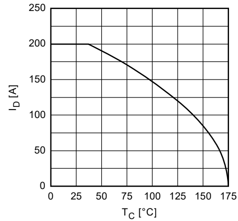
Figure 2. Drain Current vs. Case Temperature
