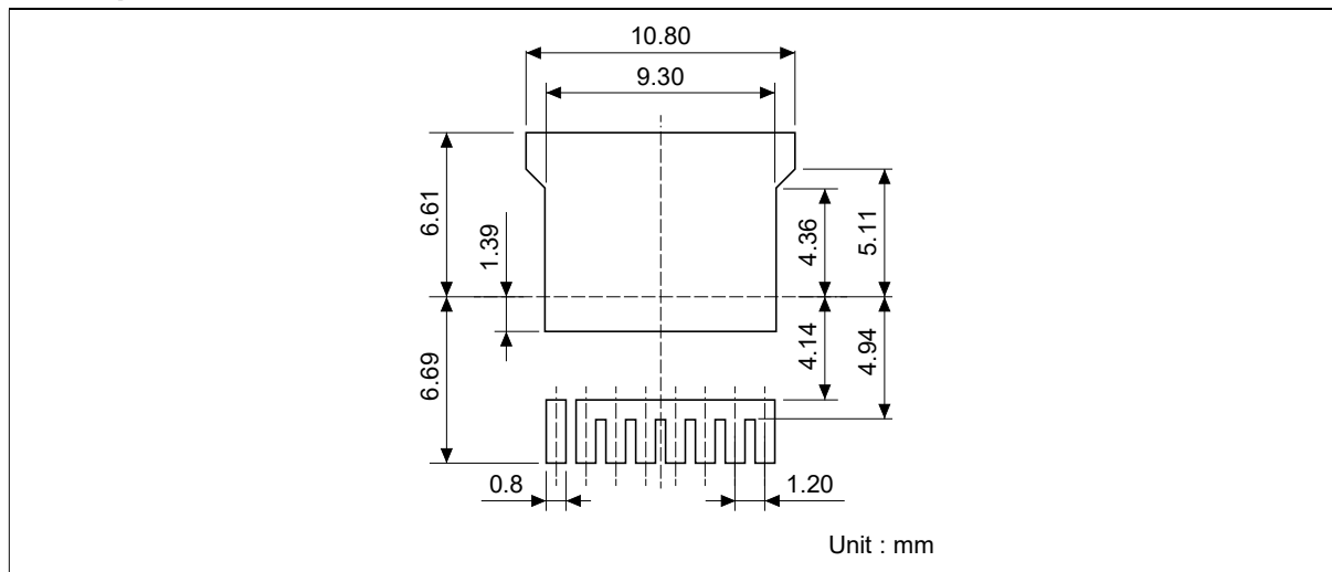
Figure 19. Mount Pad Information
