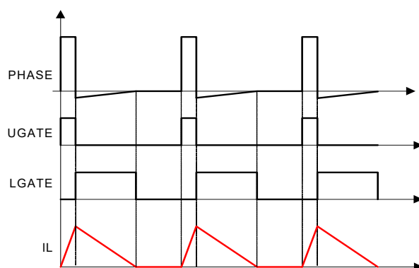
Figure 46. Diode Emulation
