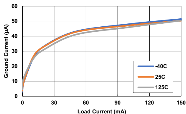
Figure 4. Ground Current vs Load
