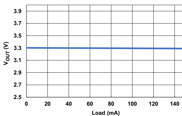
Figure 6. Output Voltage vs Load
