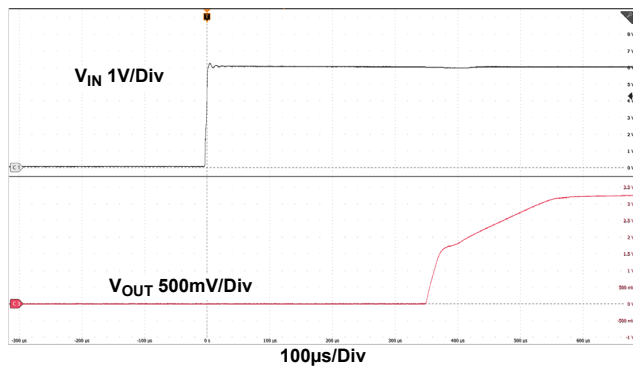
Figure 10. Startup Waveform ( I_{\text{OUT}} = 10\text{mA} )
