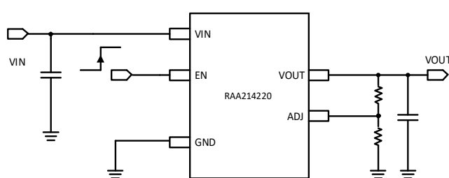
Figure 2. RAA214220 Typical Application (2)
