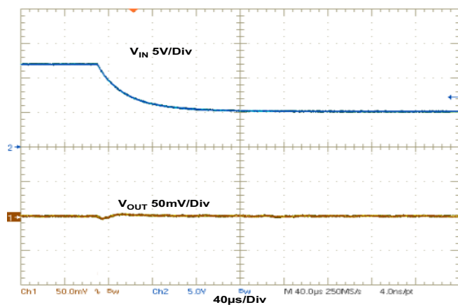
Figure 19. Line Transient (12V to 5V, V_{OUT} = 3.3V , I_{OUT} = 1mA )
