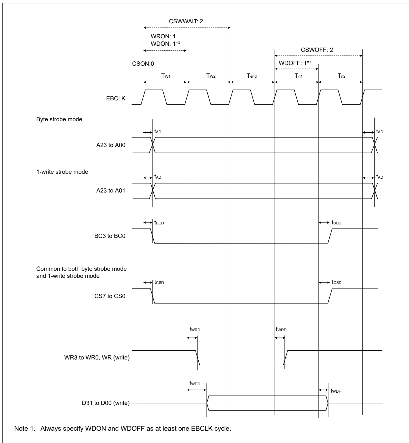
Figure 2.31 External bus timing for normal write cycle with bus clock synchronized
