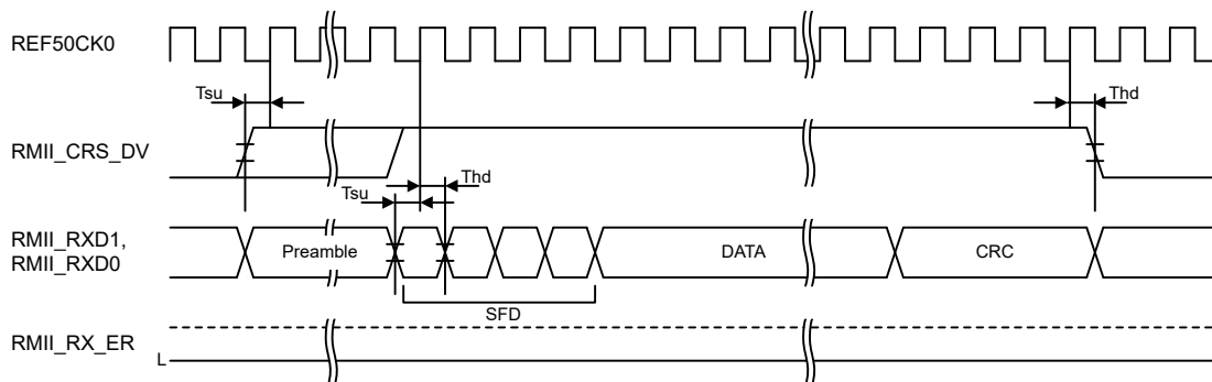
Figure 2.82 RMII reception timing in normal operation
