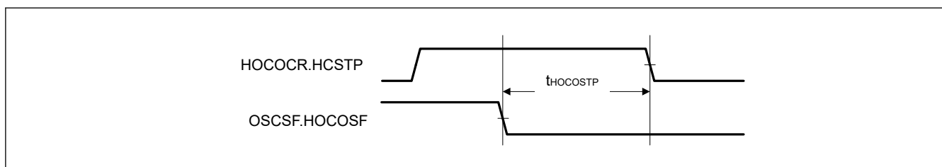
Figure 2.21 HOCO stop width time
