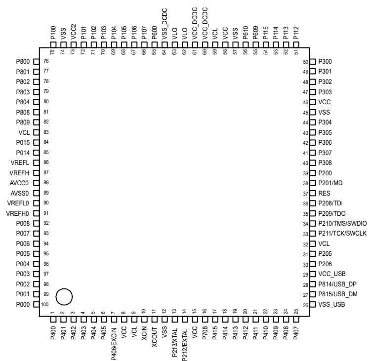
Figure 1.6 Pin assignment for LQFP 100-pin
