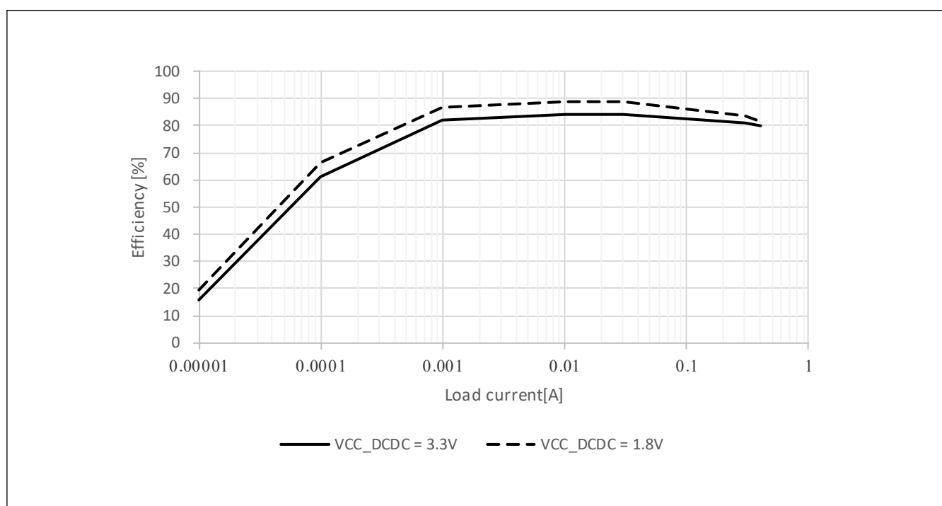
Figure 2.11 Typical DCDC efficiency (%) vs load current (A) in Low-speed mode and Software Standby mode, T_j = 25^\circ\text{C}
