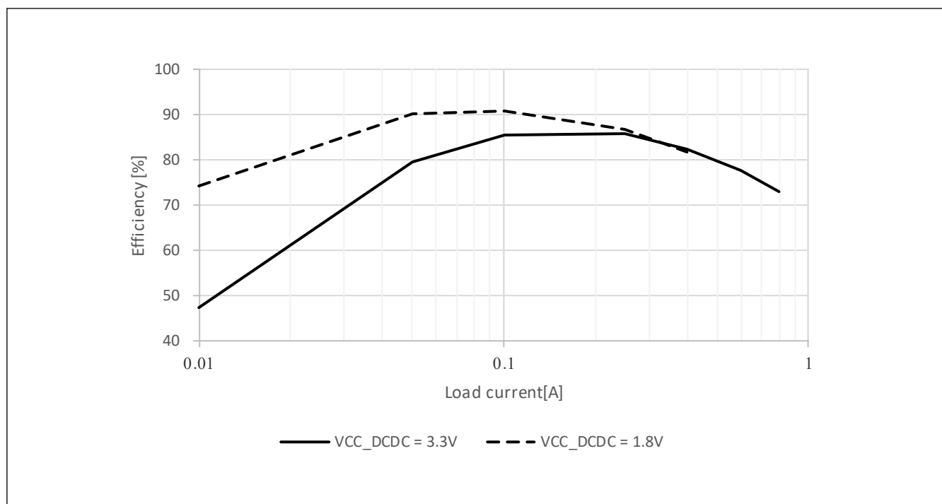
Figure 2.10 Typical DCDC efficiency (%) vs load current (A) in High-speed mode , T_j = 125^\circ\text{C}
