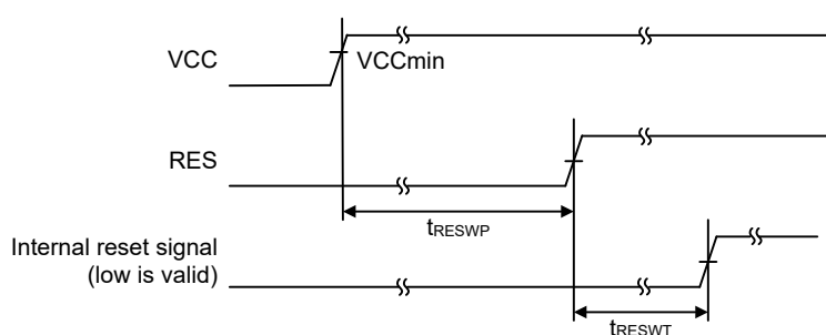
Figure 2.22 RES pin input timing under the condition that VCC exceeds V_{POR} voltage threshold
