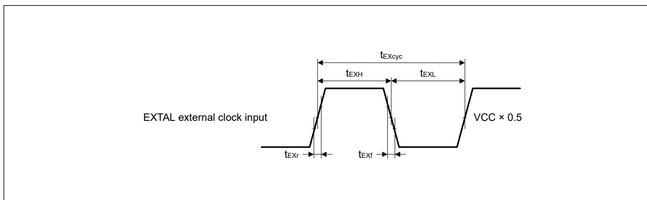
Figure 2.16 EXTERNAL external clock input timing
