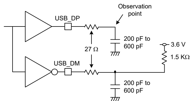
Figure 2.92 Test circuit in low-speed mode
