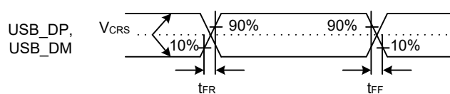
Figure 2.93 USB_DP and USB_DM output timing in full-speed mode
