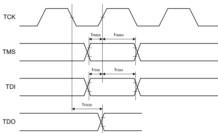
Figure 2.102 Boundary scan input/output timing (1)
