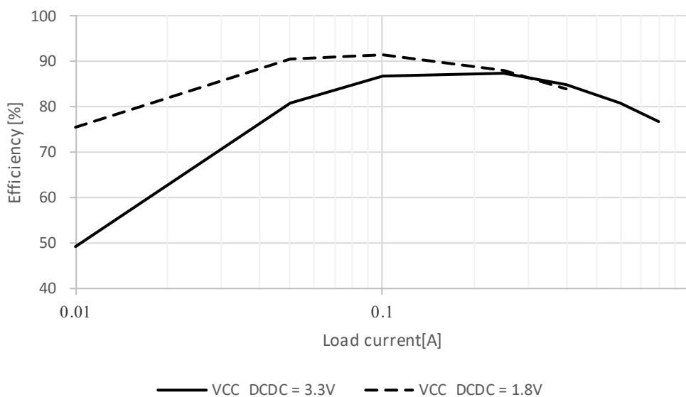
Figure 2.9 Typical DCDC efficiency (%) vs load current (A) in High-speed mode , T j = 25°C
