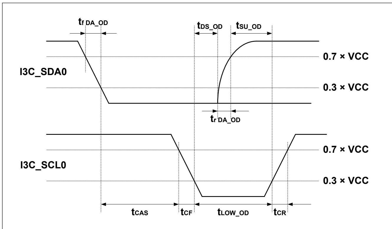
Figure 2.70 I3C START condition Timing
