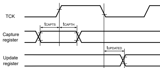
Figure 2.103 Boundary scan input/output timing (2)
