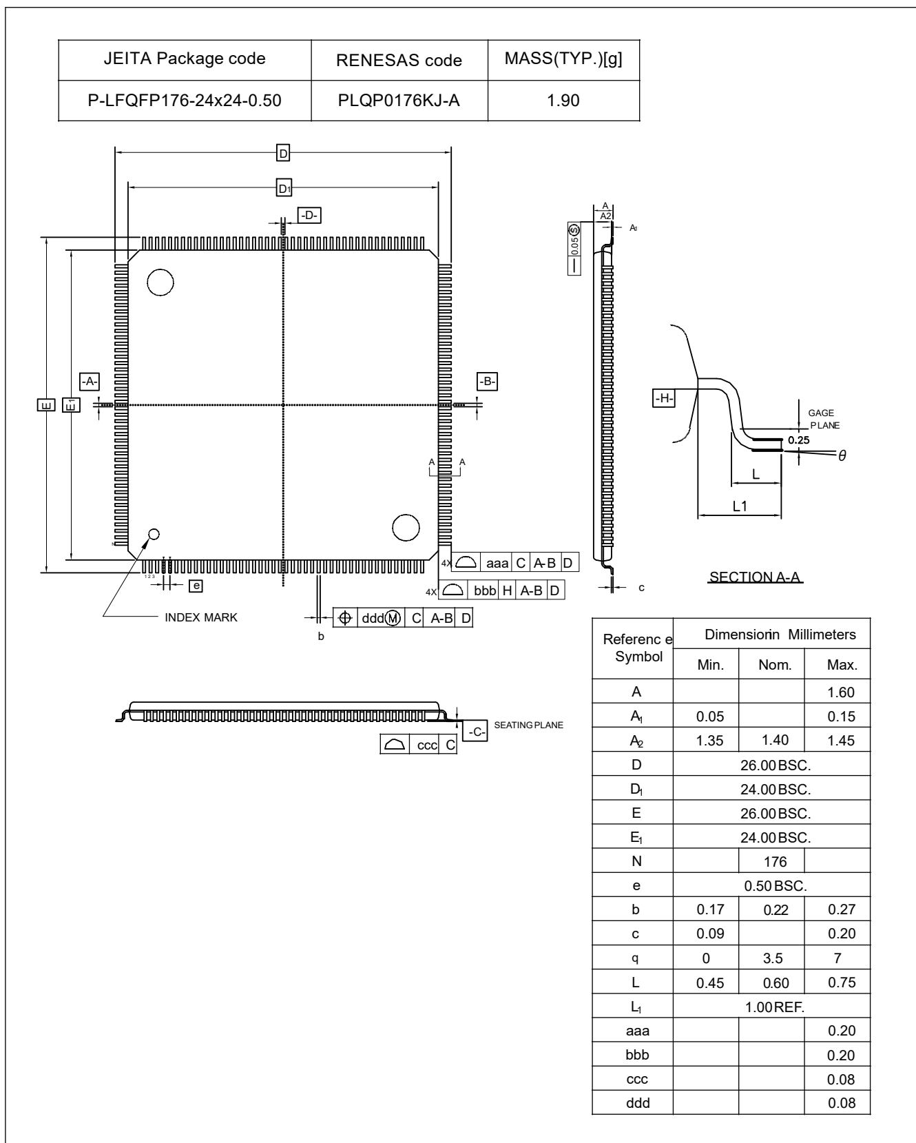
Figure A2.1 LQFP 176-pin
