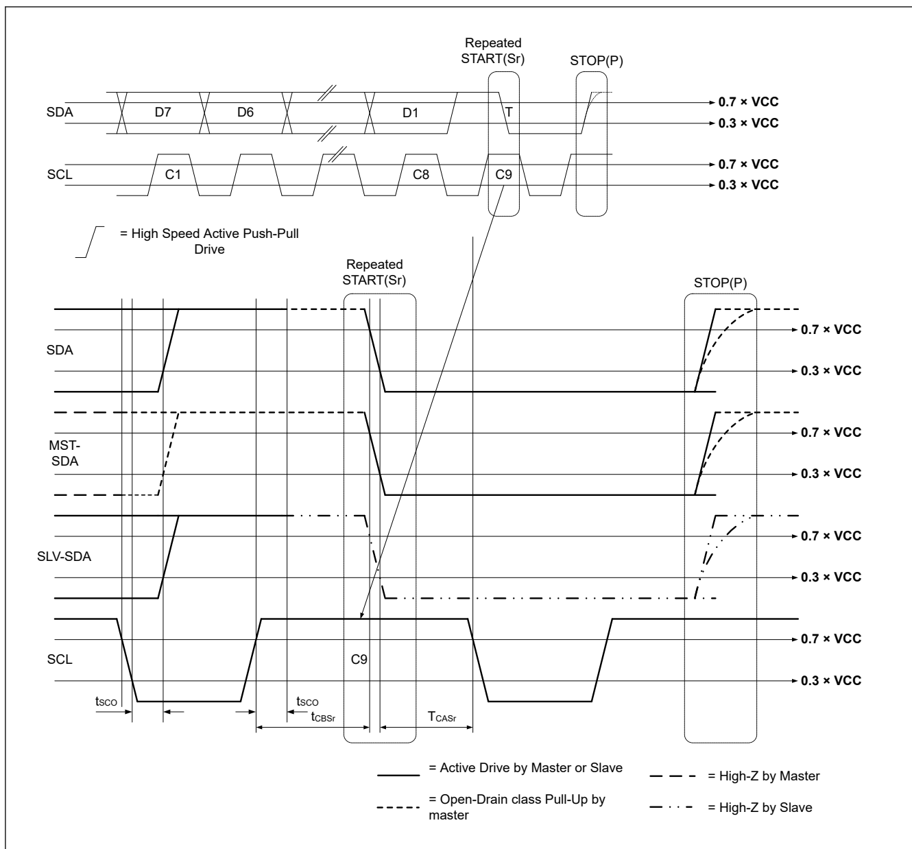
Figure 2.82 T-Bit When Master Ends Read with Repeated START and STOP
