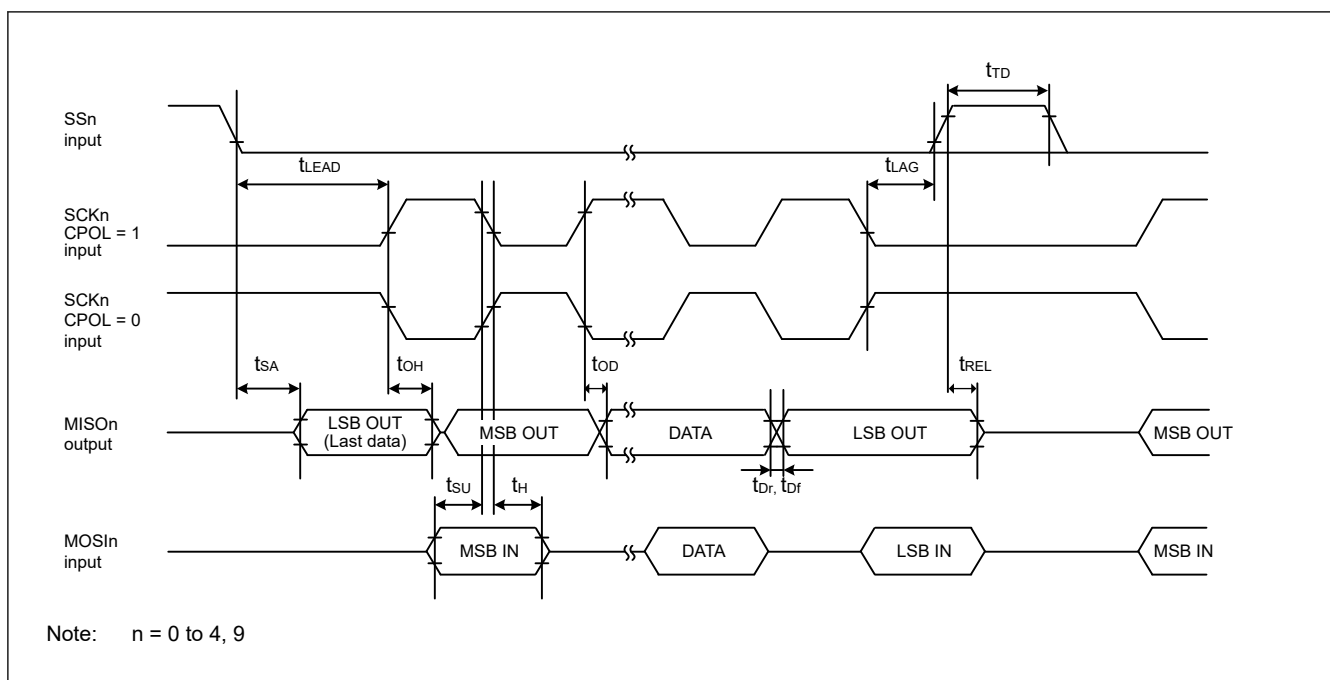
Figure 2.56 SCI simple SPI mode timing for slave when CPHA = 1
