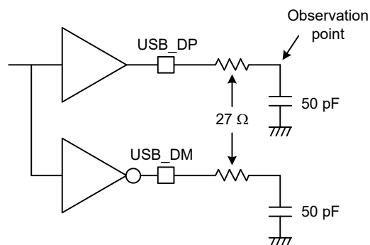
Figure 2.107 Test circuit in full-speed mode
