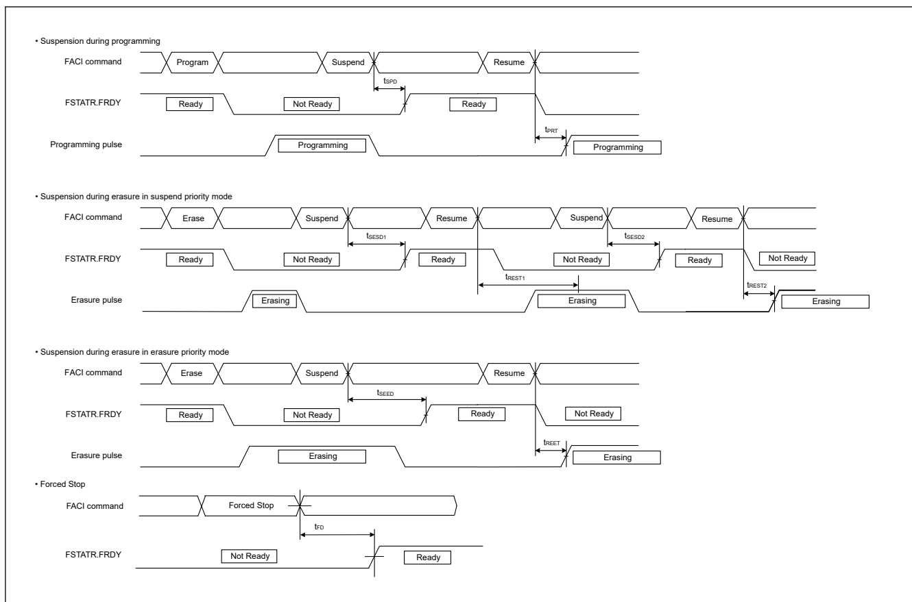
Figure 2.123 Suspension and forced stop timing for flash memory programming and erasure
