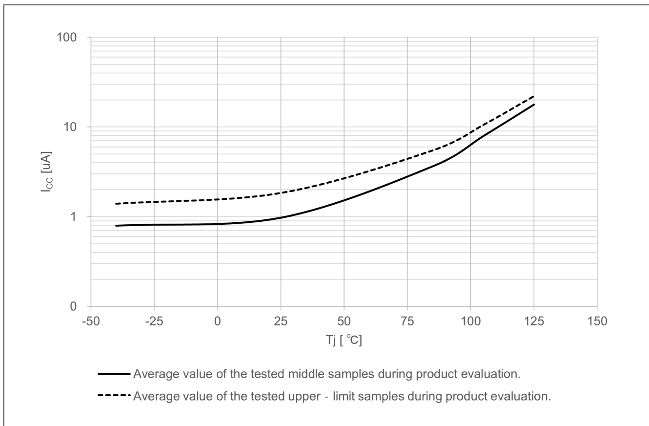
Figure 2.7 Temperature dependency in Deep Software Standby mode 3 (reference data)
