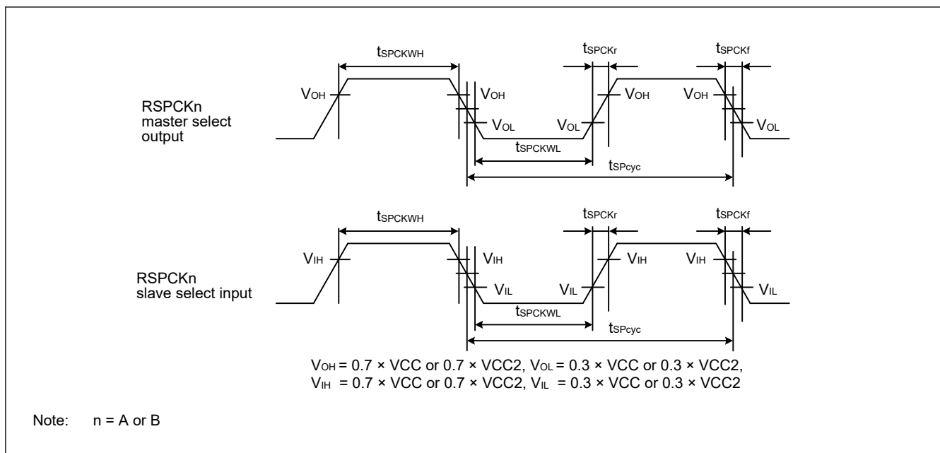
Figure 2.58 SPI clock timing
