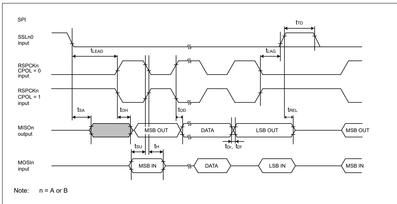
Figure 2.63 SPI timing for Motorola SPI slave when CPHA = 1
