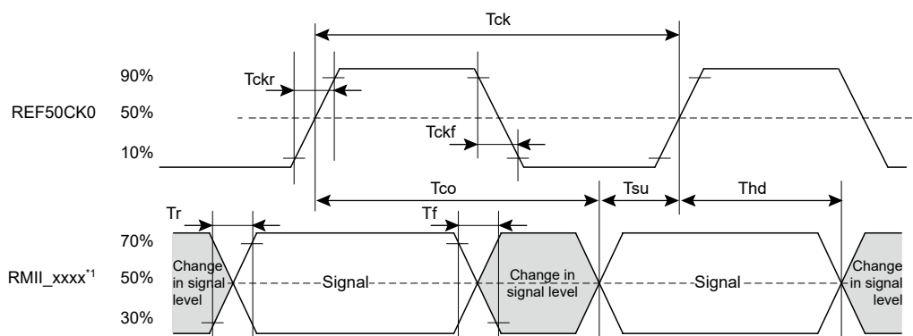
Figure 2.91 REF50CK0 and RMII signal timing
