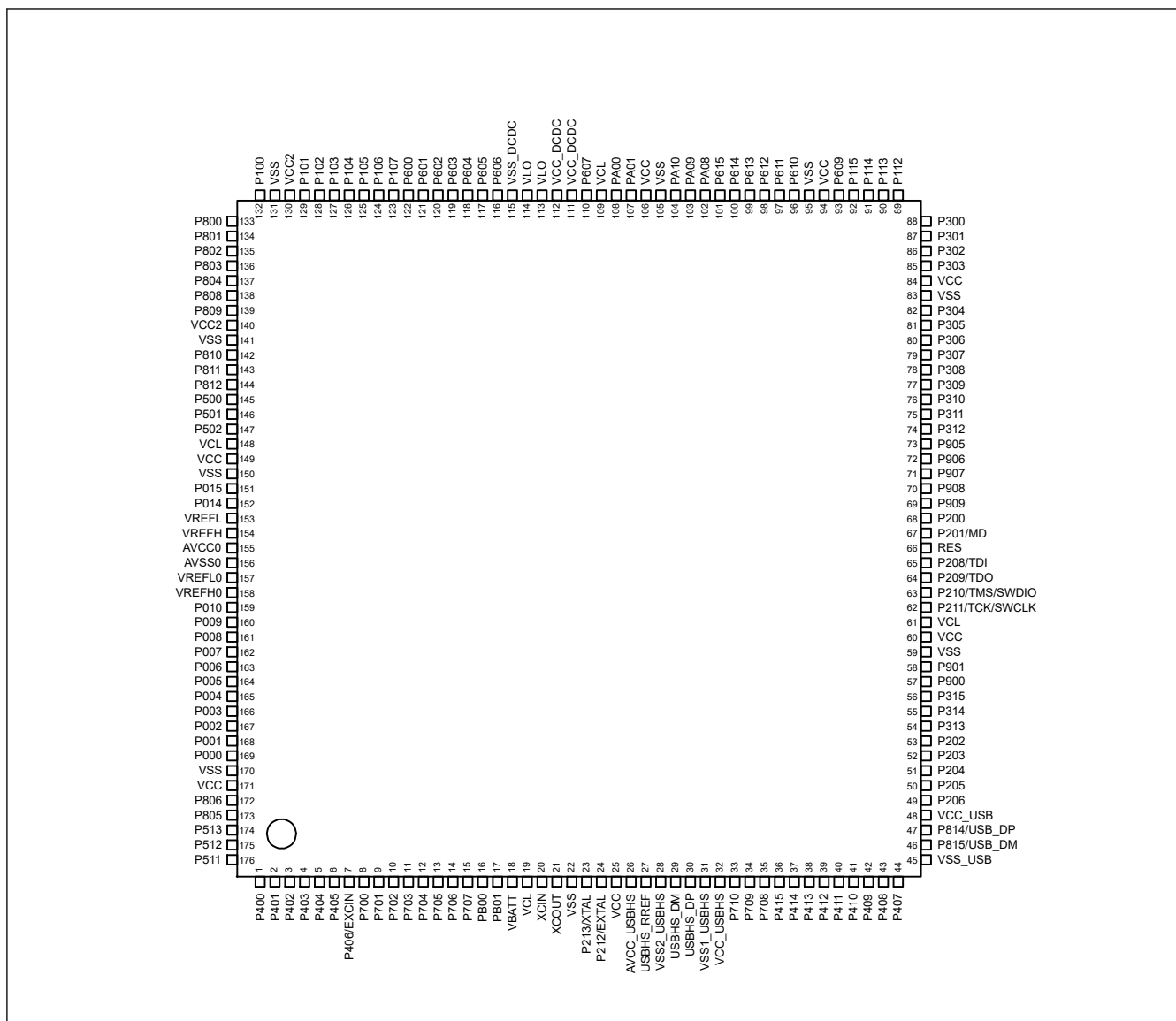
Figure 1.5 Pin assignment for 176-pin
