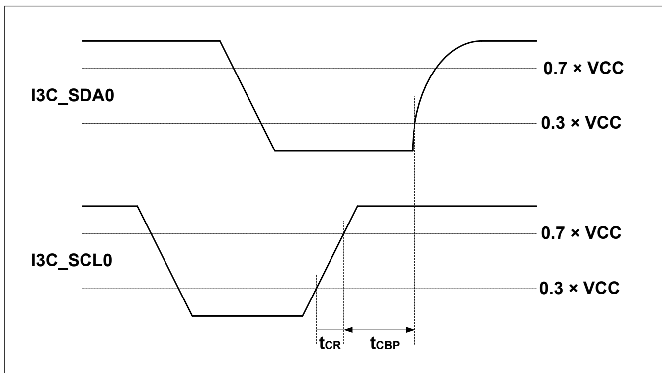
Figure 2.77 I3C STOP condition Timing
