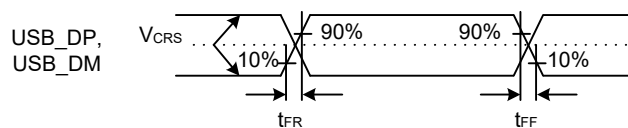
Figure 2.106 USB_DP and USB_DM output timing in full-speed mode
