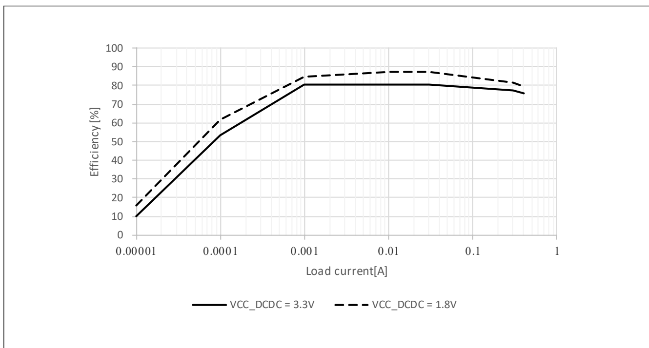
Figure 2.12 Typical DCDC efficiency (%) vs load current (A) in Low-speed mode and Software Standby mode, T_j = 125^\circ\text{C}
