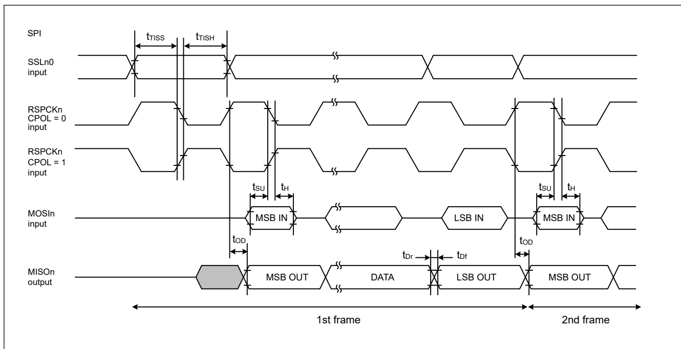
Figure 2.65 SPI timing for TI SSP slave when transmit with no delay between frames
