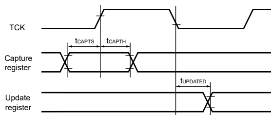
Figure 2.126 Boundary scan input/output timing (2)
