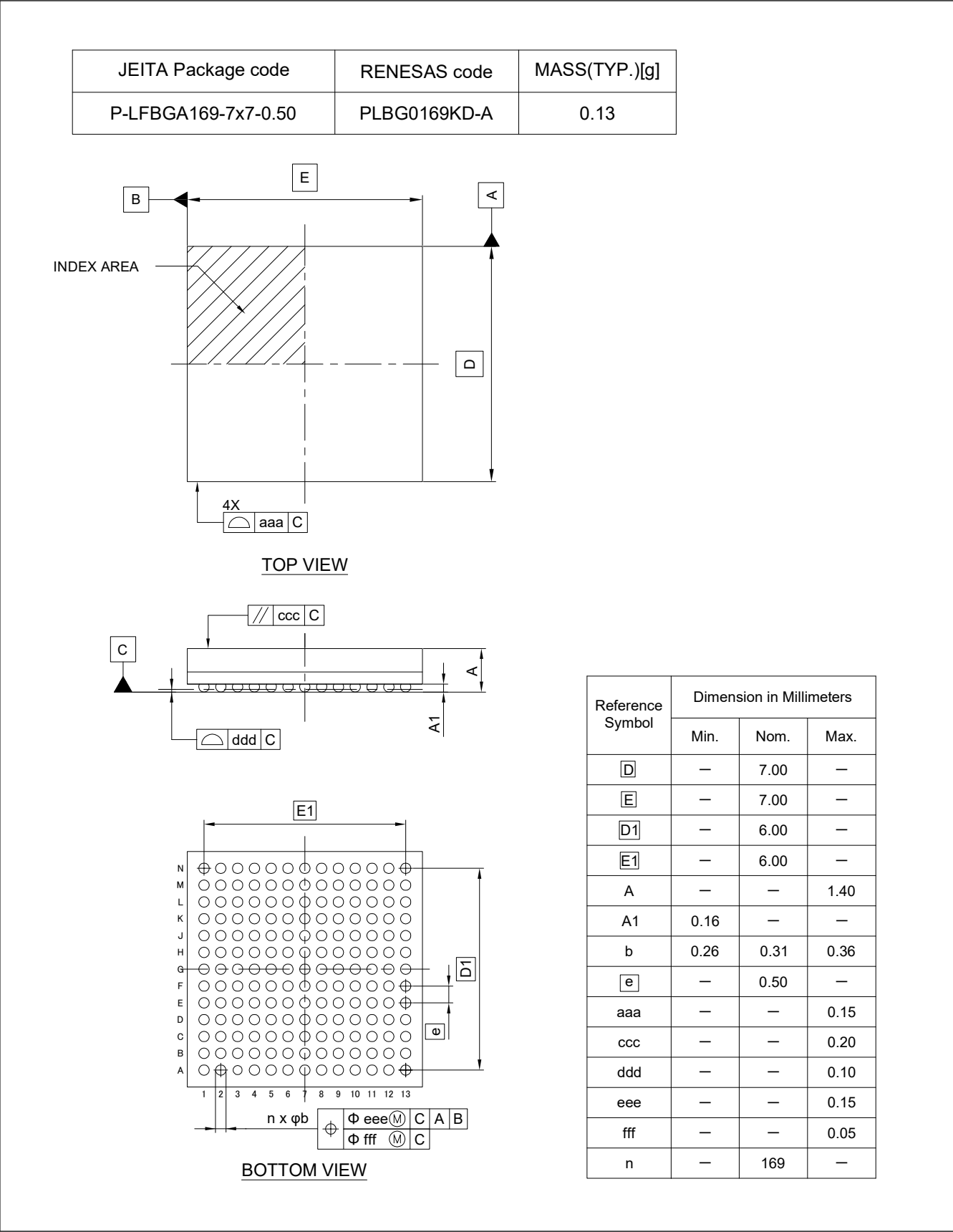
Figure A2.5 BGA 169-pin
