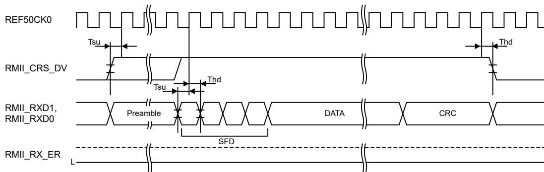
Figure 2.93 RMII reception timing in normal operation
