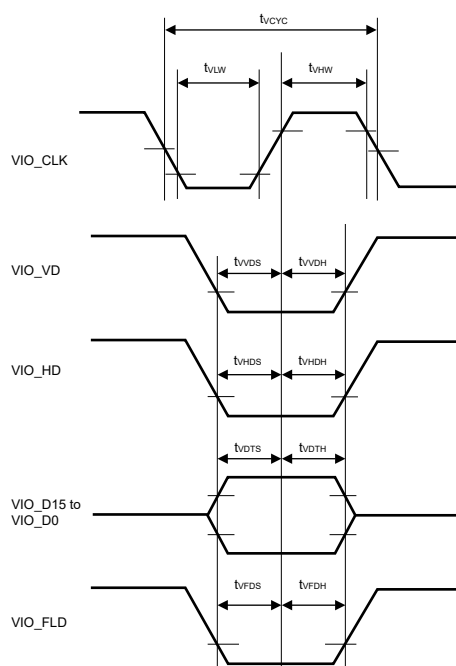
Figure 2.101 Capture Engine Unit Module Signal Timing of data capturing on the rising edge of VIO_CLK
