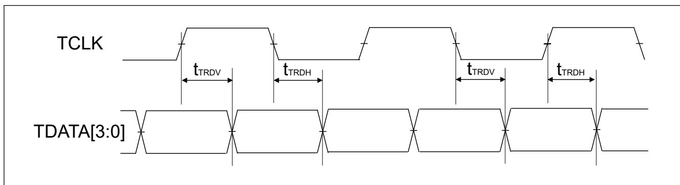
Figure 2.133 ETM output timing
