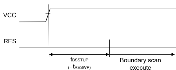
Figure 2.130 Boundary scan circuit startup timing
