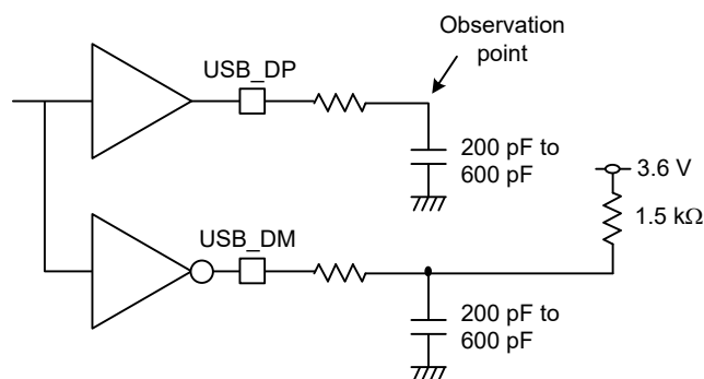
Figure 2.112 Test circuit in low-speed mode
