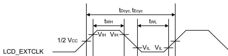
Figure 2.103 LCD_EXTCLK clock timing
