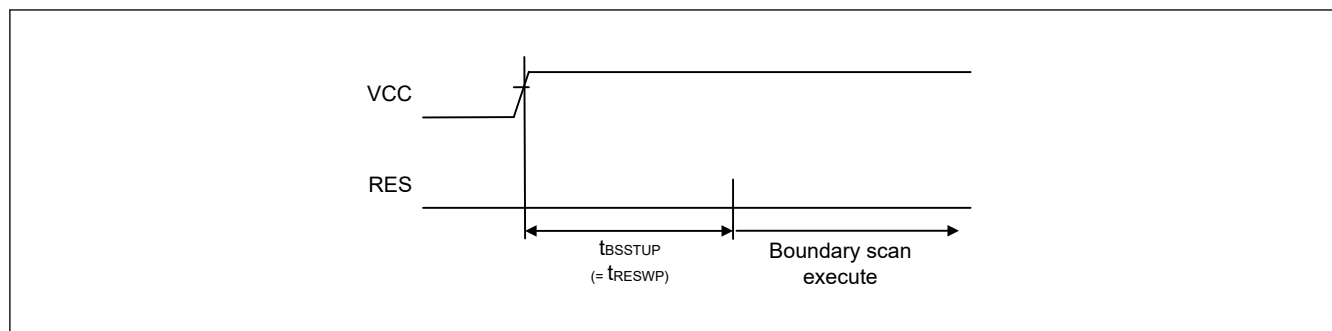
Figure 2.66 Boundary scan circuit startup timing
