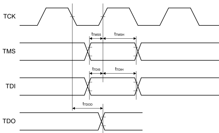
Figure 2.65 Boundary scan input/output timing
