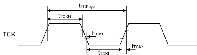
Figure 2.64 Boundary scan TCK timing
