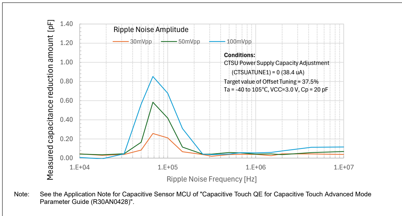
Figure 2.62 Measured capacitance reduction amount
