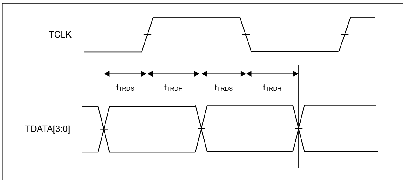
Figure 2.72 ETM output timing
