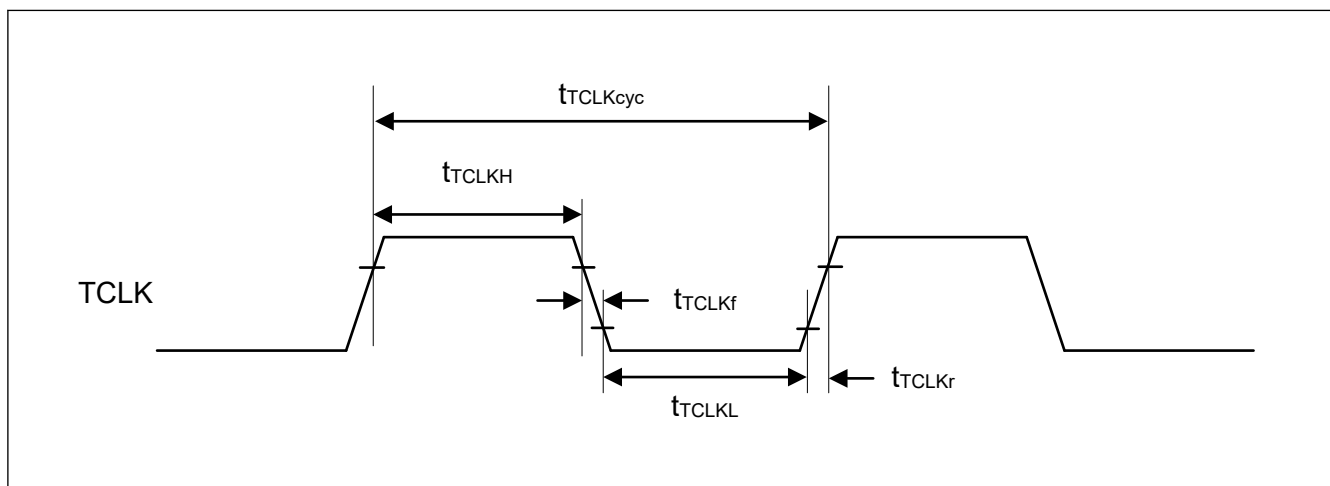
Figure 2.71 ETM TCLK timing
