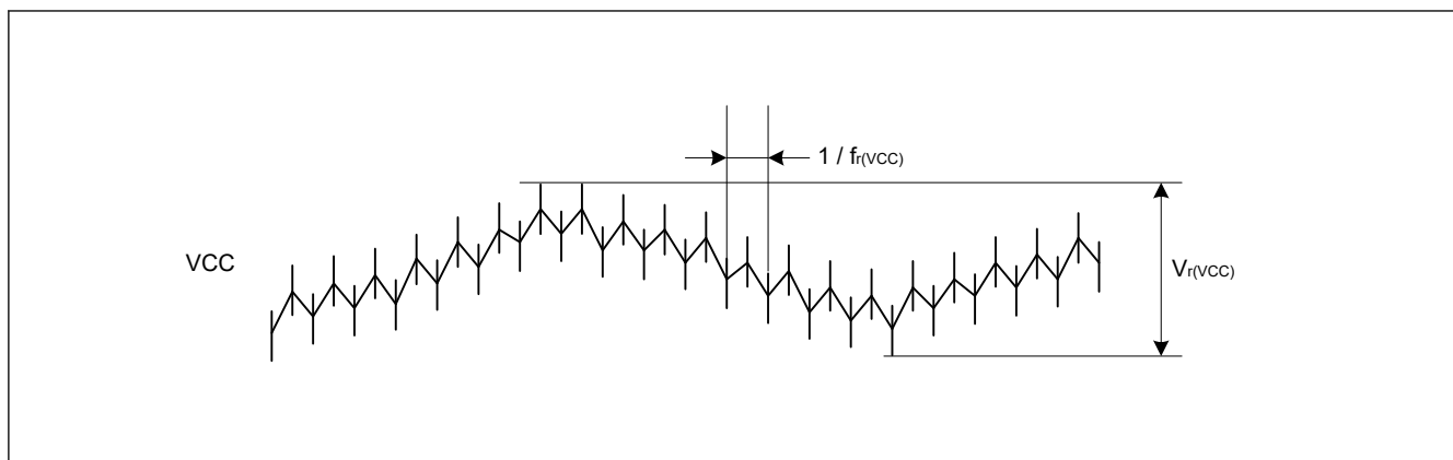
Figure 2.5 Ripple waveform
