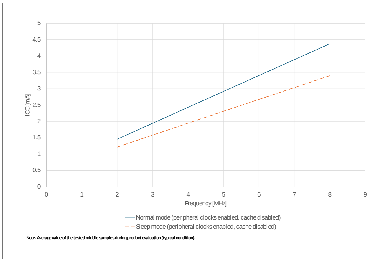
Figure 2.4 Frequency dependency in Middle-speed mode (reference data)
