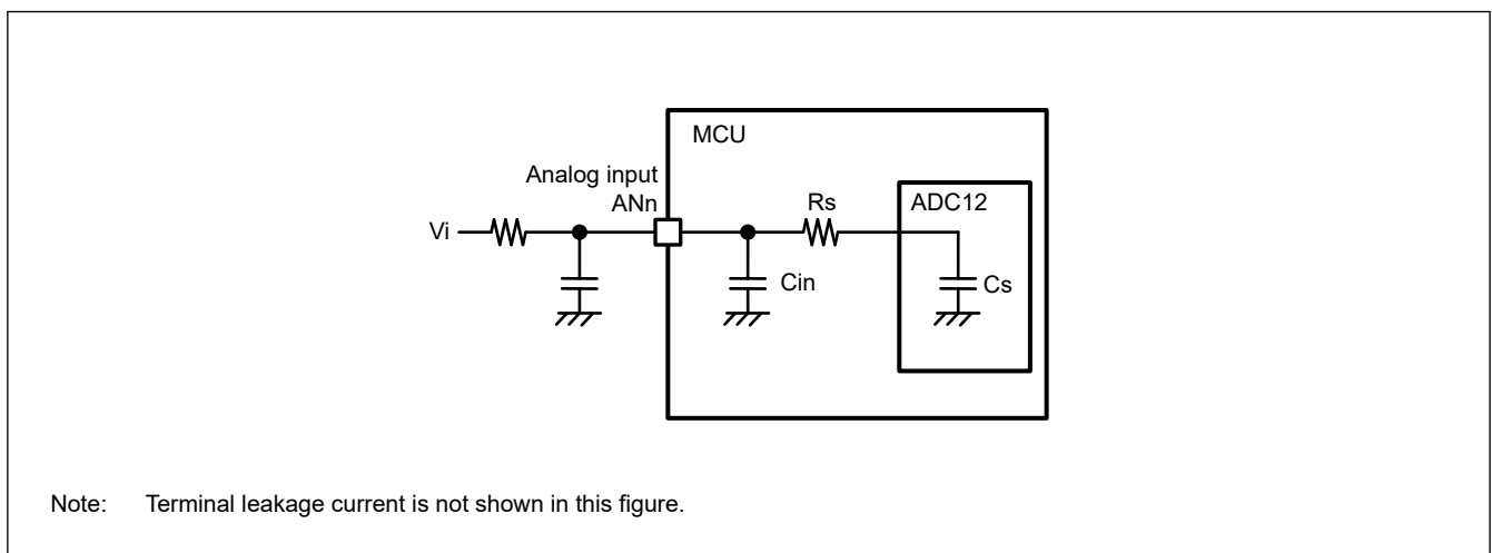
Figure 2.44 Equivalent circuit for analog input
