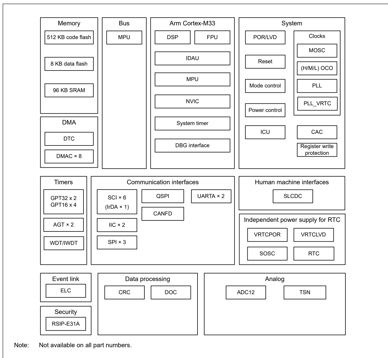
Figure 1.1 Block diagram
