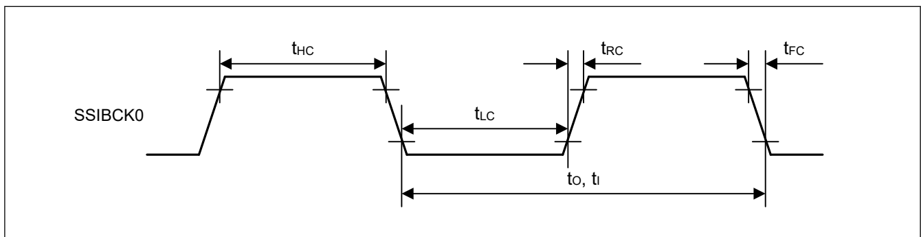
Figure 2.45 SSIE clock input/output timing
