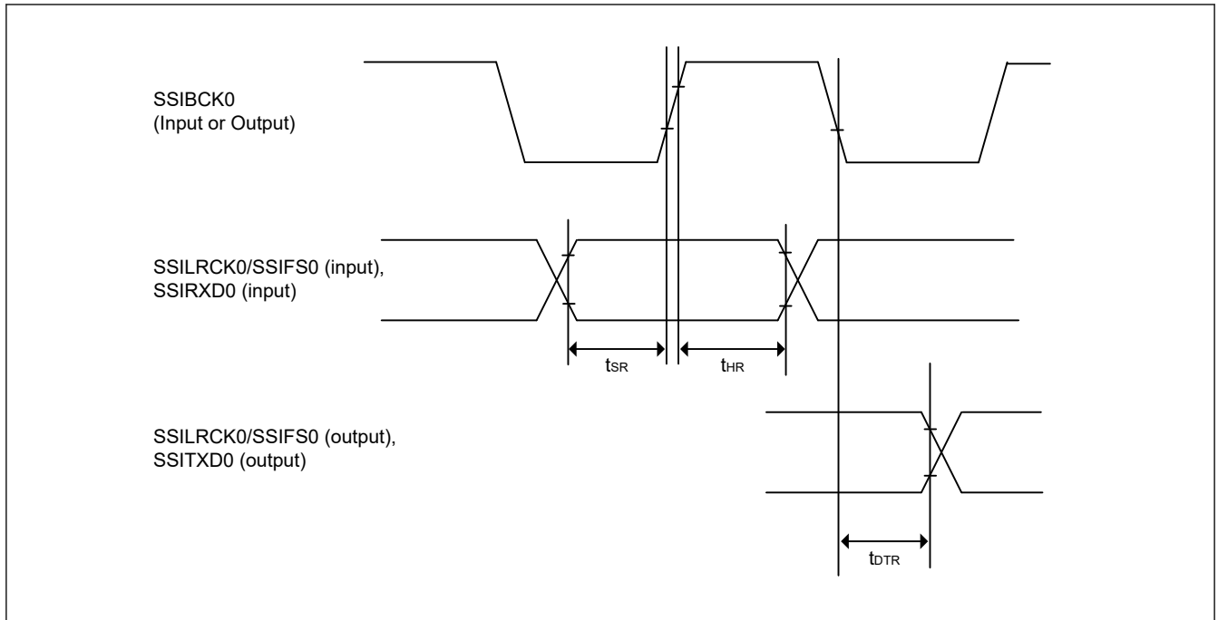
Figure 2.47 SSIE data transmit and receive timing when SSICR.BCKP = 0
