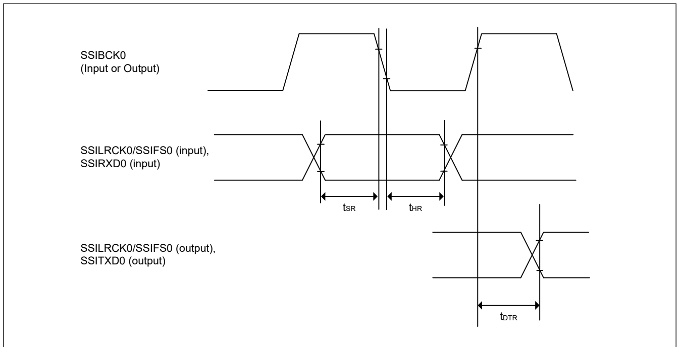
Figure 2.48 SSIE data transmit and receive timing when SSICR.BCKP = 1
