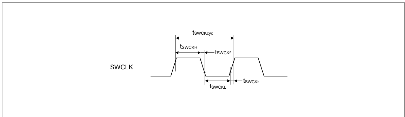
Figure 2.62 SWD SWCLK timing
