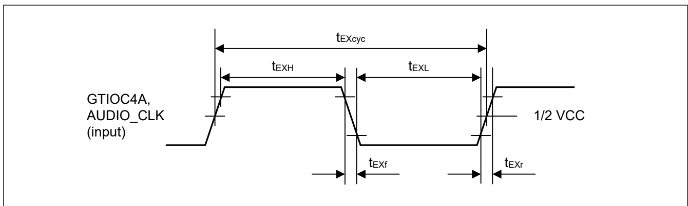
Figure 2.46 Clock input timing
