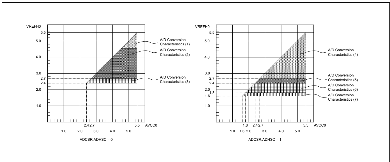
Figure 2.53 AVCC0 to VREFH0 voltage range
