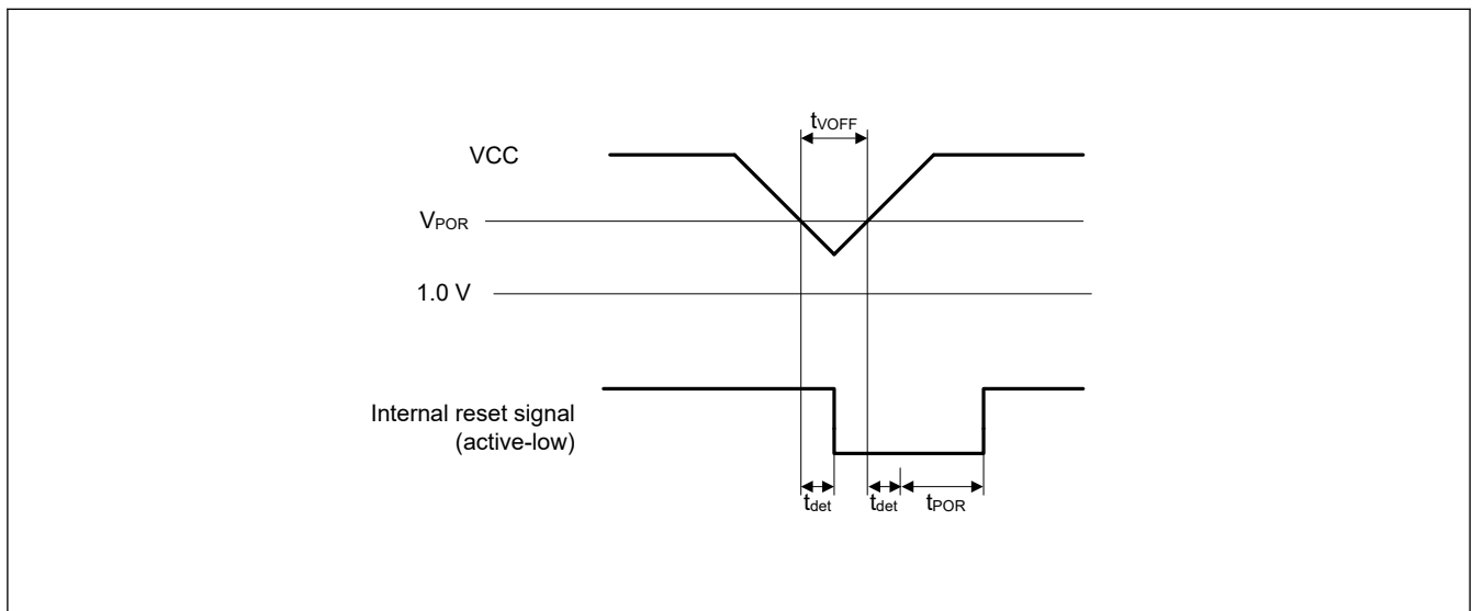
Figure 2.57 Voltage detection reset timing
