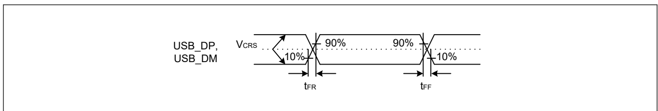
Figure 2.51 USB_DP and USB_DM output timing in full-speed mode
