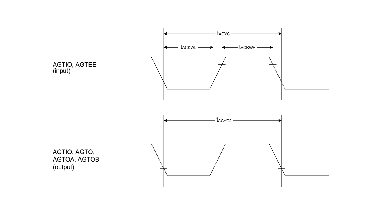
Figure 2.17 AGTW I/O timing
