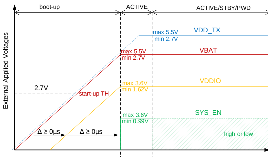
Figure 10. Supply Ramp-Up Sequence
