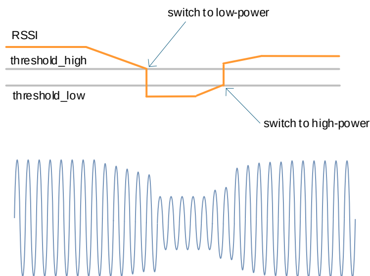
Figure 5. DDPC Concept
