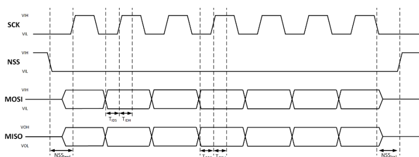
Figure 12. SPI Mode
