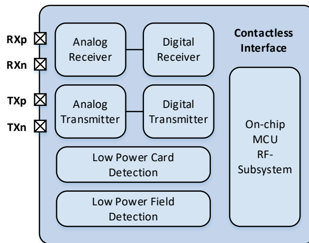
Figure 6: Contactless Interface
