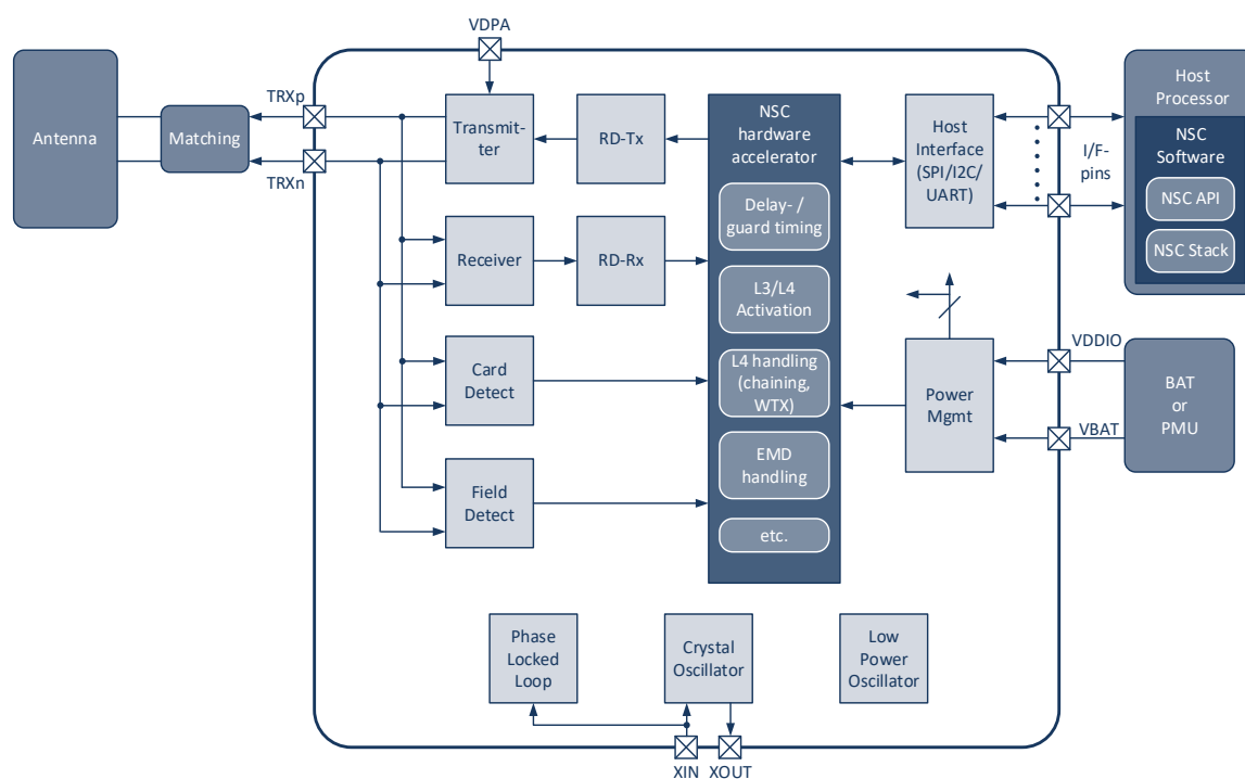
Figure 1: Block Diagram
