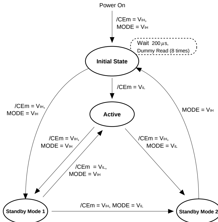
Figure 6-1. Standby Mode State Machine
