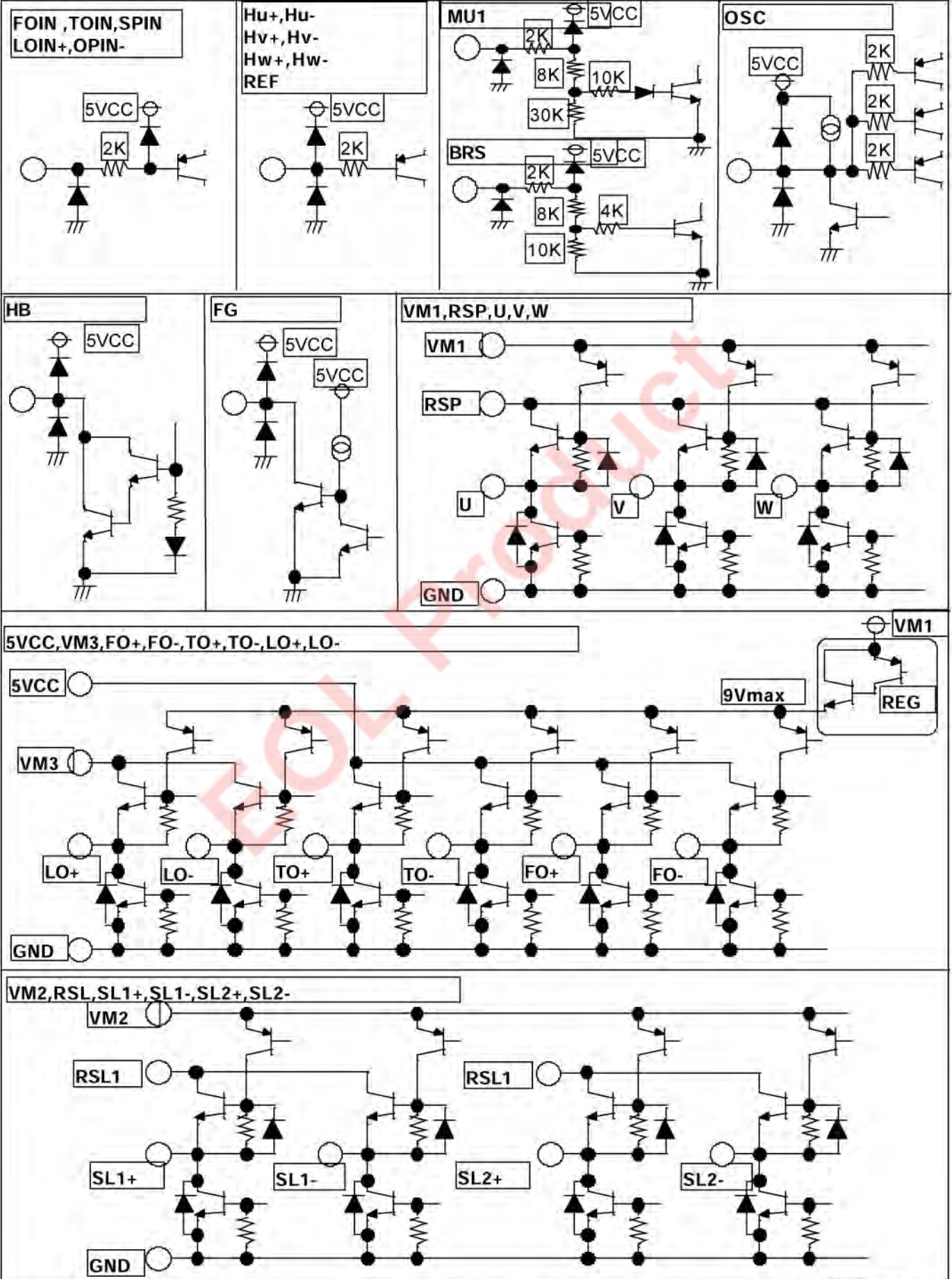
I/O circuit
