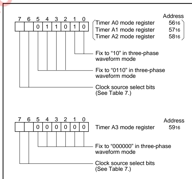
Fig. 42 Bit configuration of timer A0, A1, A2, mode register and timer A3 mode register in three-phase waveform mode
