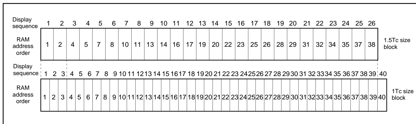
Fig. 64. RAM data for 3nth character
