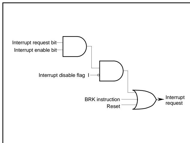
Fig. 6. Interrupt control
