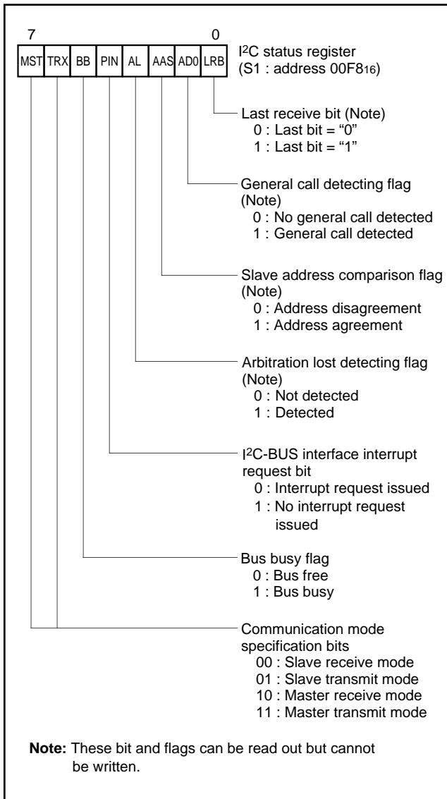
Fig. 41. Structure of I²C status register
