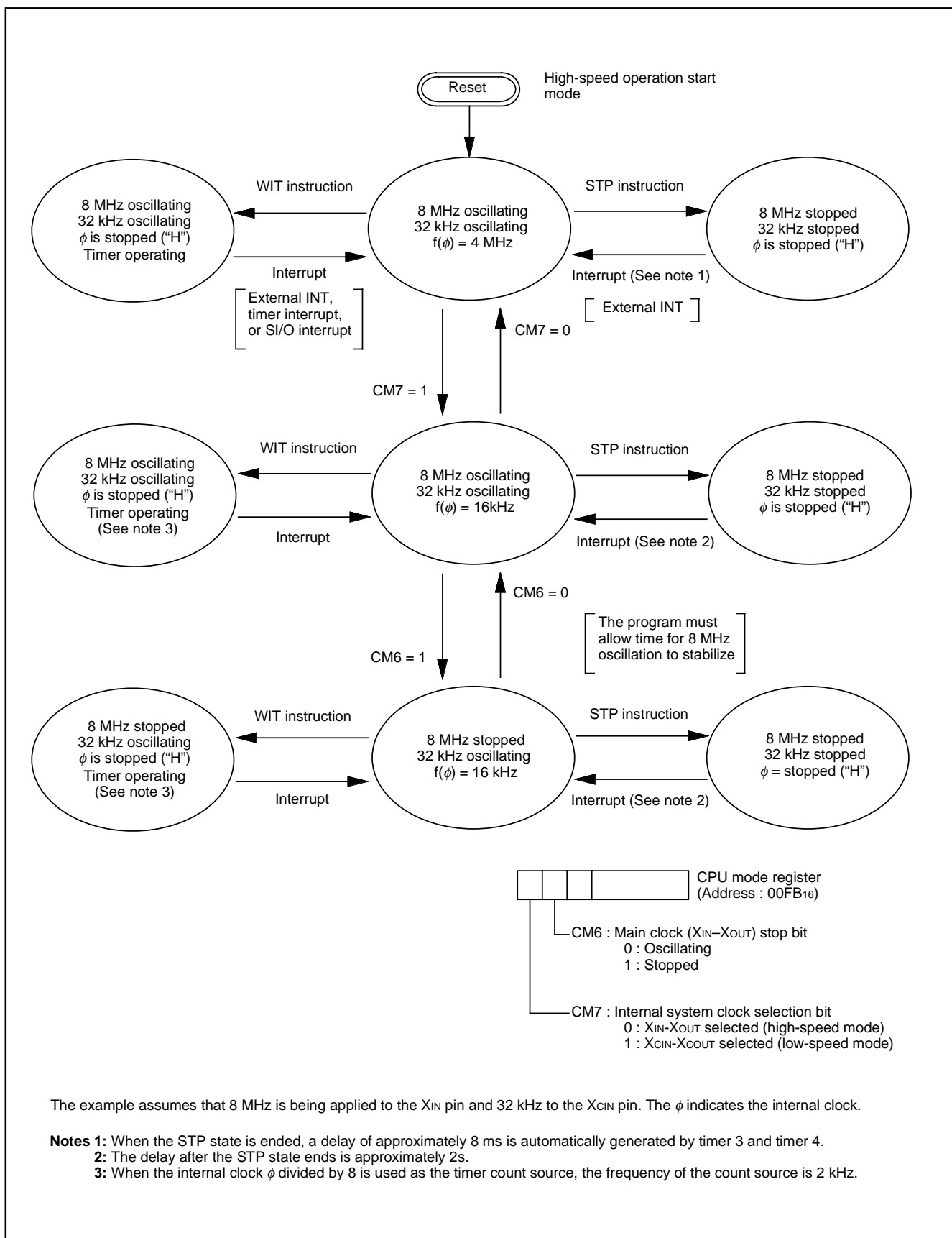
Fig.8.14.5 State Transitions of System Clock
