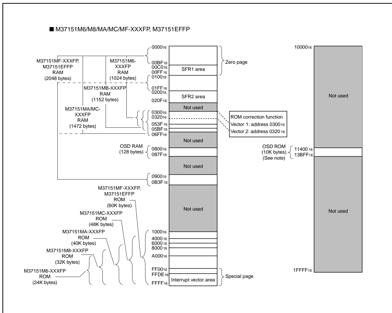
Fig. 8.2.1 Memory Map (M37151M6/M8/MA/MC/MF-XXXFP, M37151EFPF)
