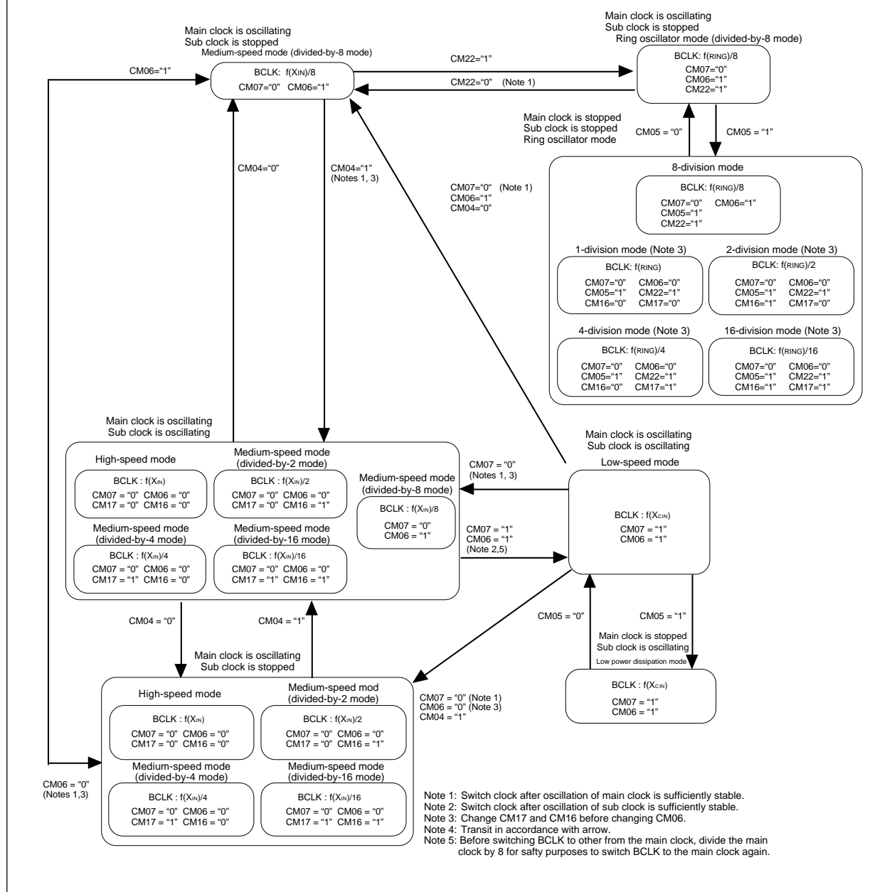
Figure 1.9.2. Clock transition (2)
