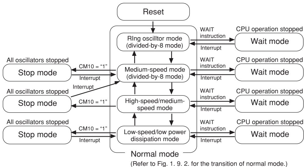
Figure 1.9.1. Clock transition (1)
