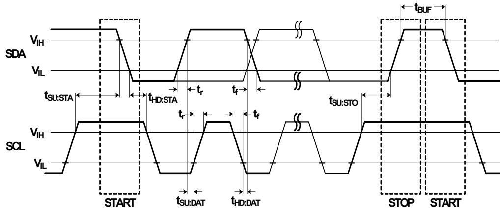
FIGURE 16. I 2 C TIMING DEFINITION
