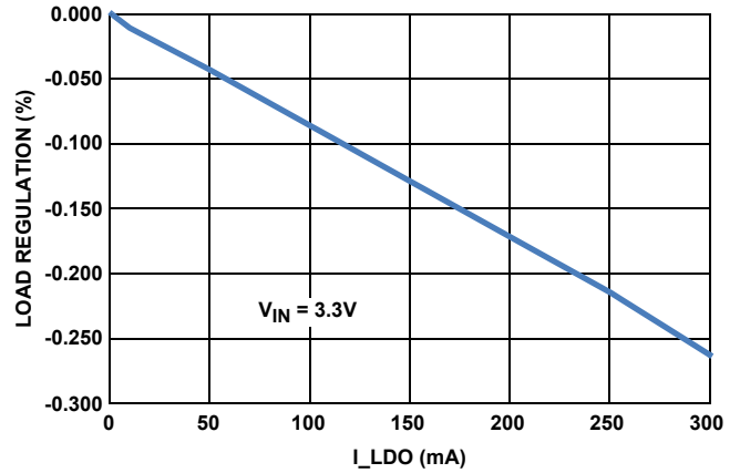
FIGURE 10. L_{D0} LOAD REGULATION
