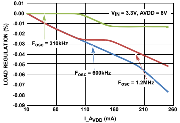
FIGURE 2. AVDD LOAD REGULATION
