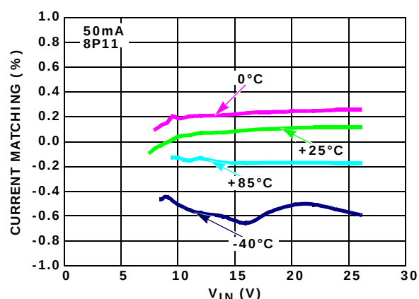
FIGURE 8. CURRENT MATCHING vs V_{IN} vs TEMPERATURE
