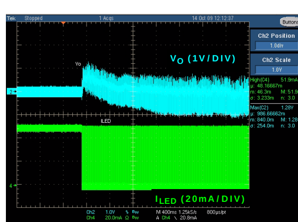
FIGURE 20. LOAD REGULATION WITH I_{LED} CHANGES FROM 100 % TO 0.4 % PWM DIMMING
