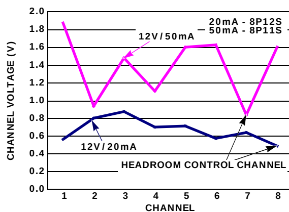
FIGURE 10. TYPICAL CHANNEL VOLTAGE EXAMPLE
