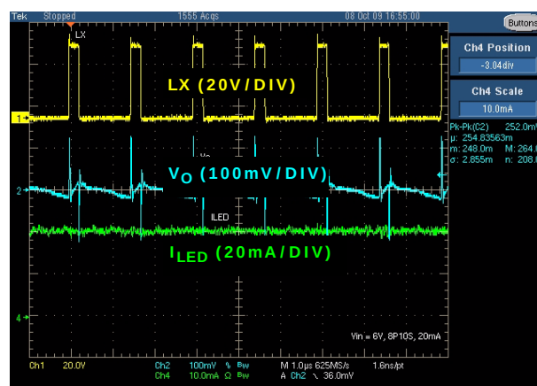
FIGURE 14. V_{OUT} RIPPLE VOLTAGE
