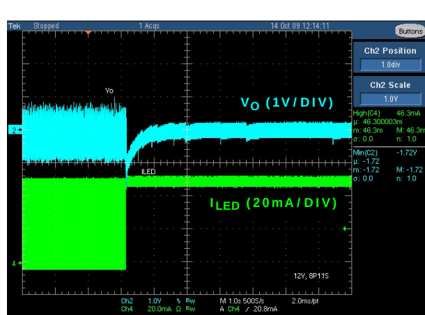
FIGURE 19. LOAD REGULATION WITH I_{LED} CHANGES FROM 0.4 % TO 100 % PWM DIMMING
