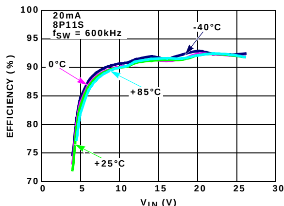
FIGURE 4. EFFICIENCY vs V_{IN} vs TEMPERATURE AT 20mA
