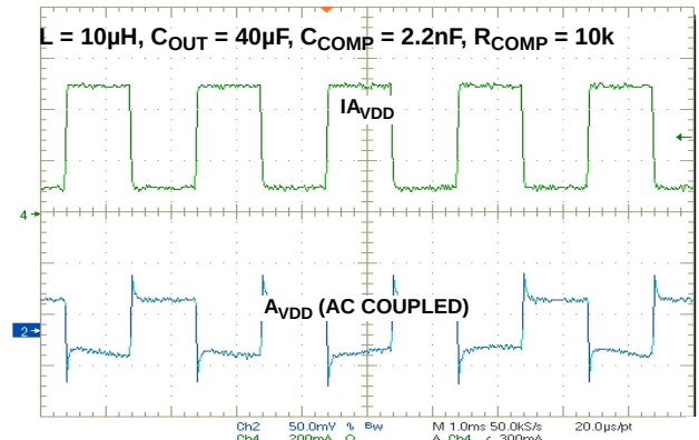
FIGURE 4. BOOST CONVERTER TRANSIENT RESPONSE
